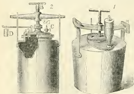
Papin's Digester.
