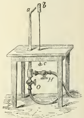
Drummond Light Apparatus.
