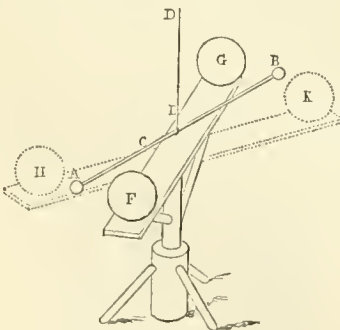
Baily's Apparatus.
