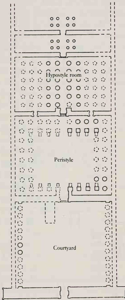
3. The Ramesseum at Thebes: plan, according to Jollois and Devilliers.
