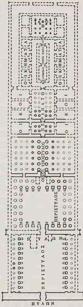
1. The Ramesseum at Thebes: reconstruction by Jollois and Devilliers, based on Diodorus.
