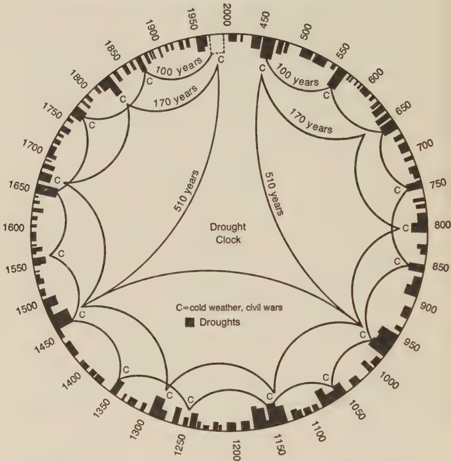
Figure 10 DR. RAYMOND WHEELER'S "DROUGHT CLOCK"
