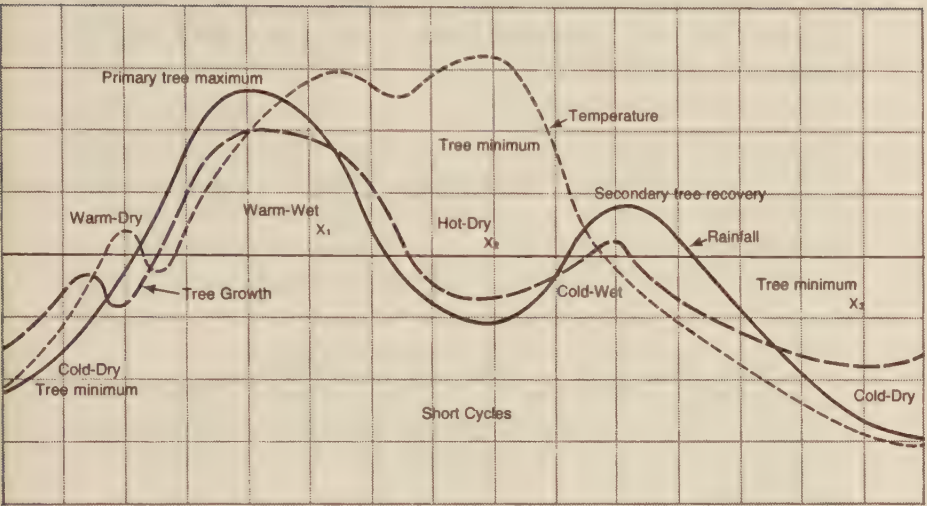
Figure 6 TREE GROWTH IN RELATION TO THE CLIMATIC CYCLE (SCHEMATIC)
