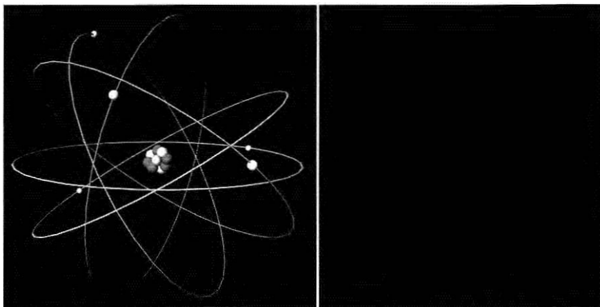
Newtonian Atom
