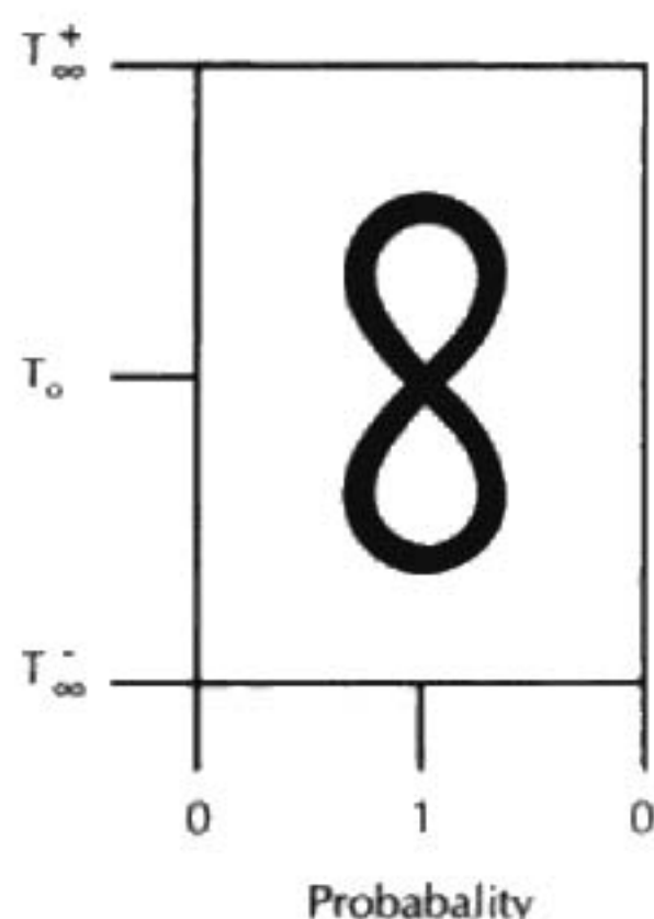
Figure 3. Significant probabilities in "shadow" time.
