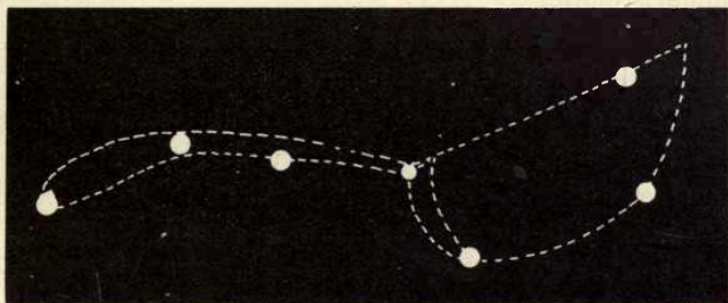
STARS OF THE PLOUGH, AS THE WINNOWING FAN.
