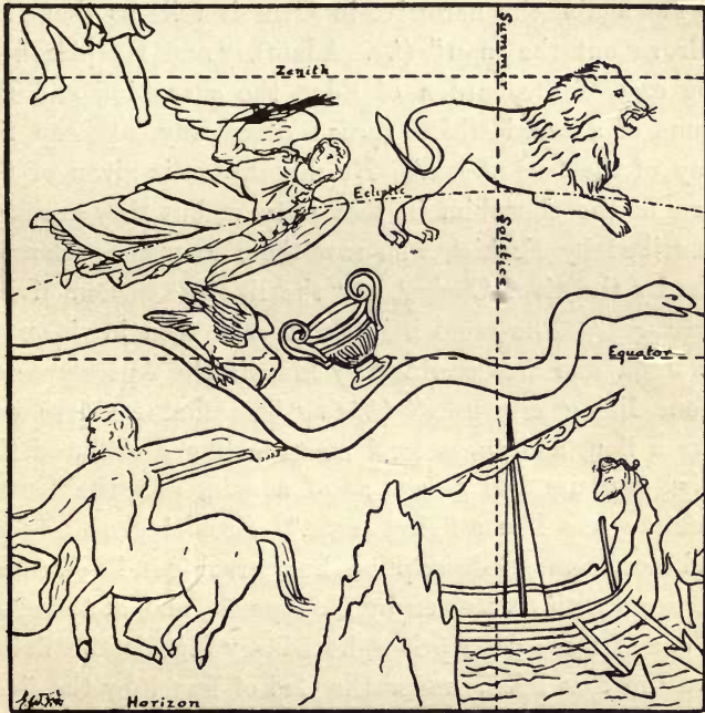
THE MIDNIGHT CONSTELLATIONS OF WINTER, B.C. 2700.
