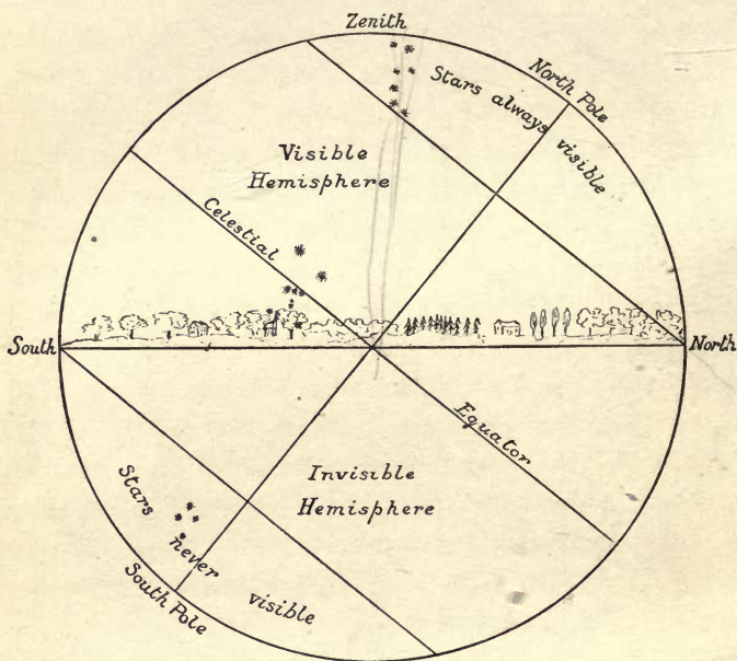
THE CELESTIAL SPHERE.
