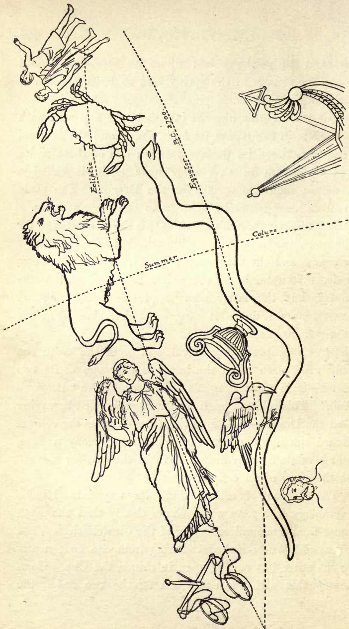
HYDRA AND THE NEIGHBOURING CONSTELLATIONS.
