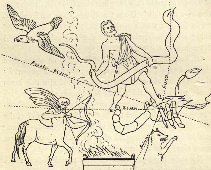
OPHIUCHUS AND THE NEIGHBOURING CONSTELLATIONS.
