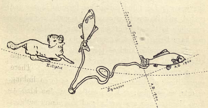
POSITION OF SPRING EQUINOX, A.D. 1900.
