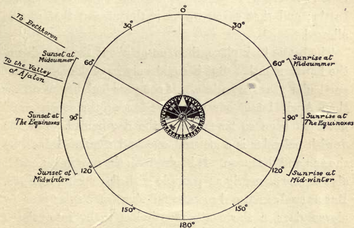
BEARINGS OF THE RISING AND SETTING POINTS OF THE SUN FROM GIBEON.
