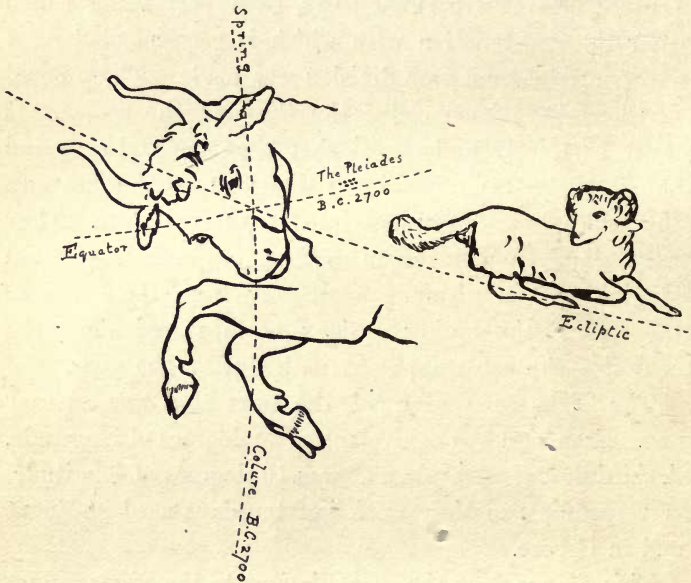
POSITION OF SPRING EQUINOX, B.C. 2700.
