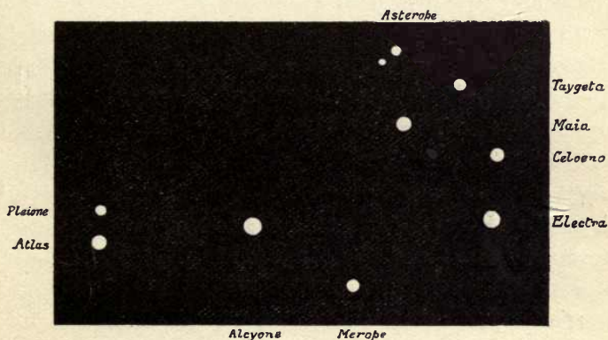
STARS OF THE PLEIADES.
