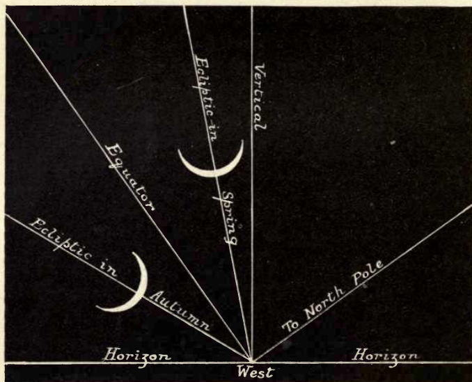
POSITION OF THE NEW MOON AT THE EQUINOXES.
