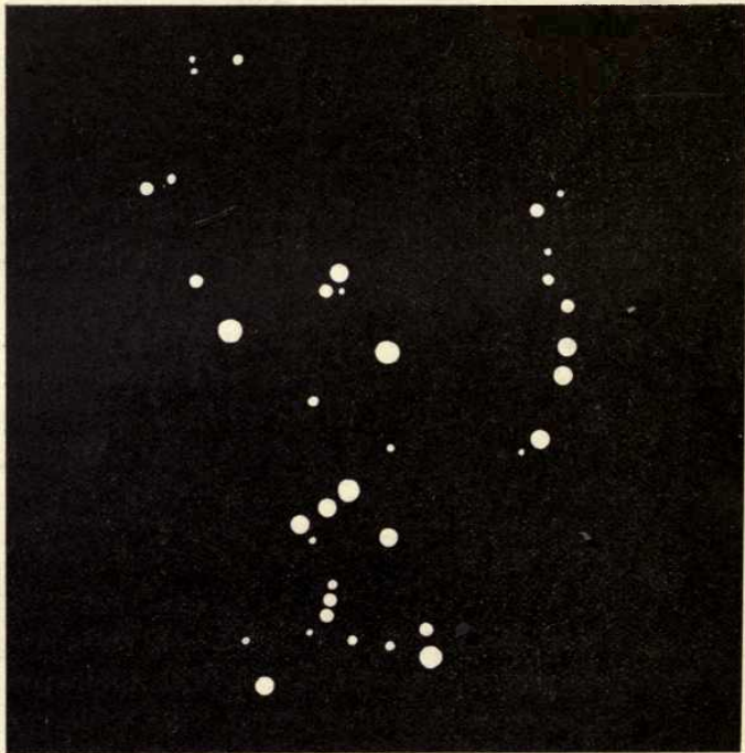
THE STARS OF ORION.
