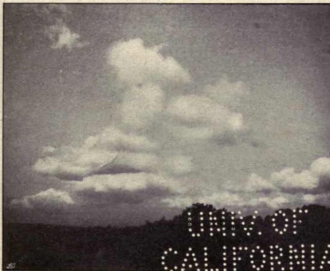
CUMULI FROM TUNBRIDGE WELLS, 1906, MAY 20.
