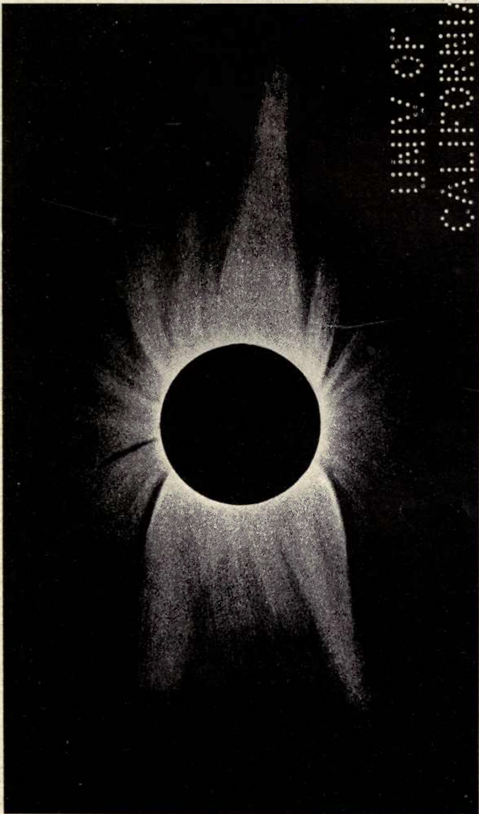
CORONA OF MINIMUM TYPE. Drawing made by W. H. Wesley, from photographs of the 1900 Eclipse.
