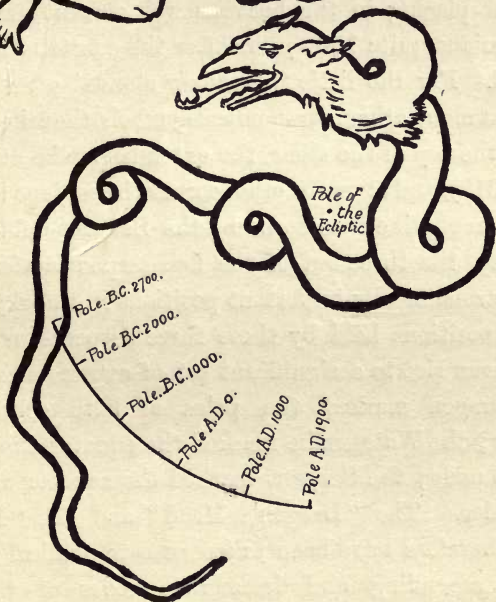
HERCULES AND DRACO.
