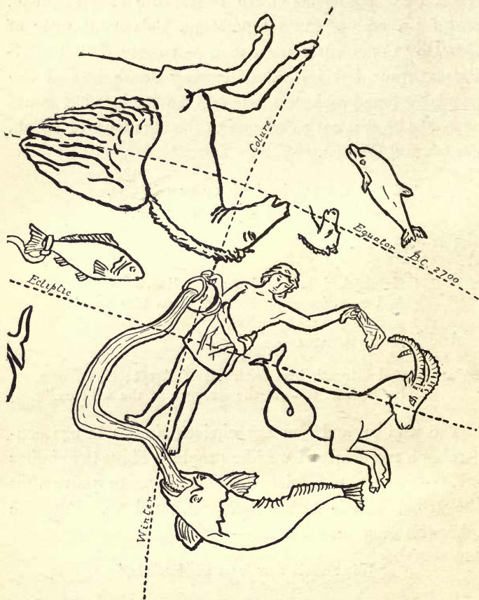
AQUARIUS AND THE NEIGHBOURING CONSTELLATIONS.
