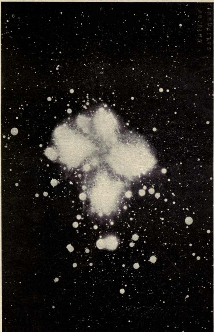
South NEBULOSITIES OF THE PLEIADES.
