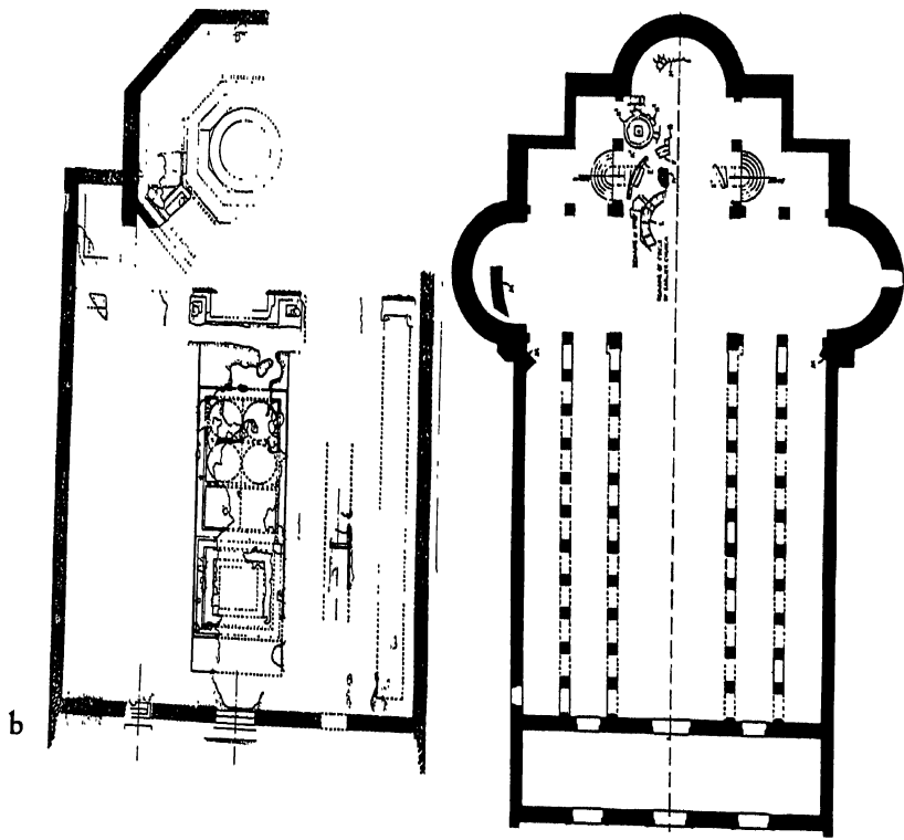
a. Plan of Constantinian church of Eleona, Mount of Olives.—b. Plan of Constantine's church at Bethlehem.—c. Plan of Justinian's reconstruction of same.
