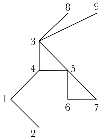
Figure 5.20. Tree of Aristotle’s proof.
