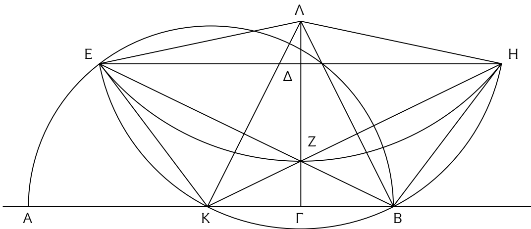
Figure 1.14. Hippocrates’ Third Quadrature.
