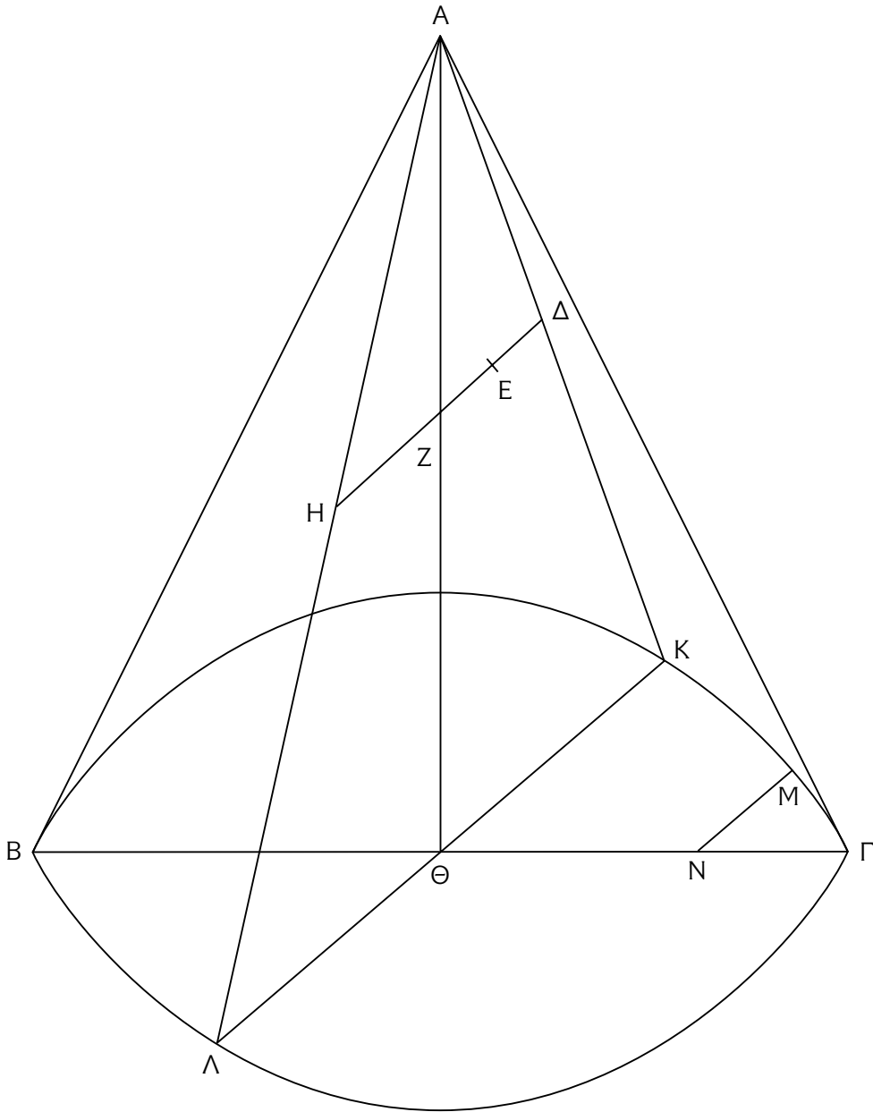
Figure 1.12. Apollonius' Conics I.6 (One of the Cases).
