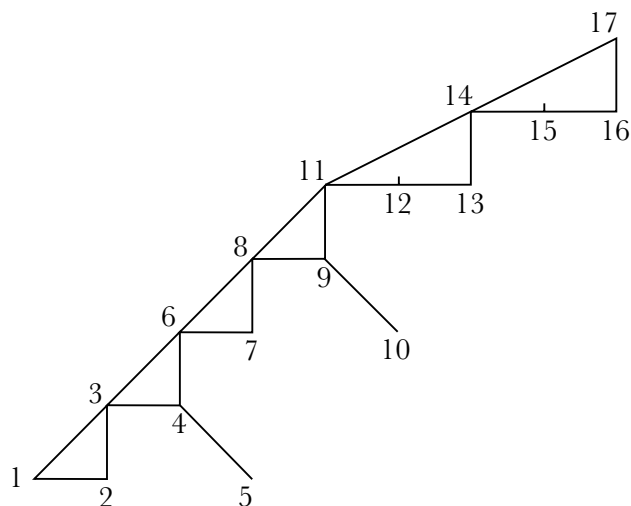
Figure 5.18. The tree of Euclid's Elements II.5.
