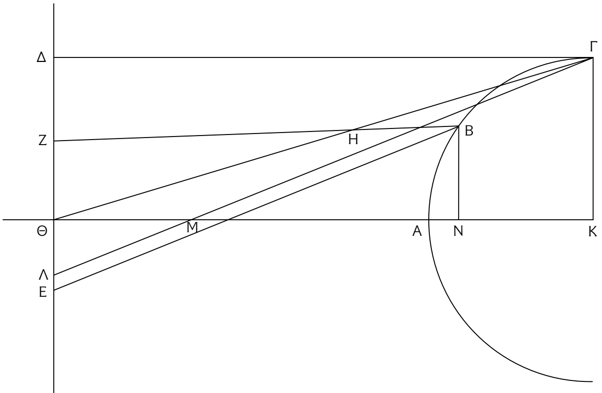
Figure 1.8. Apollonius' Conics I.45 (Hyperbola Case).
