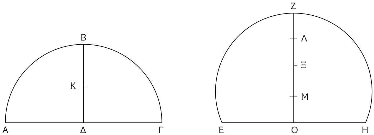
Figure 1.10. Archimedes' PE II.7.
