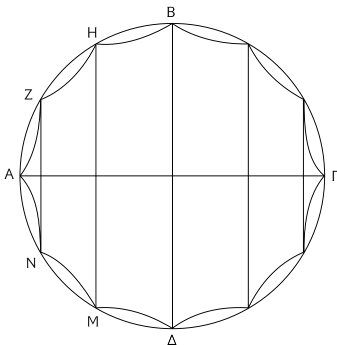
Figure 5.12. Archimedes' SC I.23.
