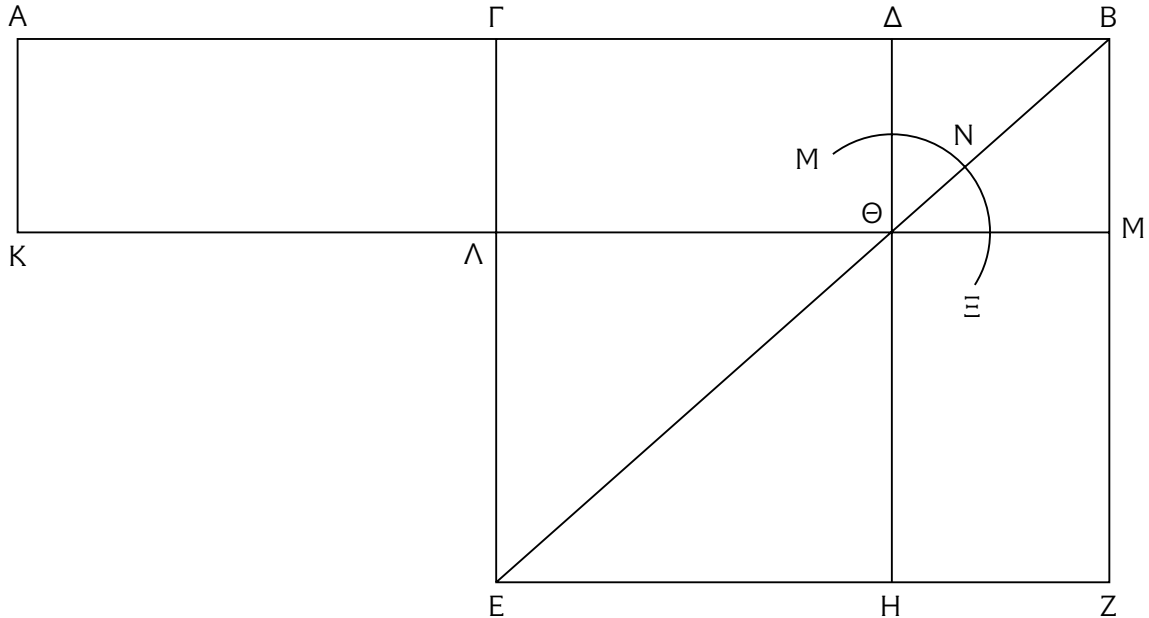
Figure 5.17. Euclid's Elements II.5.
