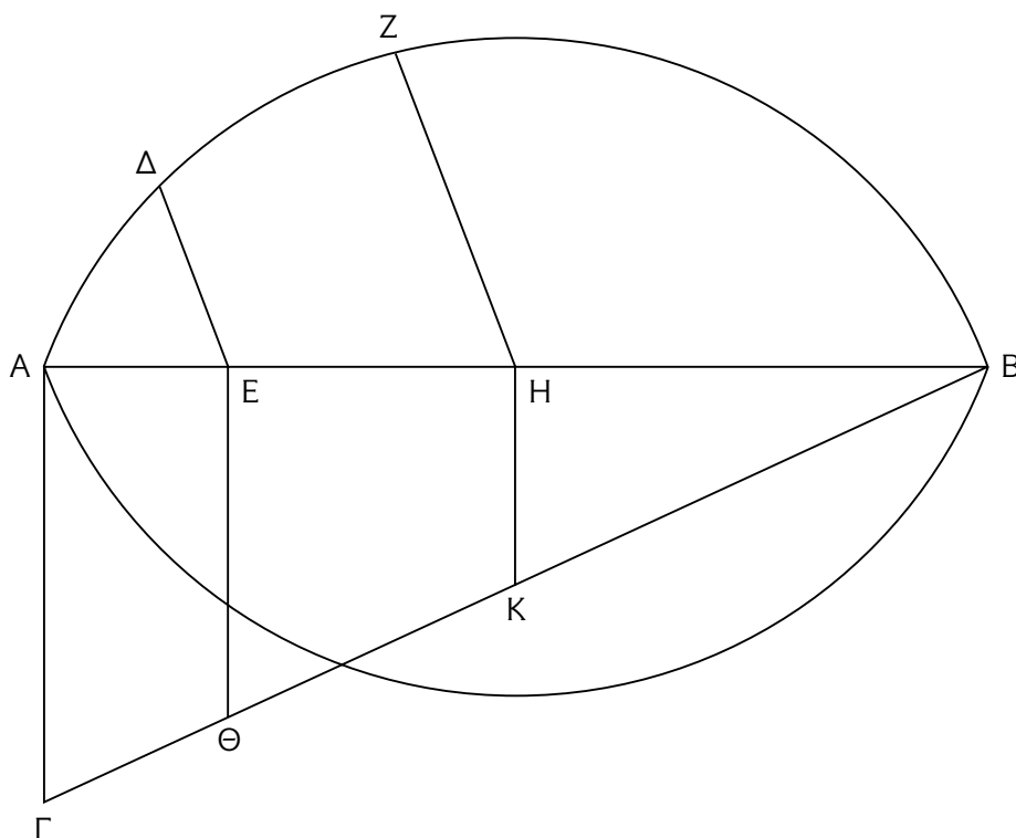
Figure 5.25. Apollonius' Conics 1.21 (Ellipse Case).
