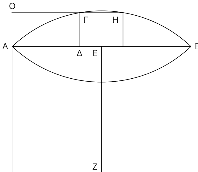
Figure 5.9. Apollonius's Conics 1.41 (Ellipse Case).
