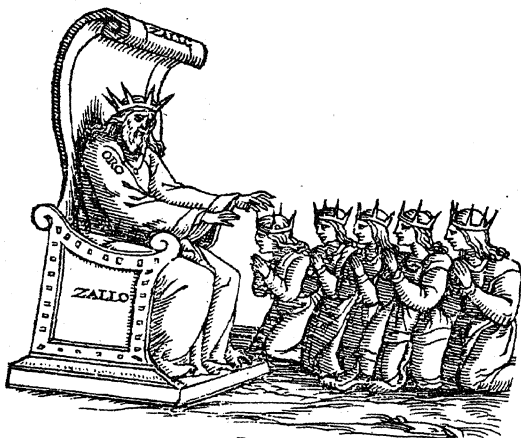
SYMBOLICAL ILLUSTRATION Representing the Transmutation of the Metals.
