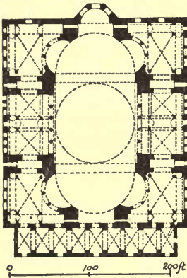
FIG. 76.—PLAN OF HAGIA SOPHIA.
