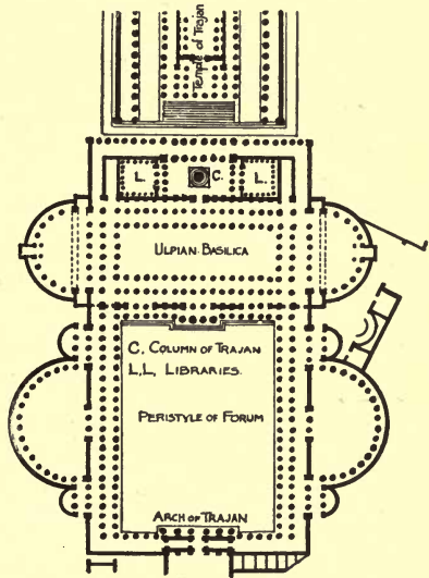
FIG. 57.—FORUM AND BASILICA OF TRAJAN.
