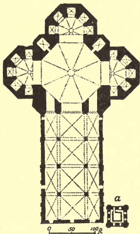
FIG. 152.—DUOMO AT FLORENCE. PLAN.
