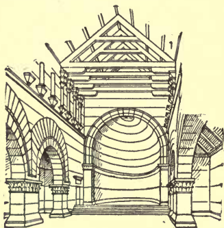
FIG. 69.—CHURCH AT KALB LOUZEH.
