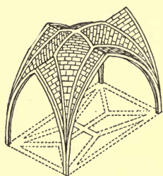
FIG. 111.—RIBBED VAULT, ENGLISH TYPE WITH DIVIDED GROIN-RIBS AND RIDGE-RIBS.
