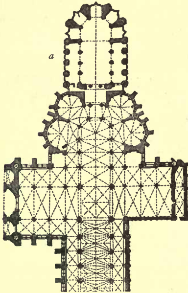
FIG. 142.—EASTERN HALF OF WESTMINSTER ABBEY. PLAN.
