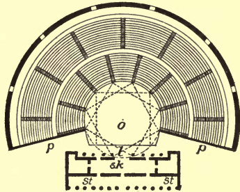
FIG. 40.—PLAN OF GREEK THEATRE. o , Orchestra; l , Logeion; p , Paraskenai; sk , Skene; st, st , Stoa.
