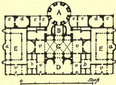
FIG. 60.—THERMÆ OF CARACALLA. PLAN OF CENTRAL BLOCK.
