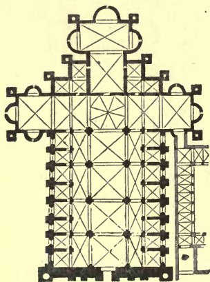
FIG. 158.—PLAN OF CERTOSA AT PAVIA.
