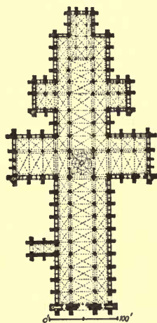
FIG. 133.—PLAN OF SALISBURY CATHEDRAL.
