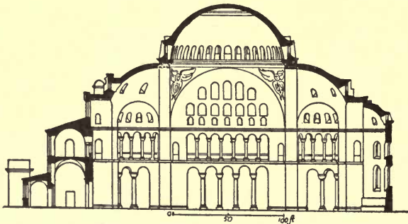
FIG. 77.—SECTION OF HAGIA SOPHIA.
