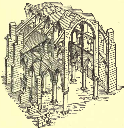
FIG. 108.—CONSTRUCTIVE SYSTEM OF GOTHIC CHURCH. ILLUSTRATING PRINCIPLES OF ISOLATED SUPPORTS AND BUTTRESSING.
