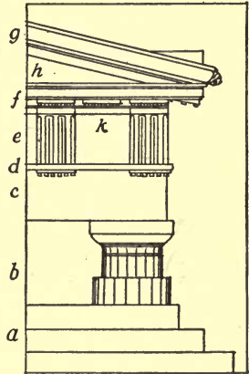
FIG. 26.—GREEK DORIC ORDER.
