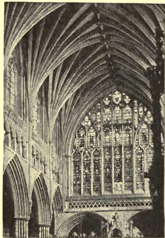
FIG. 134.—RIBBED VAULTING, CHOIR OF EXETER CATHEDRAL.
