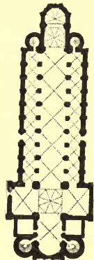
FIG. 102.—PLAN OF MINSTER AT WORMS.
