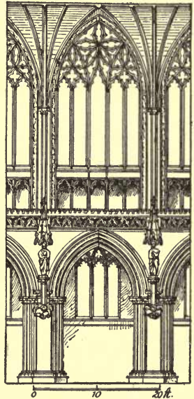
FIG. 140.—ONE BAY OF CHOIR, LICHFIELD CATHEDRAL.
