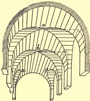
FIG. 112.—PENETRATIONS AND INTERSECTIONS OF VAULTS.
