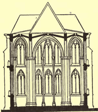
FIG. 145.—SECTION OF ST. ELIZABETH, MARBURG.
