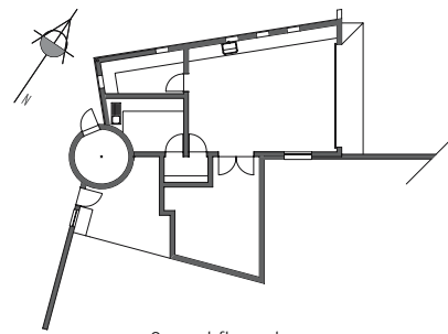
Ground floor plan of entrance tower
