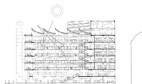
North-south longitudinal section
