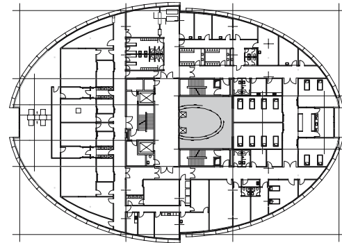
Fifth floor plan (surgery area)
