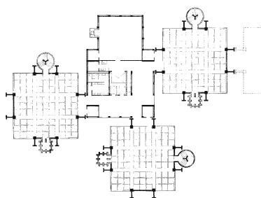
Richards Medical Research Building at the University of Pennsylvania, Philadelphia, USA; architect: Louis I. Kahn, 1957-1961. Connection of two laboratory buildings
