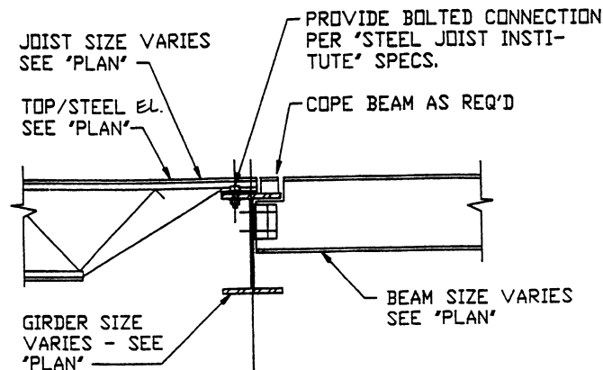
BAR JOIST AND BEAM CONNECTION AT INTERIOR GIRDER
