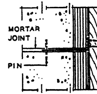
Vertical section
