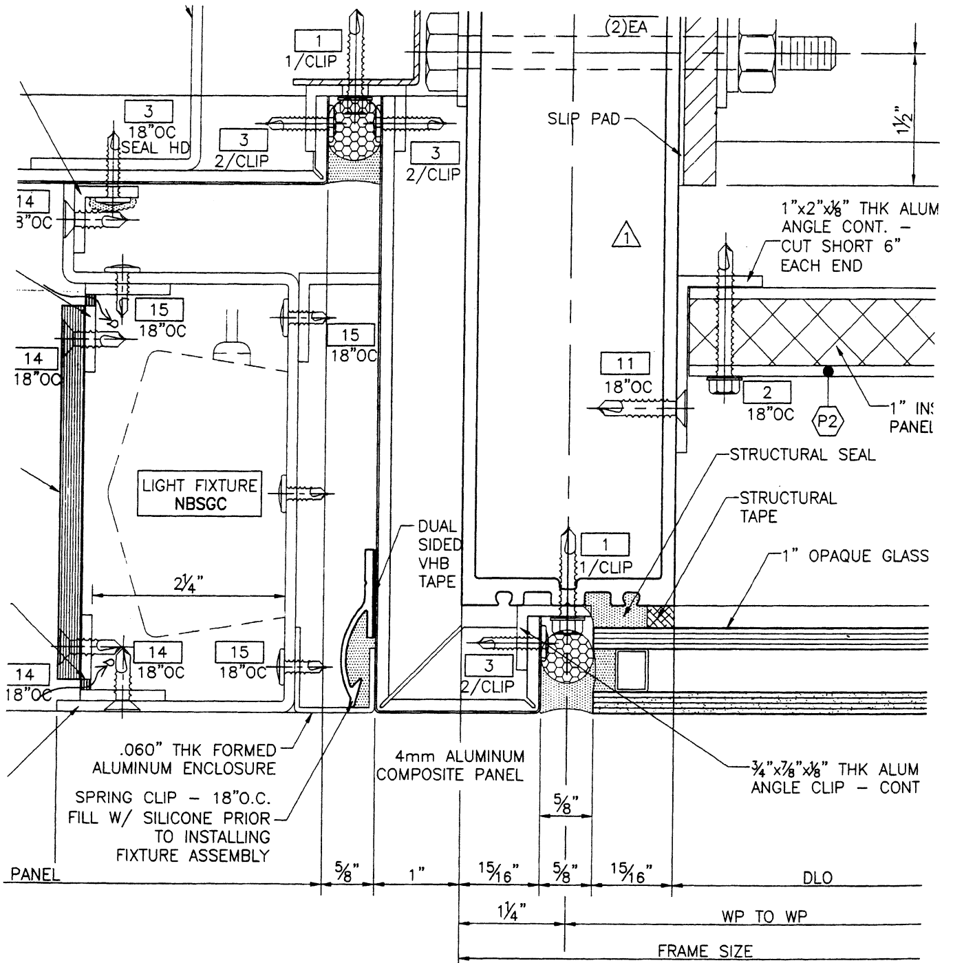
Fig. 12-5 Example of shop drawing for panel wall system. Extreme example that shows each device and part, precisely, so shop personnel can easily assembly the parts. originally drawn full size; reduced here.
