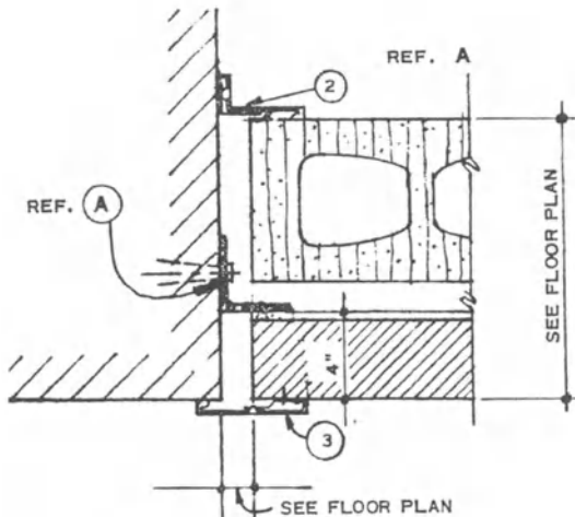
B EXPANSION JOINT CONNECTION AT EXTERIOR WALL
