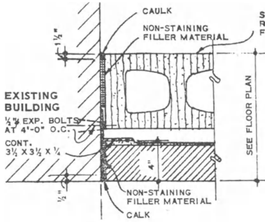
A CONNECTION NEW EXTERIOR WALL TO EXISTING
