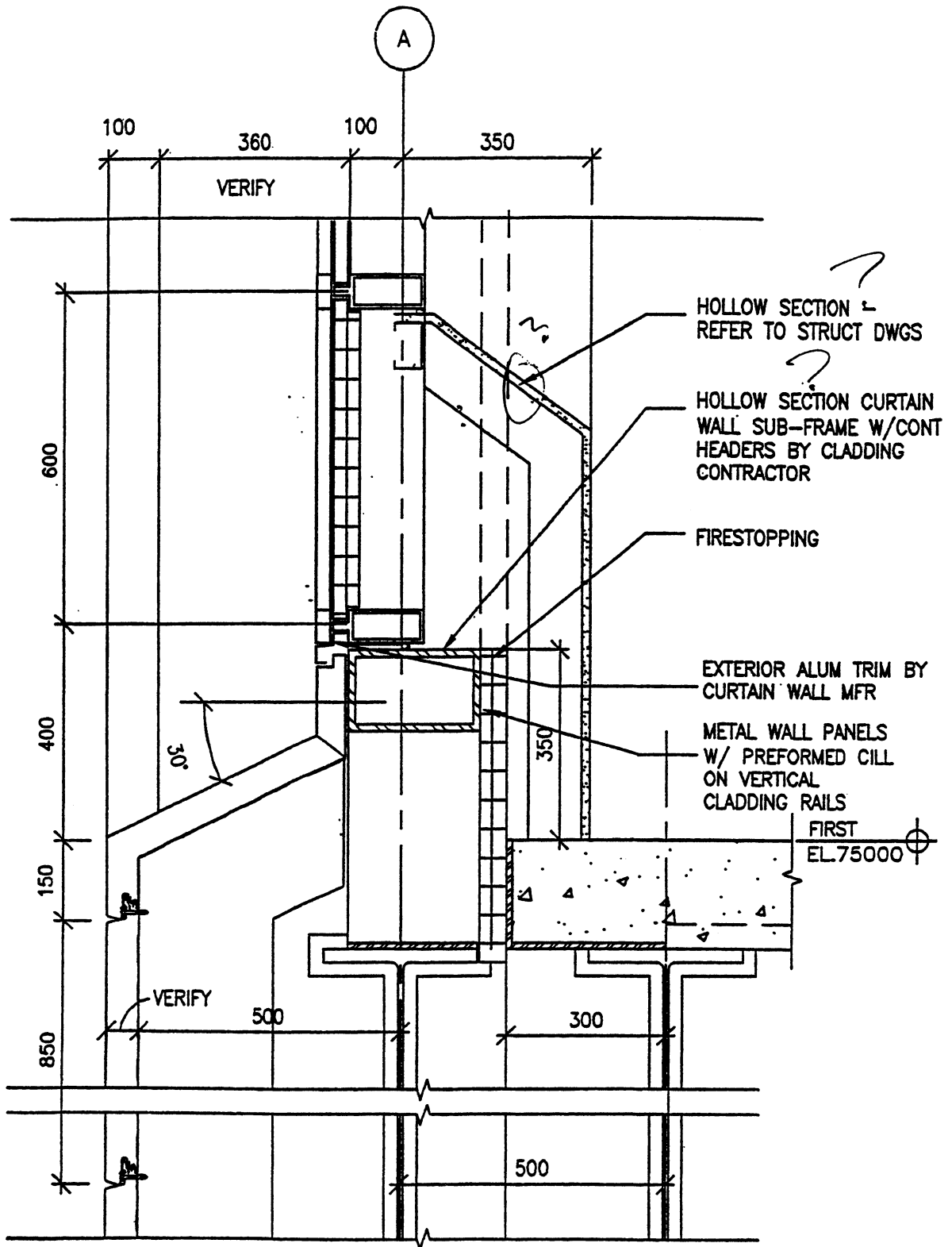
Fig. 10-36 Detail in question due to lack of clarity between notes and graphic drawing
