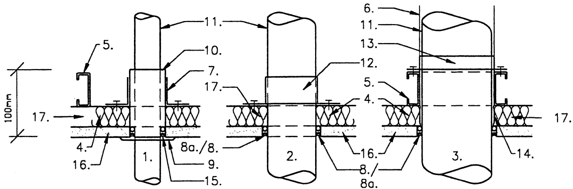
SECTIONS SHOWN AT PENETRATIONS AT RIGHT ANGLES TO CEILING SECTION CHANNELS, PENETRATIONS PARALLEL TO CEILING CHANNELS ARE SIMILAR
