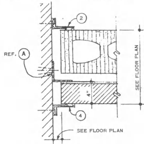
E EXPANSION JOINT CONNECTION AT EXTERIOR WALL
