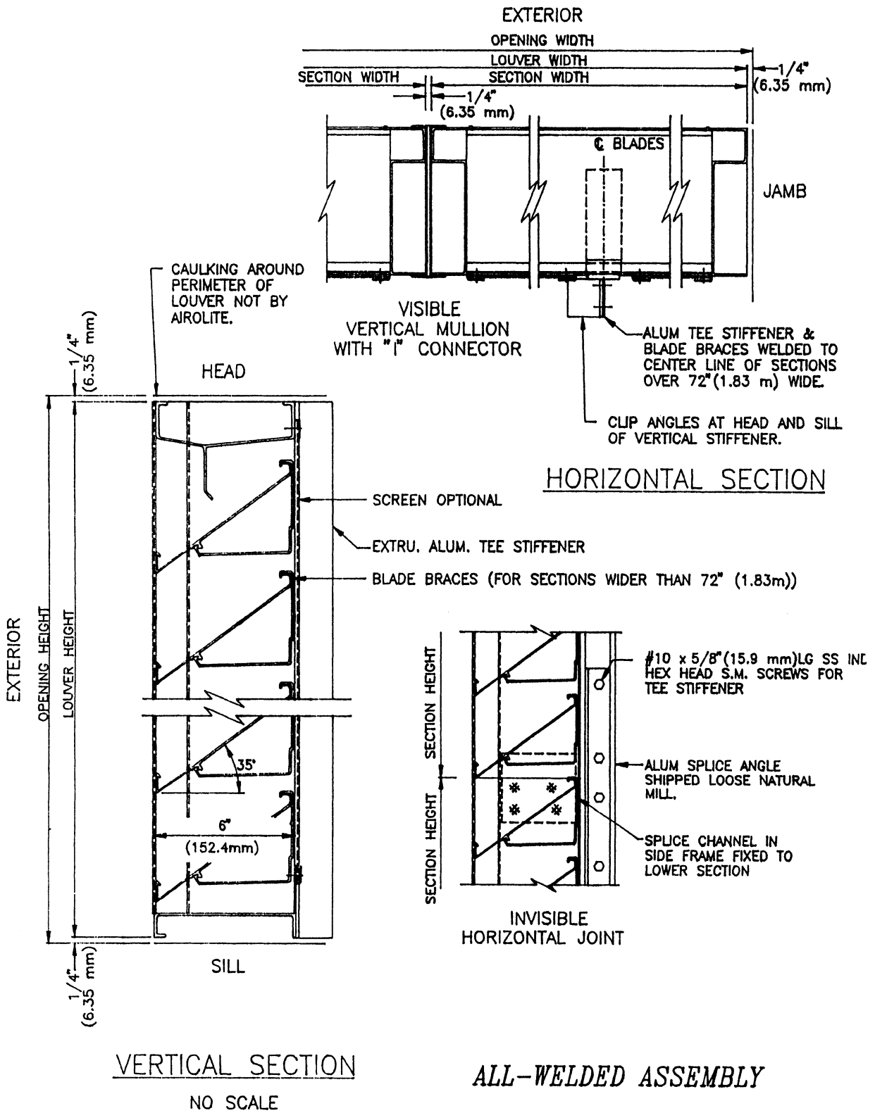
Fig. 12-17 Wall louver details from another manufacturer show various views of the unit
