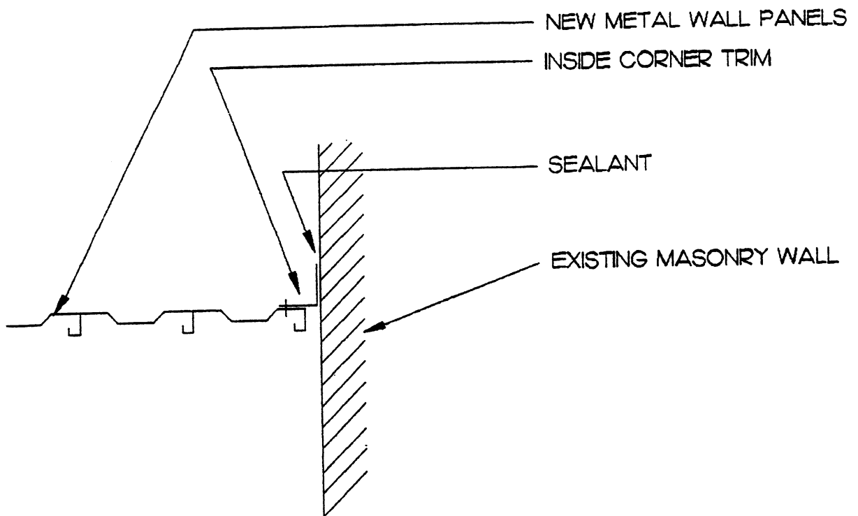
Fig. 10-9 Questionable detail- i.e., is it really necessary. Simply shows the trim between metal wall panels and masonry, and location of sealant.
