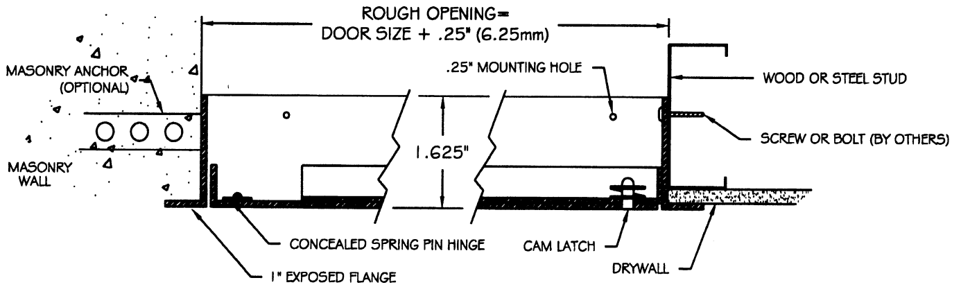
A CUT-THRU SECTION A NOT TO SCALE
