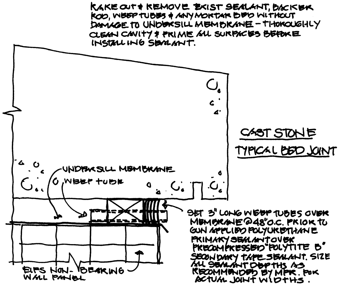
Fig. 11-16 Reviewer's vertical section showing bed joint under sills and added weep tubes
