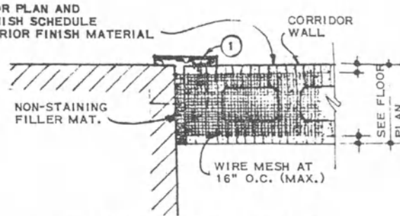
C CONNECTION NEW INTERIOR WALL TO EXISTING AT CORRIDOR
