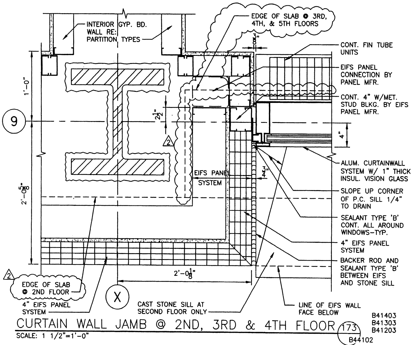
Fig. 11-10 Plan view of the jamb of the sill and fit to adjacent construction
