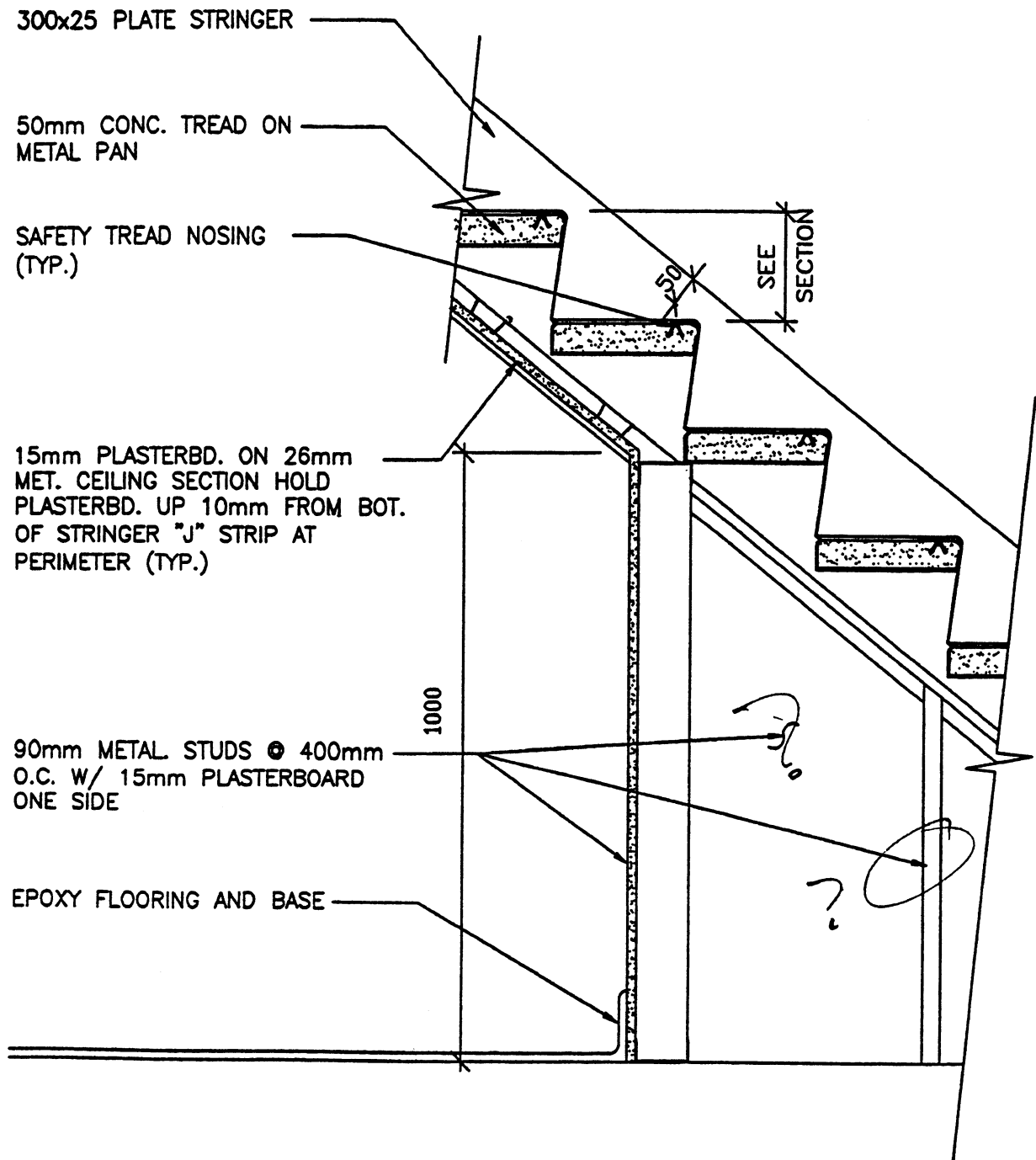
Fig. 10-59 Using multiple leader lines from one note to several areas/materials in differing locations and views is questionable—leads to confusion and unnecessary questions
