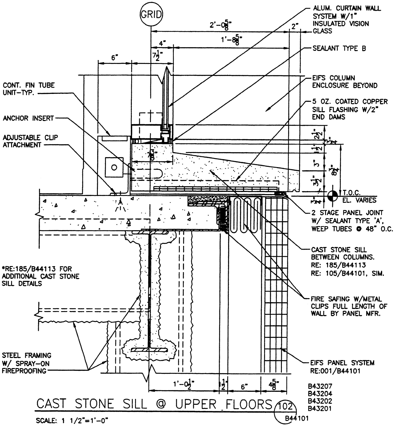
Fig. 11-8 Sill another location- same sill with some varied information
