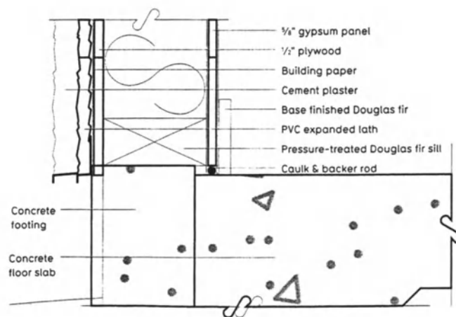
Exterior wall at foundation
