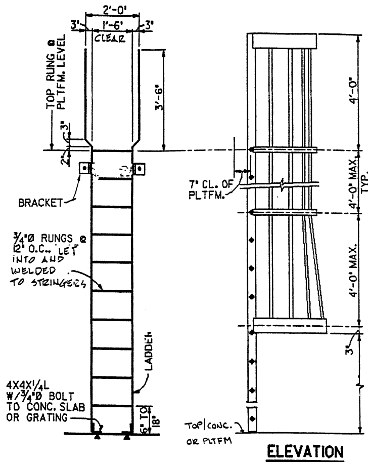
TYPICAL LADDER DETAILS
