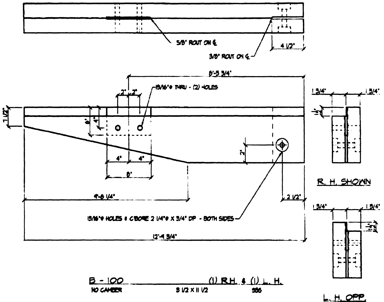
Fig. 12-13 Shop drawing showing the precise fabrication requirements for a large pre-fabricated wood beam.
