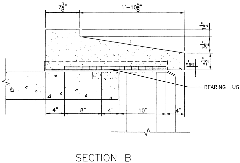
Fig. 11-6 Section B taken as noted on Fig. 11-4
