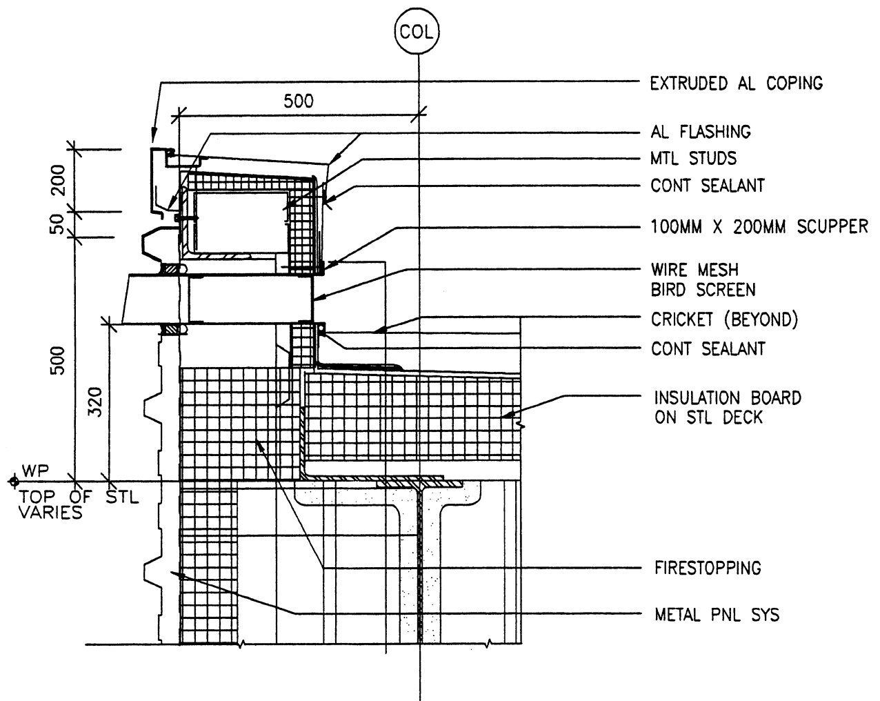
Fig. 10-19 Scupper detail with a lot going on, but somewhat murky because of the strong material symbol. Parts of construction need to be stronger than that symbol for clarity
