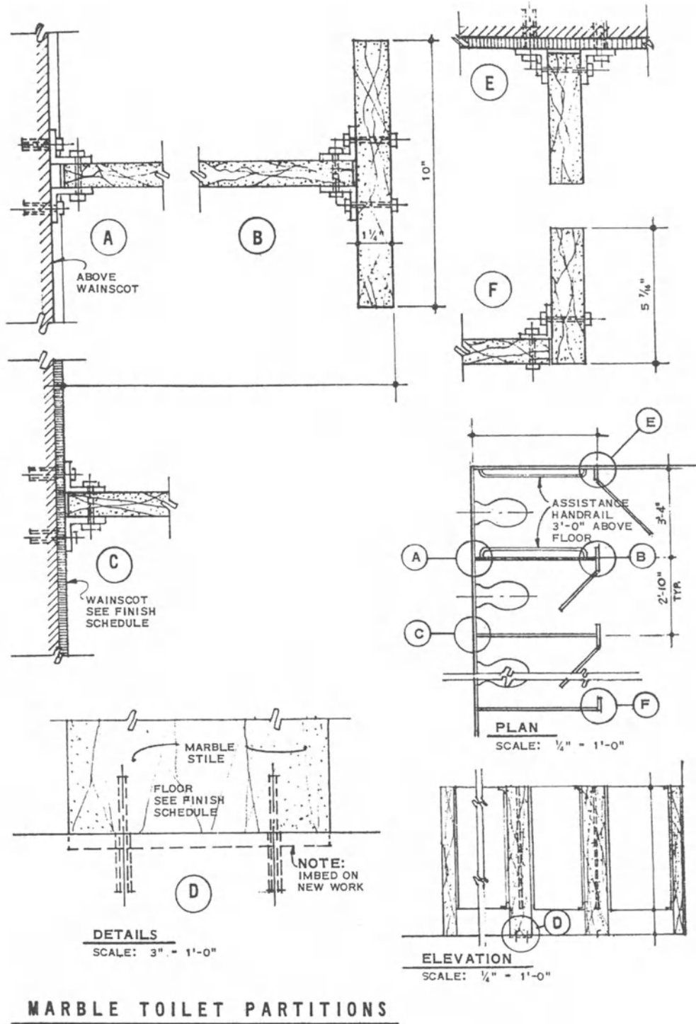
Fig. 12-11 Unusual details since stone or marble toilet compartments are used for high-profile, up-scale installations only. But nonetheless, details are required when the system is used, to ensure consistent high quality.
