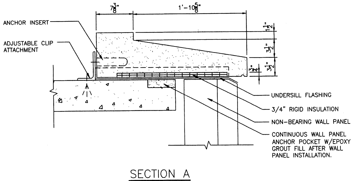
Fig. 11-5 Section A taken as noted on Fig. 11-4
