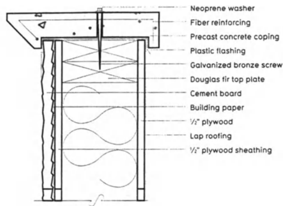
Exterior wall at parapet
