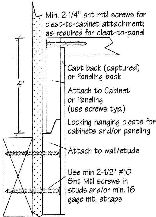
Figure 1700-01 - Cabinet or Panel Hanging
