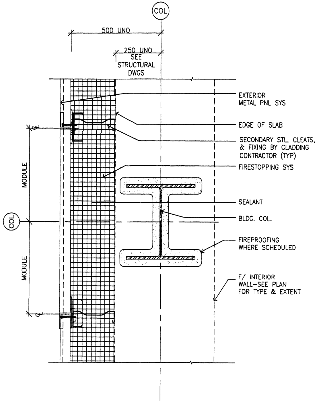
Fig. 10-63 Horizontal detail where major elements [edge of slab, exterior metal pnl sys, column, etc.] are not well-define and are overwhelmed by the least significant information [the insulation material symbol]
