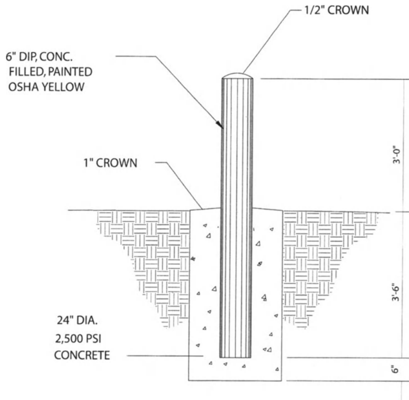
BOLLARD DETAIL
