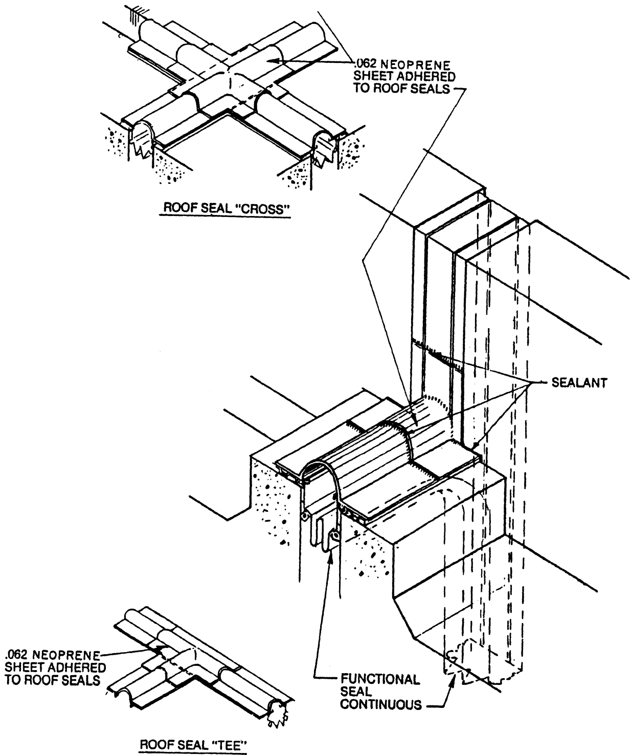
Fig. 12-25 Manufacturer's isometric views of the joint cover details
