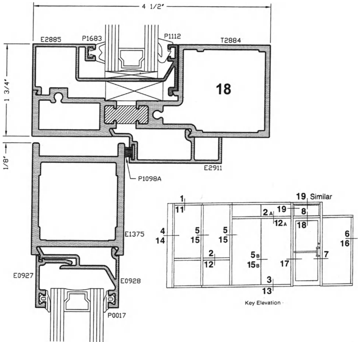
Fig. 10-44 Detail of a manufacturer that shows all of the quirks of the extrusions, but overall a very fine detail— clear and descriptive. This is the head bar between the top of the door and the glass transom light [No. 18 in elevation]. Goes well beyond what the design professional needs to provide
