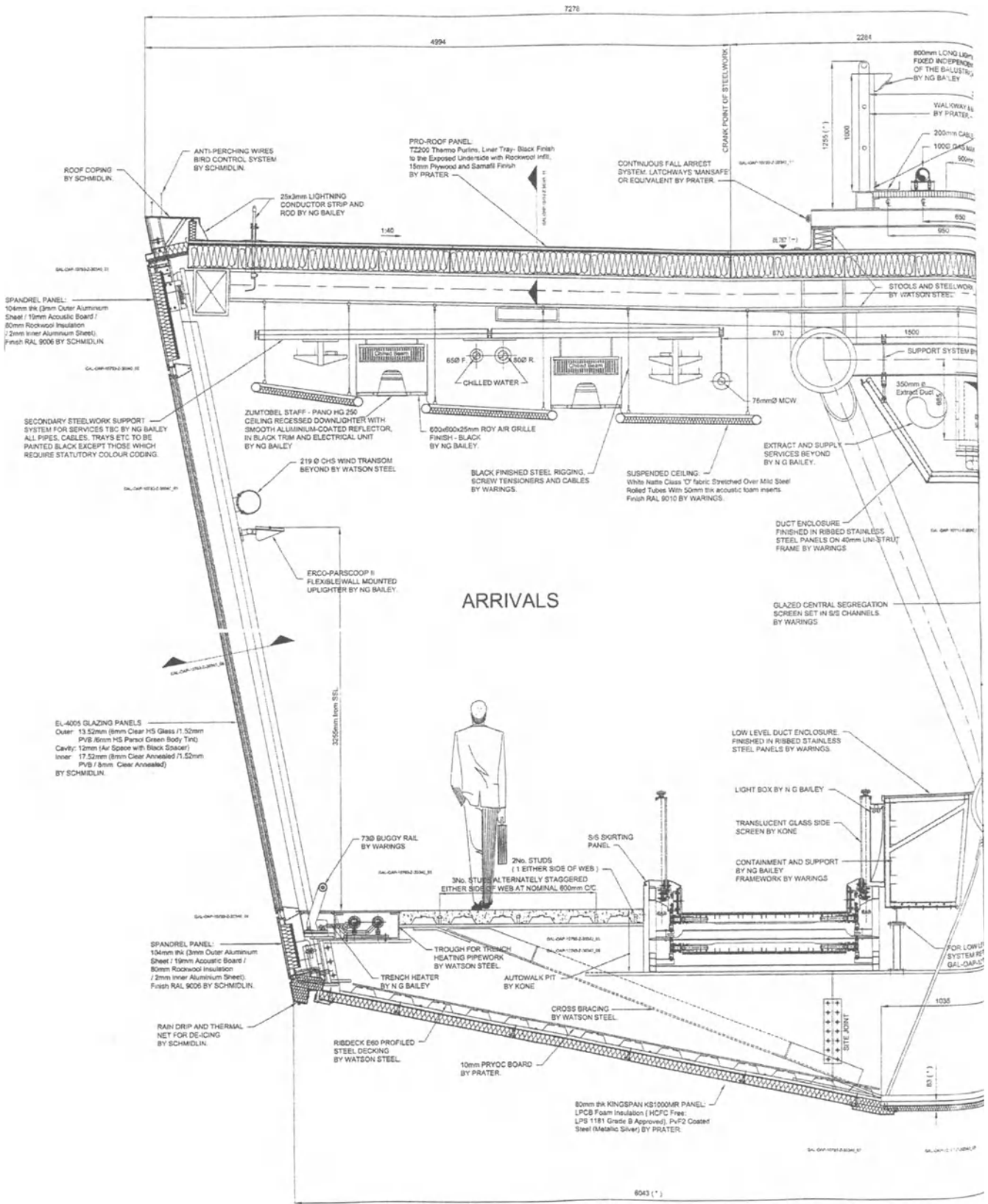
Fig. 10-2 A half-Section of the portion of a building to illustrate, the numerous instances where details will be required to show and communicate the work to be done.
