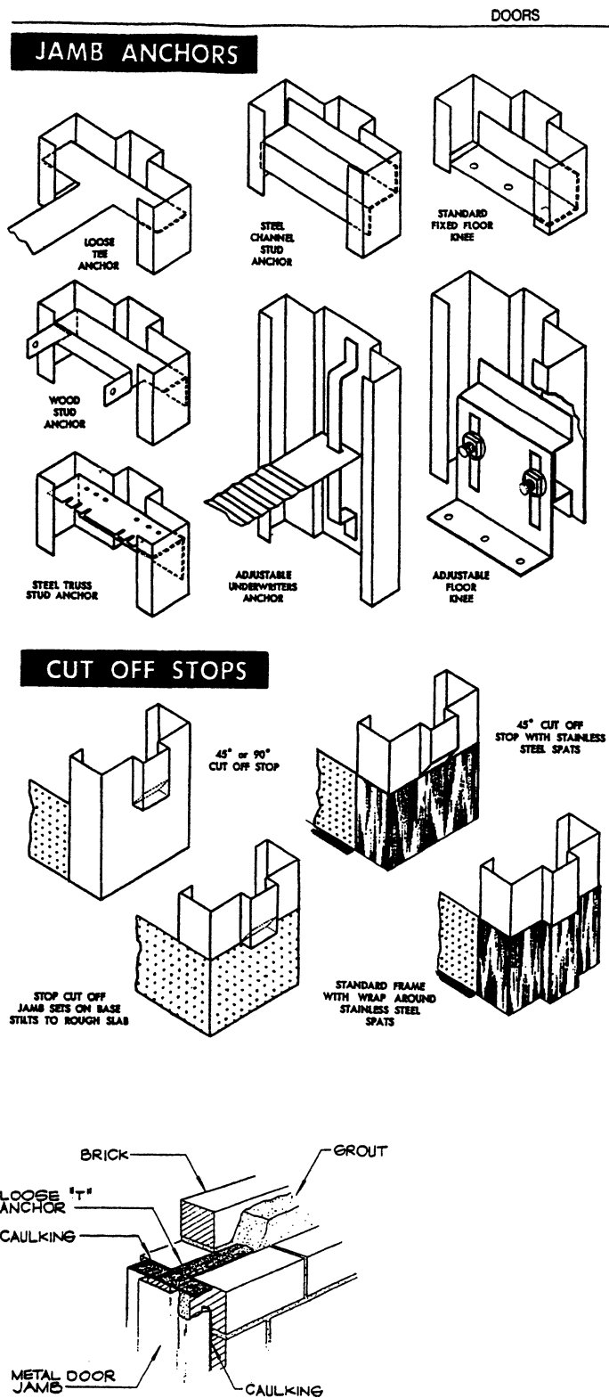
Fig. 12-15 Manufacturer's details showing anchors and stops available on hollow metal door frames
