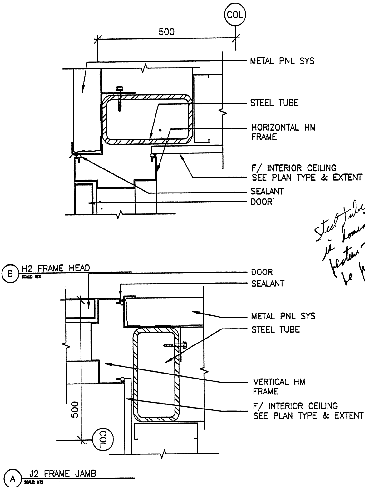
Fig. 10-40 These are door frame details and the fit into the walls, yet the frames are hardly distinguishable— not the sign of a good detail; structural tube is too dominate
