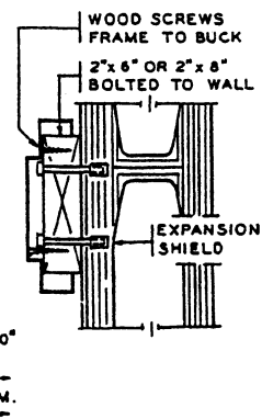
(3) Frame attached to block face scale 1 1/2" = 1'-0"
