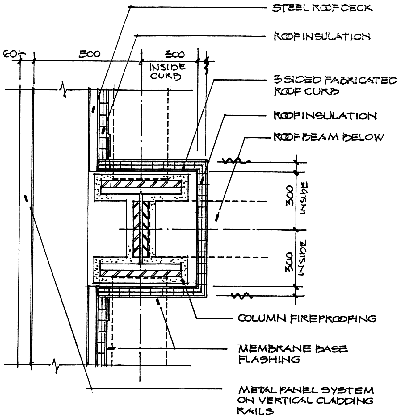
Fig. 10-81 Plan view Section associate with Fig. 10-80; see notes above
