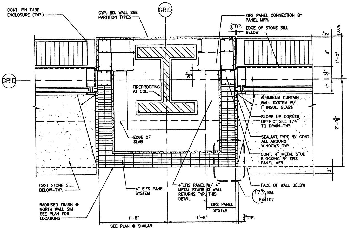
TYPICAL COLUMN DETAIL SCALE: 1 1/2"=1'-0" ● 2ND, 3RD, & 4TH FLOORS SEE UPPER FLOOR PLANS 145 B44106
