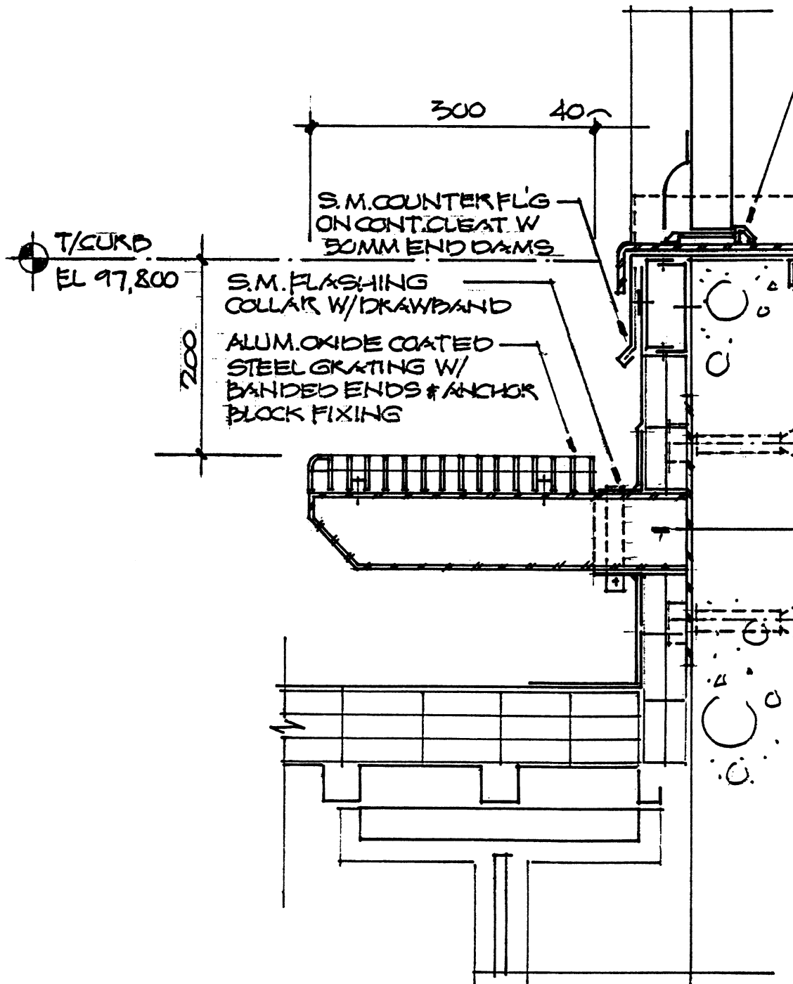
Fig. 10-86 Section detail of a metal grating step from a rooftop penthouse to the adjacent roof. Note how the line work draws the eye to the more important items being shown and lets the ancillary work regress [since it is not as important to this detail]
