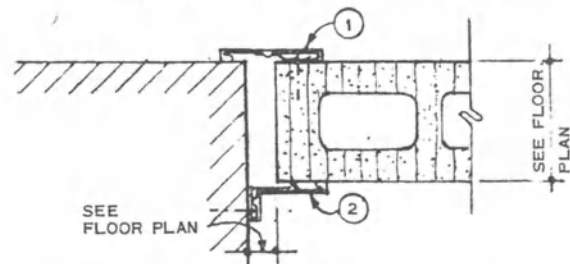
D EXPANSION JOINT AT CORRIDOR
