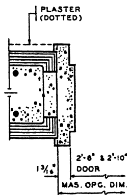
(2) 2'-6" and 2'-10" doors
