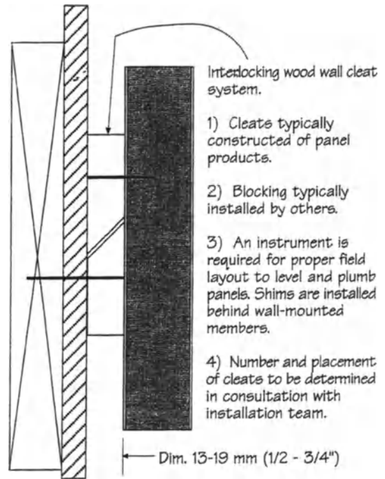
Figure 1700-03 - Wood Interlock
