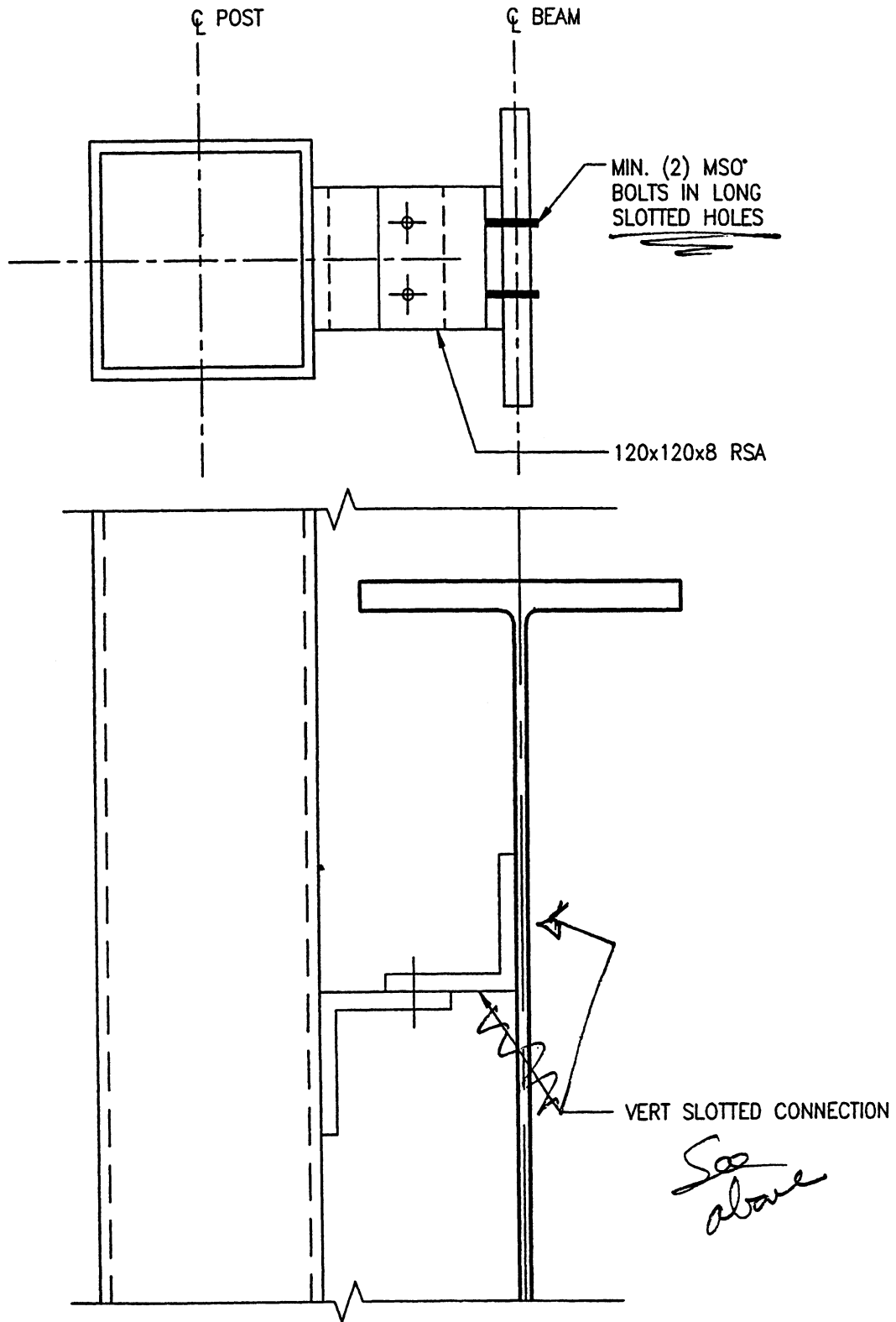
Fig. 10-55 Coordination problem, in that note in lower detail does not reflect condition shown in upper detail. Holes in horizontal legs of angles are drilled round and are not slotted as called for in vertical leg
