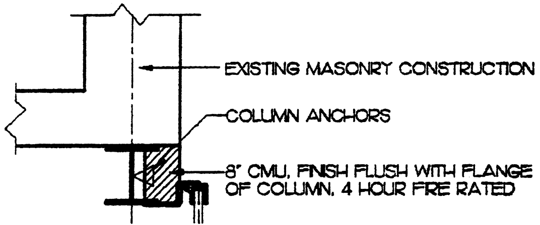
Fig. 10-8 Merely a problem of scale. Lot of information but difficult to read
