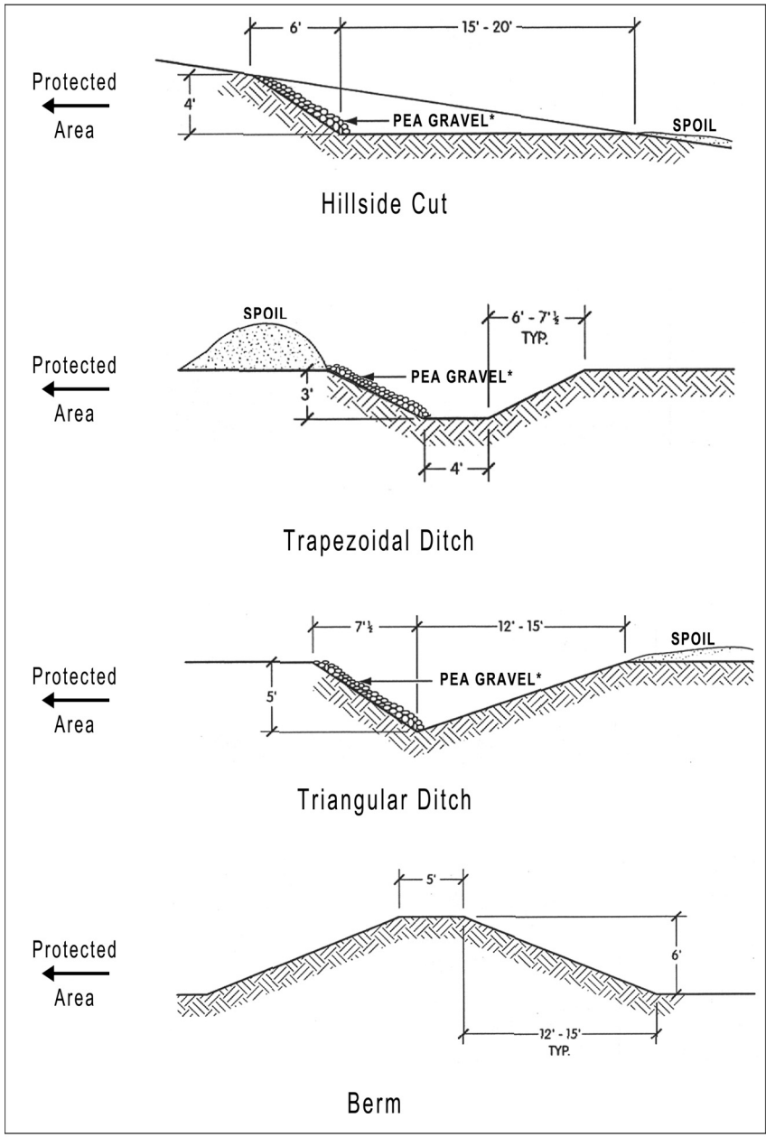
Figure 12.17 Excavation Barriers
