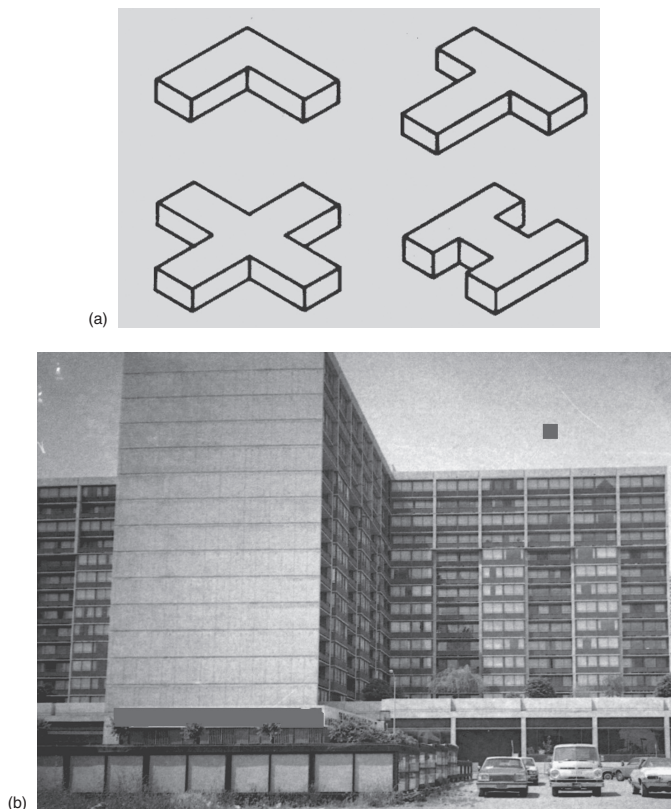
Figure 10.12 Reentrant corner plans: (a) Some plan types. (b) T-shaped building with two reentrant corners.
