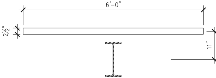
Figure 15.13 Composite Beam Section
