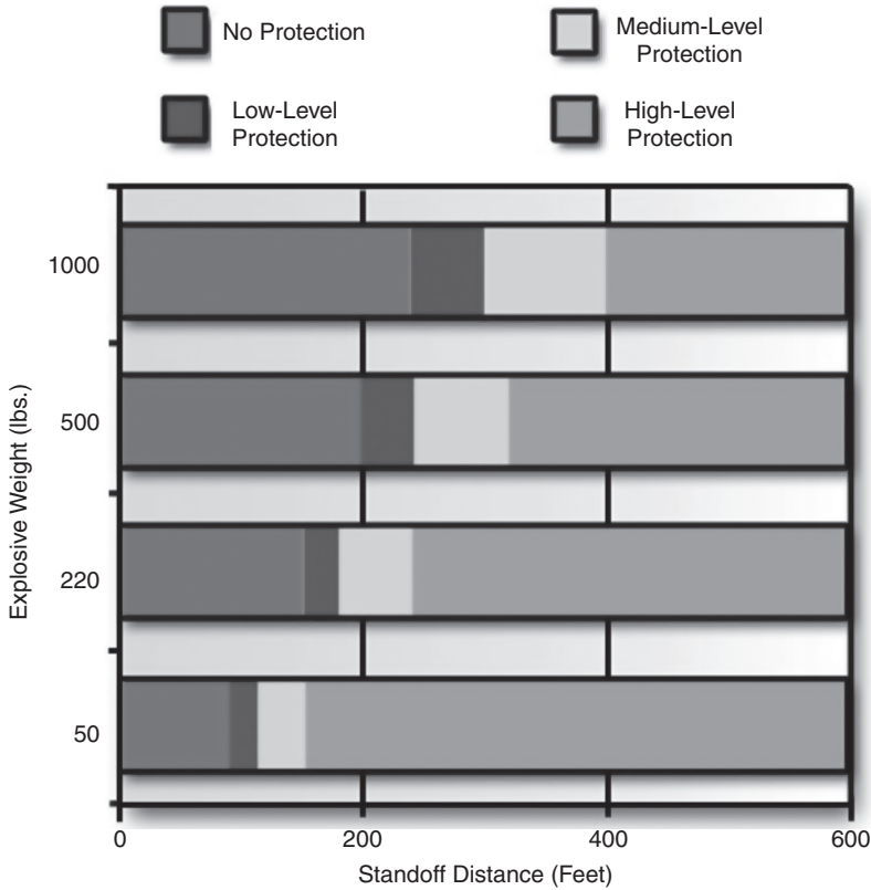
Figure 12.3 Effects of Standoff Distance for a Typical Conventionally Constructed Facility (explosive weight is in lbs of TNT equivalent)
