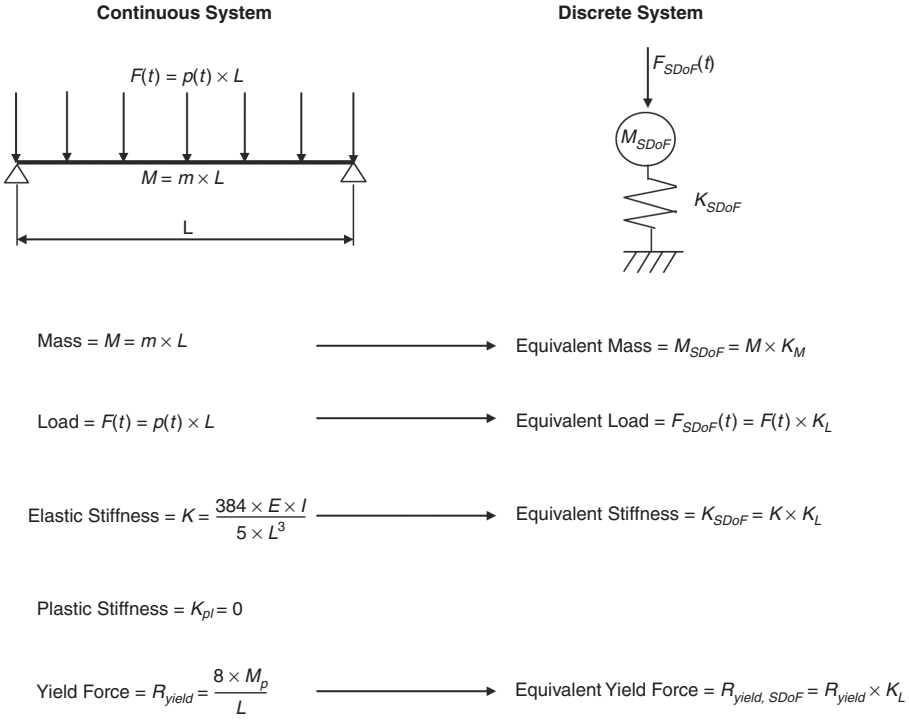
Figure 15.7 MDOF to SDOF Simplification
