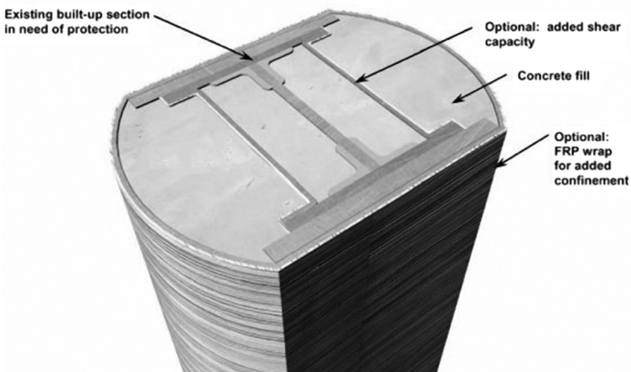
Figure 17.8 Example of the infill concept for preventing web and flange failure (Mode 3) for steel sections
