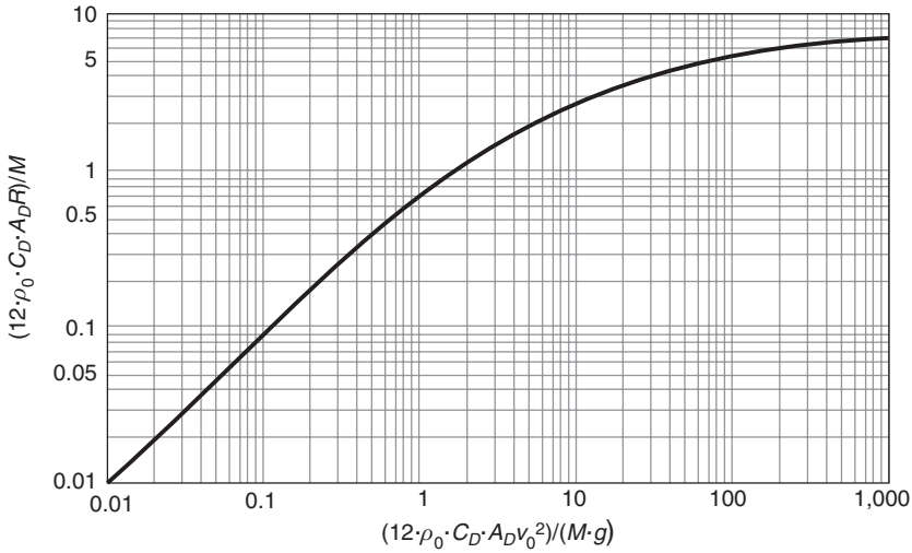
Figure 8.8 Fragment Range Prediction
