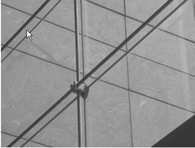
Figure 10.6 Example of Point and Cable Supported Curtain Wall
