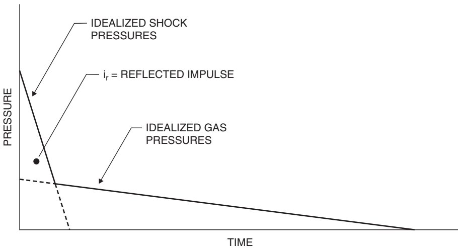
Figure 7.13 Approximate Loading from Confined Explosion
