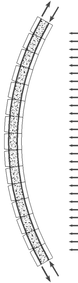
Figure 16.4 Flexural Response Mode of Reinforced Masonry
