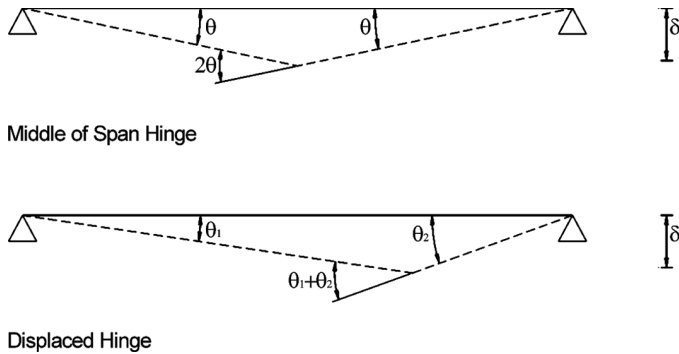
Figure 15.1 Hinge Rotation versus Connection Rotation
