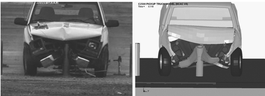
Figure 12.7 Front View of Impact versus Analysis Result (Compliments of Applied Research Associates, Inc.)
