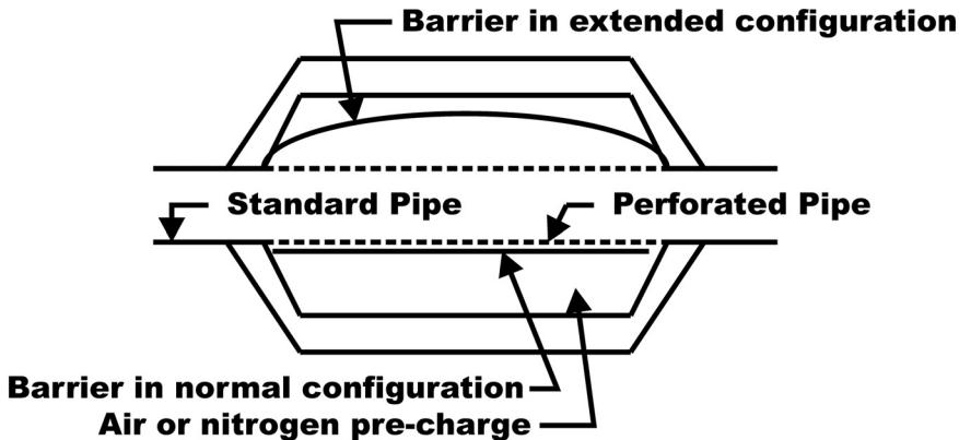
Figure 13.6 Conceptual Design of Accumulator (After U.S. Department of the Army, 1986)
