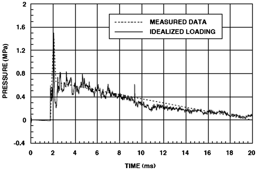
Figure 7.12 Loading from Confined Explosion
