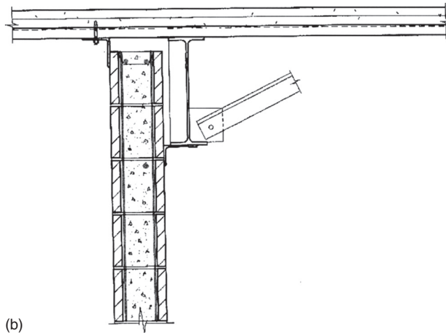
Figure 16.11 Examples of Bond Beam
