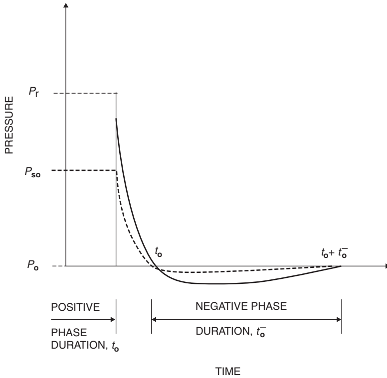
Figure 6.5 Comparison of Free Field and Reflected Blast Loads
