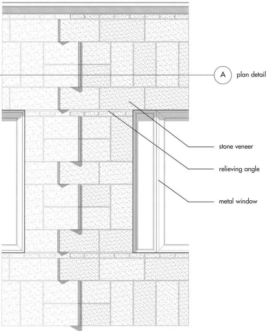
elevation detail
