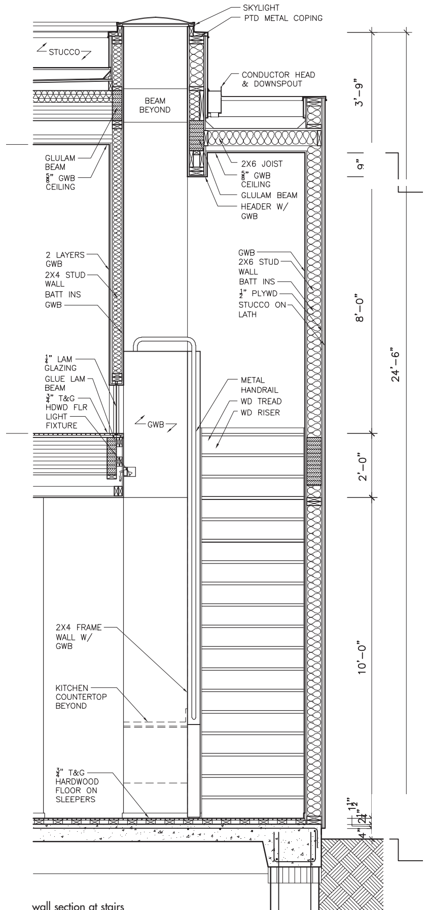
wall section at stairs
