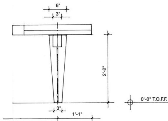
8 ELEVATION TABLE LEG 3" = 1'-0"
