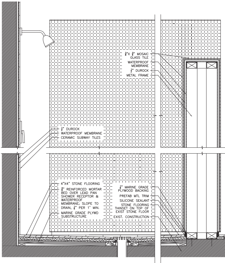
section detail at pool shower
