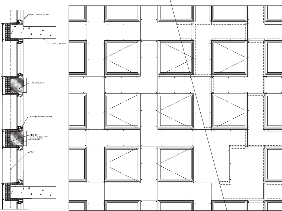
wall section
