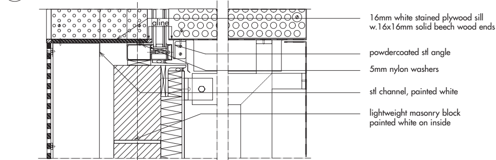
2 window type A, sill scale 1:5
