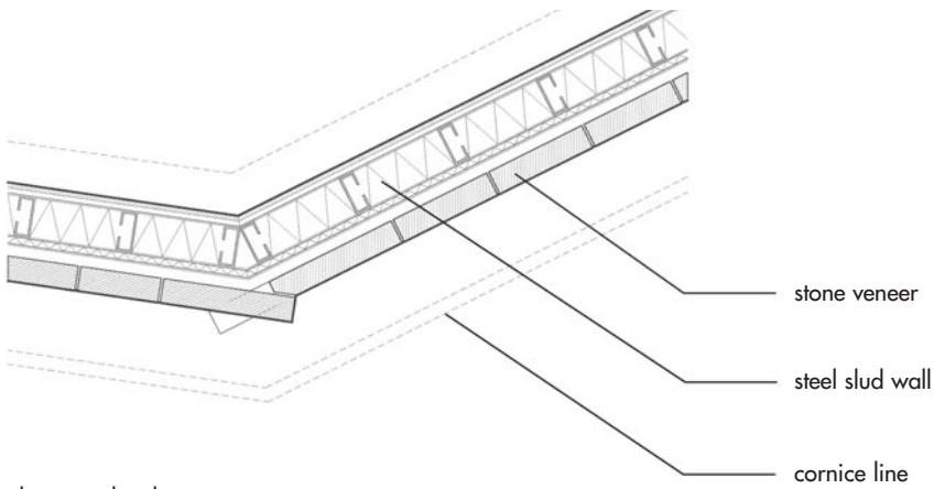
elevation detail
