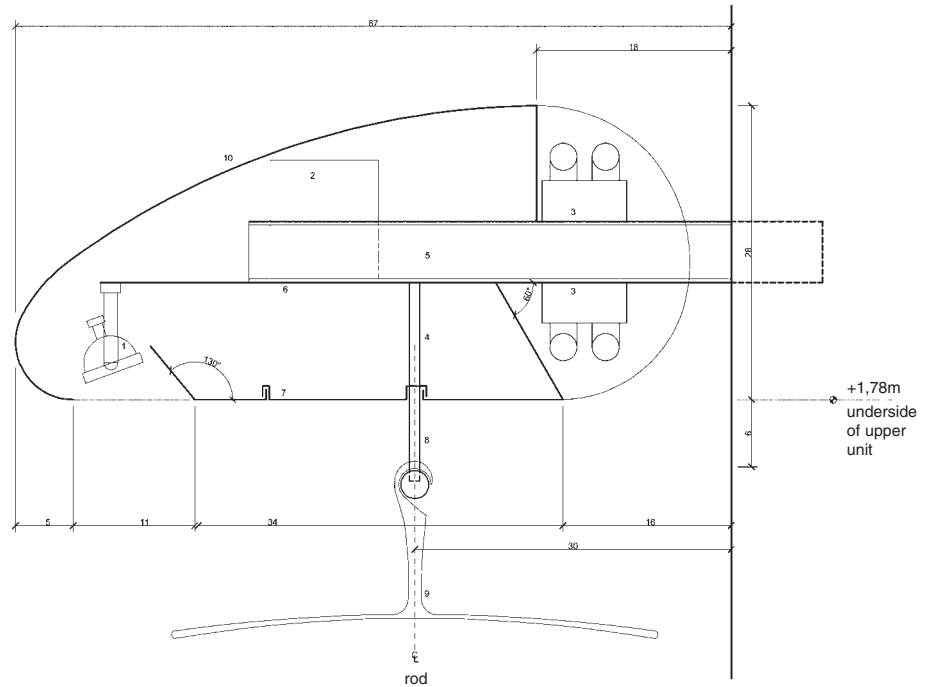
detail section @ upper hanging unit
