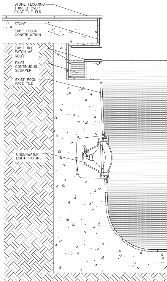
pool coping detail
