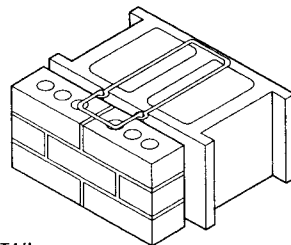
ADJUSTABLE UNIT TIES—MASONRY
