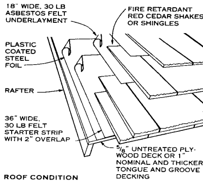
ROOF CONDITION
