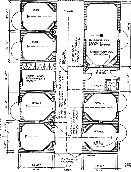
BROODMARE BARN - 7 STALLS - REFER TO NOTES
