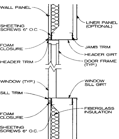
DOOR/WINDOW HEAD AND SILL DETAIL
