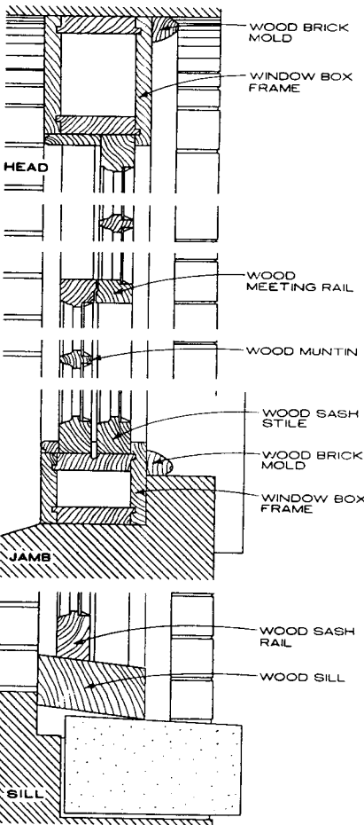
LATE 19TH CENTURY MILL WINDOW
