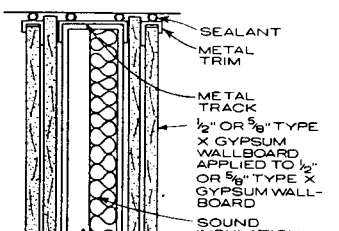
CEILING CONDITION
