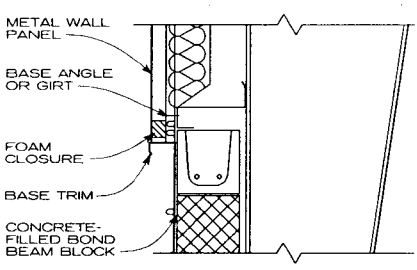
MASONRY WALL AND METAL PANEL CONNECTION
