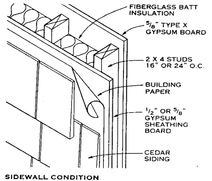
SIDEWALL CONDITION
