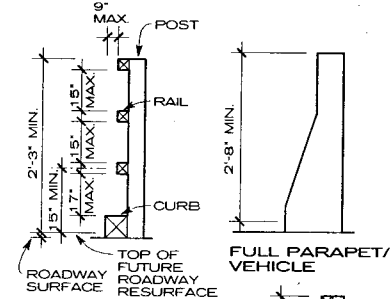
BRIDGE EDGE CONDITION
