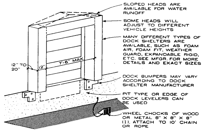
CUSHIONED DOCK SHELTER
