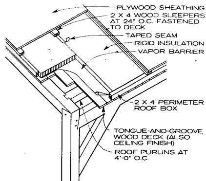
WOOD SLEEPERS AND TONGUE-AND-GROOVE CEILING ON ROOF PURLINS
