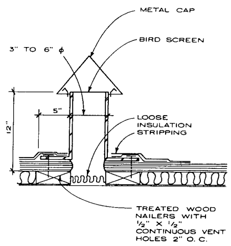
ROOF RELIEF VENT
