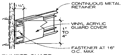
BUMPER GUARD
