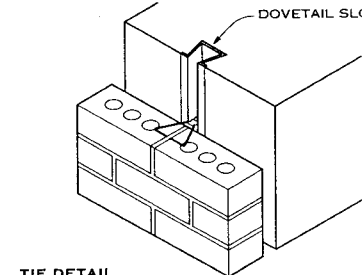
UNIT TIES—CONCRETE
