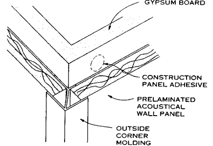
OUTSIDE CORNER
