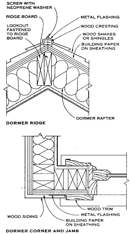
DORMER CORNER AND JAMB
