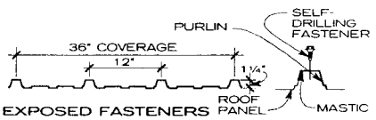
EXPOSED FASTENERS
