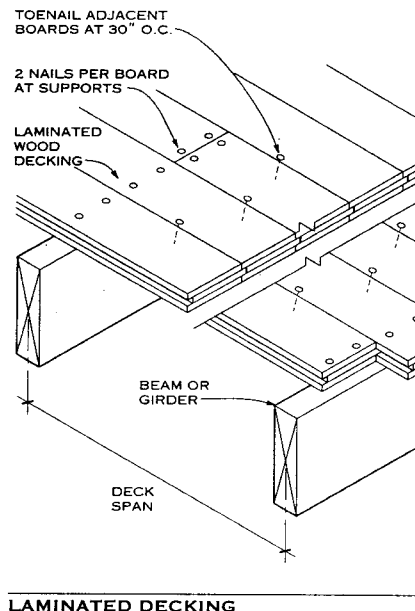
LAMINATED DECKING
