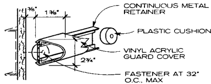
BUMPER GUARD
