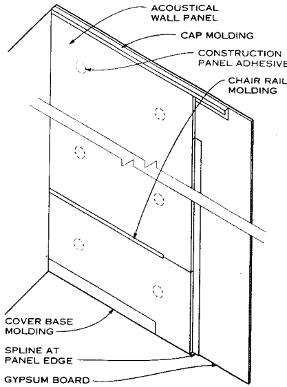
TYPICAL ACOUSTICAL WALL PANEL APPLICATION
