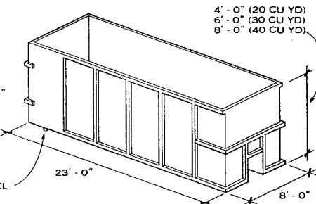
CONVENTIONAL "ROLL OFF" WASTE CONTAINER
