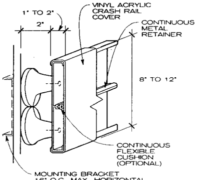
WALL-HUNG
