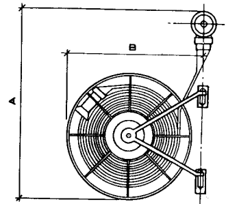
SWING REEL 1 1/2" AND 2 1/2" LINED HOSE
