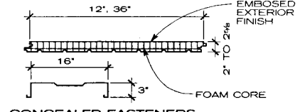
CONCEALED FASTENERS
