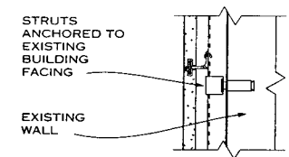
CONNECTION TO EXISTING FACING
