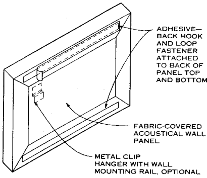
WALL PANEL MOUNTING DETAIL
