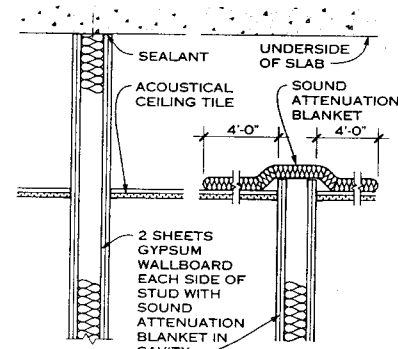
TYPICAL ACOUSTICAL WALL PANEL APPLICATION
