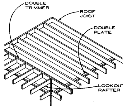
FLAT ROOF
