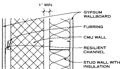
DOUBLE WALL—CMU AND STUD
