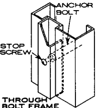
THROUGH BOLT FRAME ANCHOR LABEL AVAIL.
