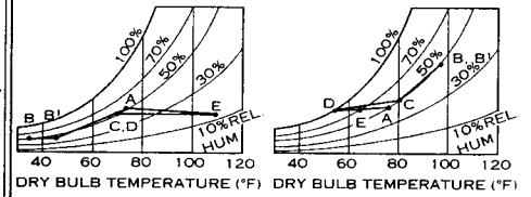
PSYCHROMETRIC CHART—WINTER
