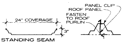
STANDING SEAM
