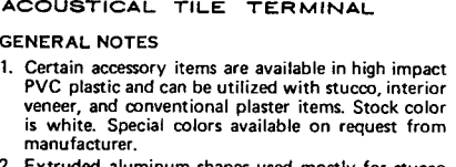
ACOUSTICAL TILE TERMINAL
