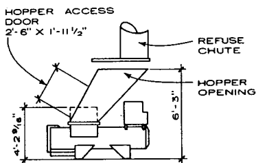
UNIT "A" COMPACTOR UNIT WITHOUT CONTAINERS
