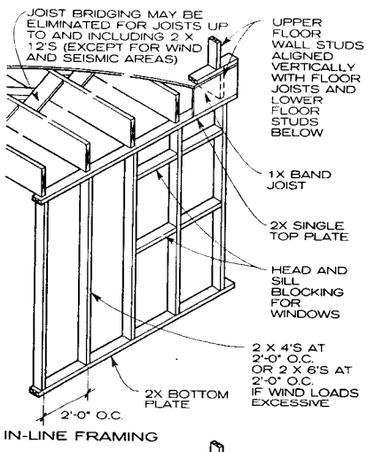
IN-LINE FRAMING
