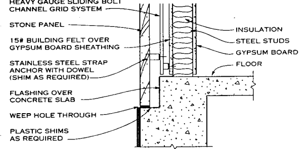
STONE SPANDREL AT GRADE
