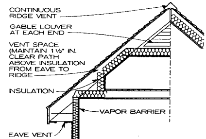
GABLE WITH OCCUPIED SPACE UNDER ROOF
