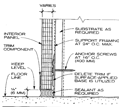
PANEL AT SILL
