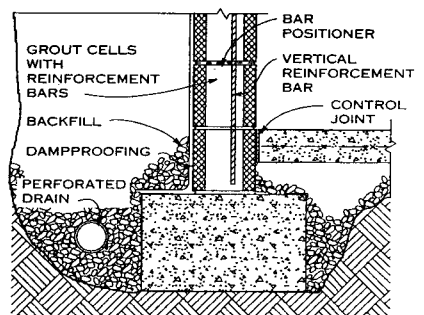
REINFORCED FOUNDATION WALL DETAIL
