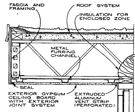
EXTERIOR SOFFIT
