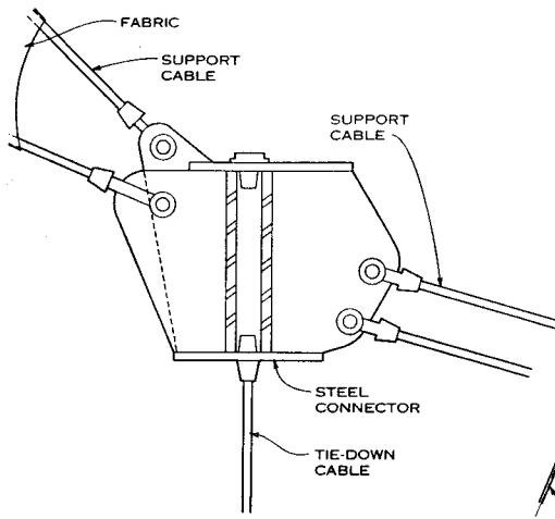
TIE-DOWN SECTION
