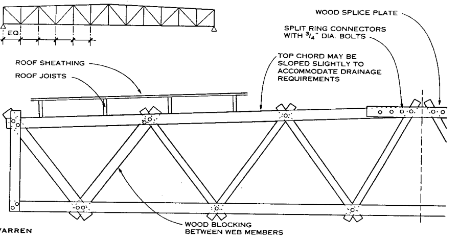
WARREN
