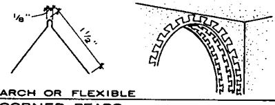
ARCH OR FLEXIBLE CORNER BEADS
