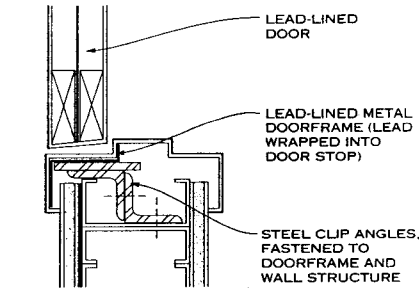
REINFORCED JAMB
