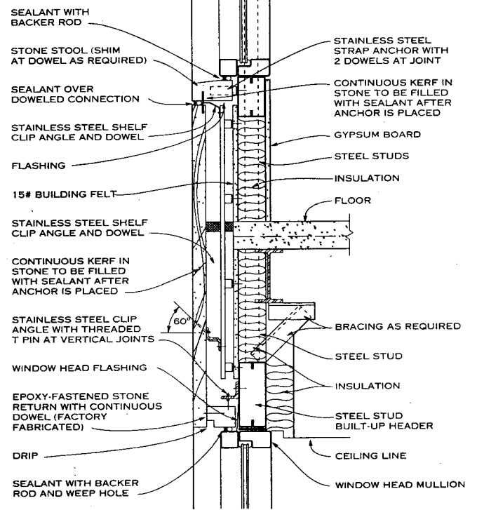
STONE SPANDREL AT WINDOW HEAD AND SILL
