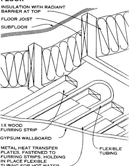
HEAT TRANSFER THROUGH CEILING
