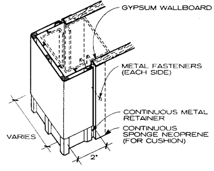
WALL-END GUARD
