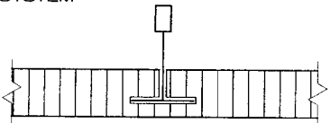
KERFED EDGE TILE, CONCEALED T SYSTEM
