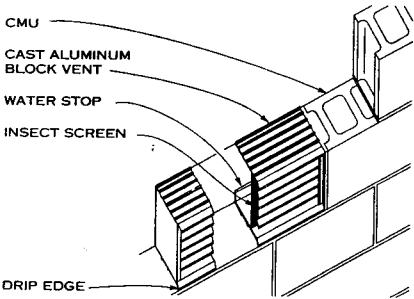
BRICK OR BLOCK VENT
