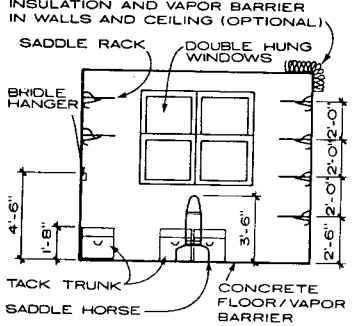
TACK ROOM ELEVATION SERVES 40 STALLS - HEAT AND HUMIDITY CONTROL REQUIRED
