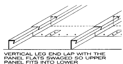
END LAPS FOR METAL ROOFING PANELS
