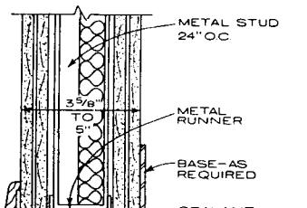
FLOOR CONDITION FIRE RATING 2HR STC 50 TO 54
