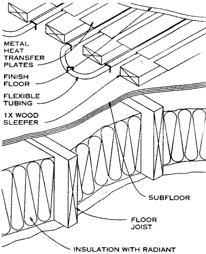
HEAT TRANSFER AT SUSPENDED FLOOR
