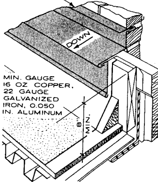
BUILDING EXPANSION JOINTS
