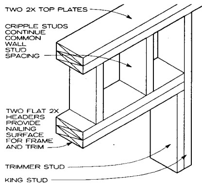
2X PARTITION WALL—HEADER DETAIL
