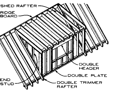
SMALL SHED DORMER
