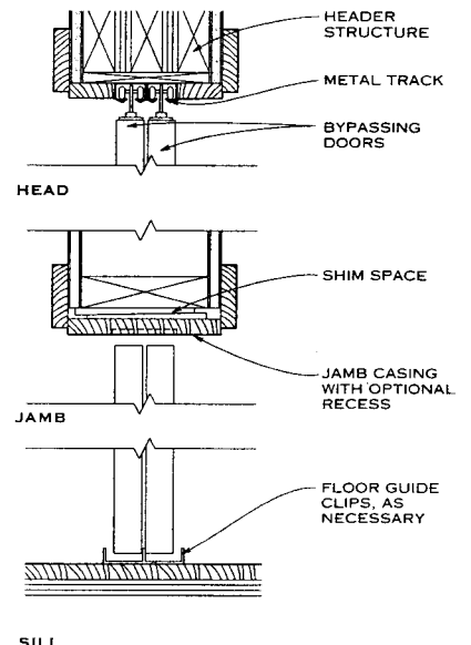
DETAIL—BYPASS DOOR
