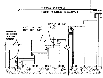
TELESCOPIC BLEACHERS (HIGHRISE)
