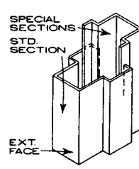
FLUSH SURFACE DOOR AND TRANSOM WELDED OR DRIVEN MULLION
