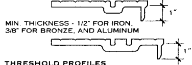
THRESHOLD PROFILES
