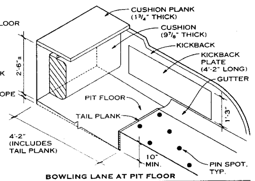
BOWLING LANE AT PIT FLOOR
