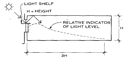
REDIRECTED DAYLIGHT PENETRATION INTO A SPACE
