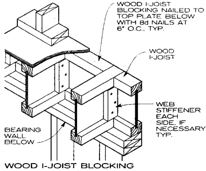
WOOD I-JOIST BLOCKING
