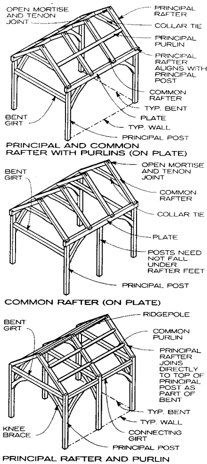
TIMBER FRAME ROOF TYPES
