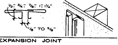
EXPANSION JOINT
