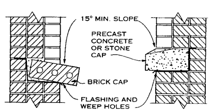
RECESS AND SILL DETAILS IN BRICK WALLS
