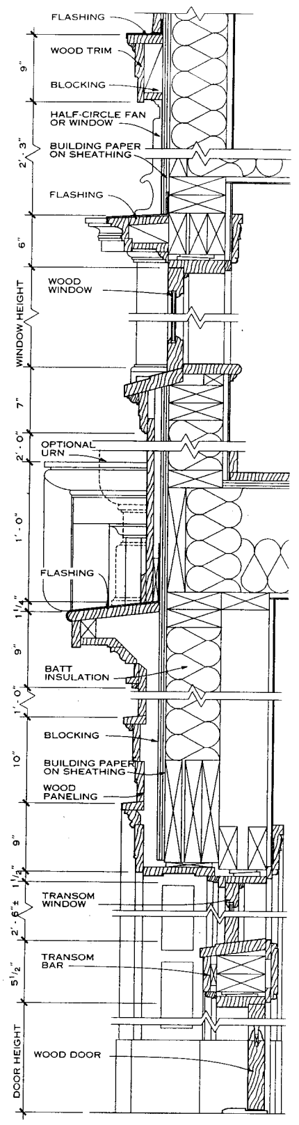
VERTICAL SECTION
