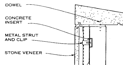
COPING
