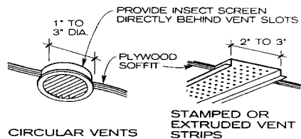
EAVE VENTILATION TYPES
