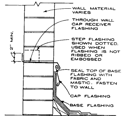
MASONRY WALL
