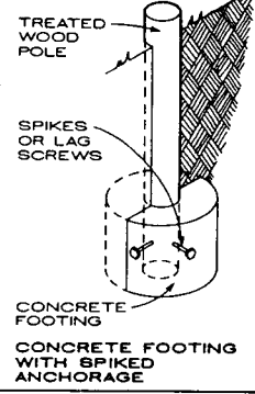
CONCRETE FOOTING WITH SPIKED ANCHORAGE
