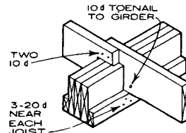
OVERLAPPING JOISTS NOTCHED OVER GIRDER BEARING ONLY ON LEDGER, NOT ON TOP OF GIRDER
