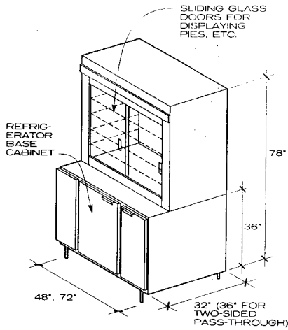
DISPLAY REACH-IN REFRIGERATOR
