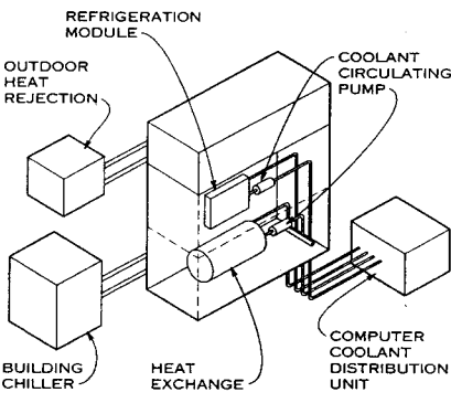
COMBINED HEAT REJECTION IN MAINFRAME COOLING SYSTEM
