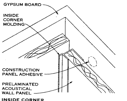
INSIDE CORNER
