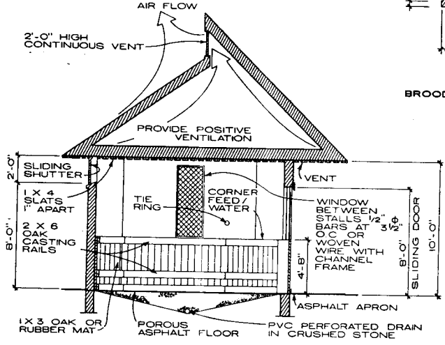
STALL SECTION THROUGH RIDING HORSE BARN
