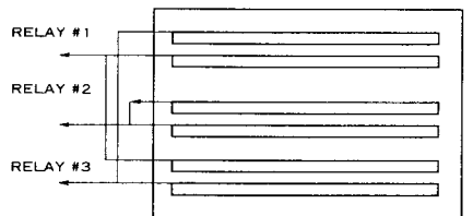
SIX-LAMP FIXTURE WITH THREE 2-LAMP BALLASTS
