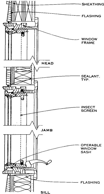
METAL-CLAD WOOD WINDOW IN WOOD CONSTRUCTION
