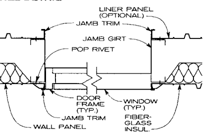
DOOR/WINDOW JAMB DETAIL
