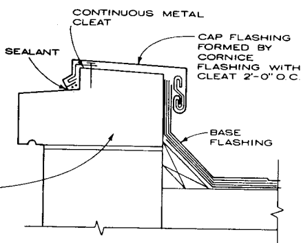
CORNICE FLASHING WITH CAP FLASHING
