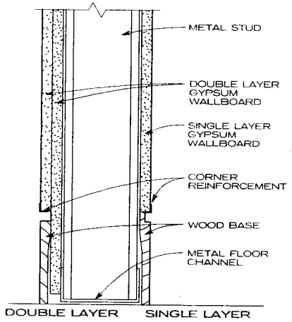
WALL AT WOOD BASE
