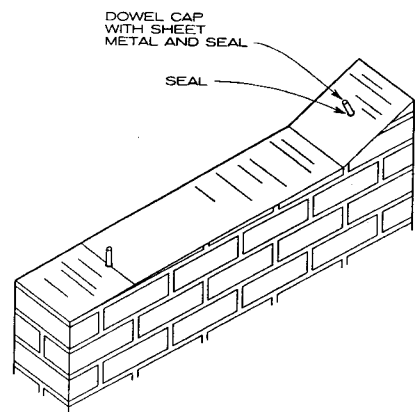
THROUGH-WALL FLASHING UNDER COPING
