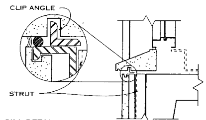
SILL DETAIL
