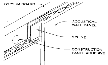
CONCEALED VERTICAL JOINT
