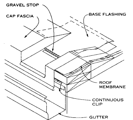
SCUPPER DETAIL AT RAISED CURB
