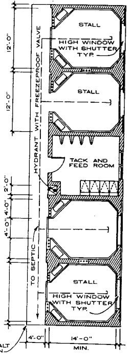
RIDING HORSE BARN 4 STALLS REFER TO NOTES
