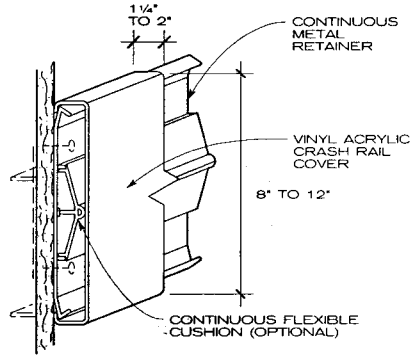
SURFACE-MOUNTED
