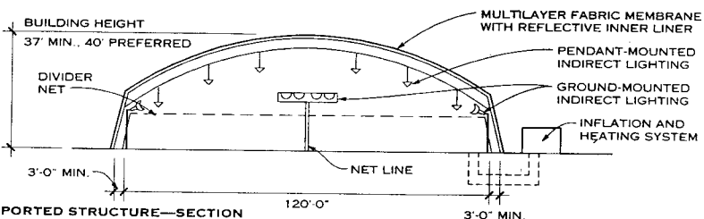
AIR-SUPPORTED STRUCTURE—SECTION
