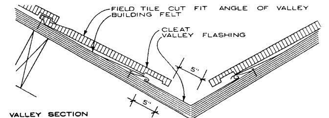
VALLEY SECTION
