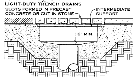
CONCEALED DRAIN
