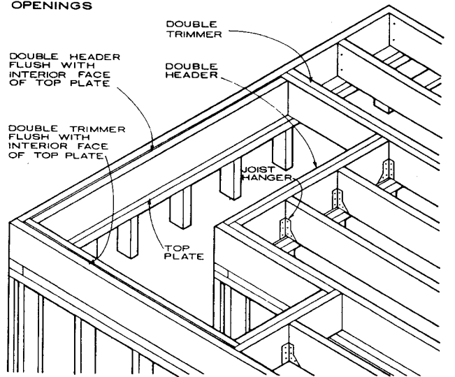
STAIR OPENING AT EXTERIOR WALL
