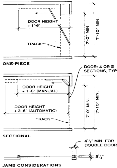
LIFT DOORS—AUTOMATIC OPTIONAL
