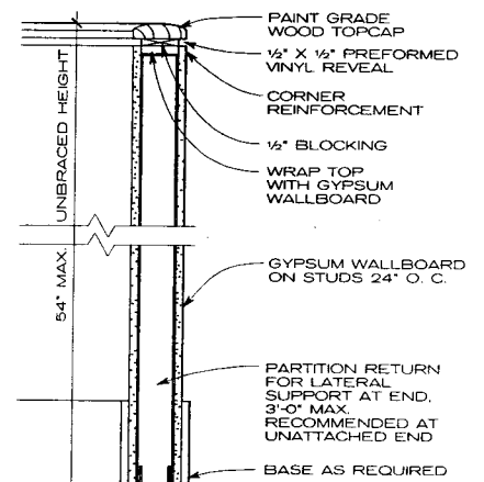
PARTIAL HEIGHT PARTITION
