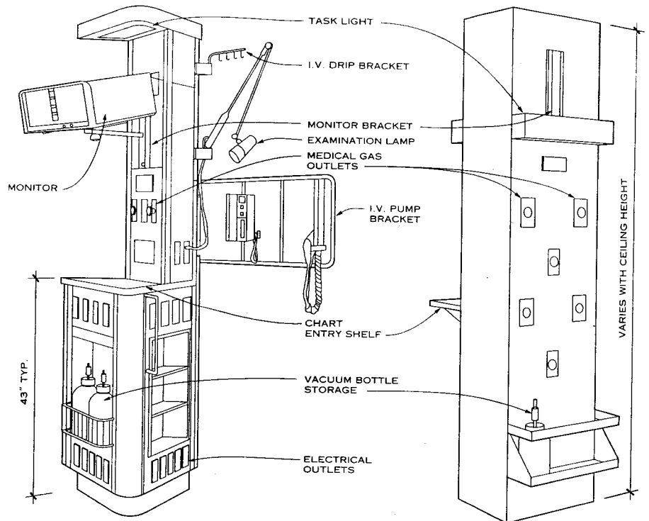
TRIANGULAR MODULE COLUMN
