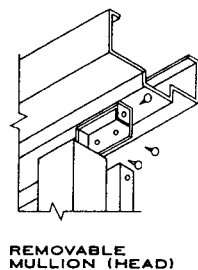
REMOVABLE MULLION (HEAD)
