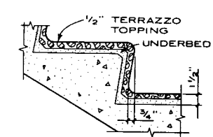
STAIR TREAD AND RISER
