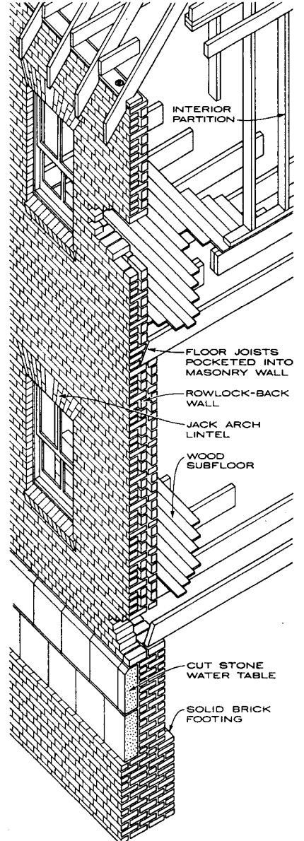
19TH CENTURY BRICK CAVITY WALL
