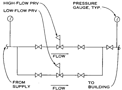
TYPICAL PRESSURE-REDUCING VALVE (PRV) STATION
