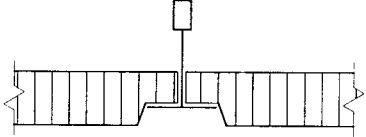
SQUARE-CUT REVEAL TILE, EXPOSED T SYSTEM
