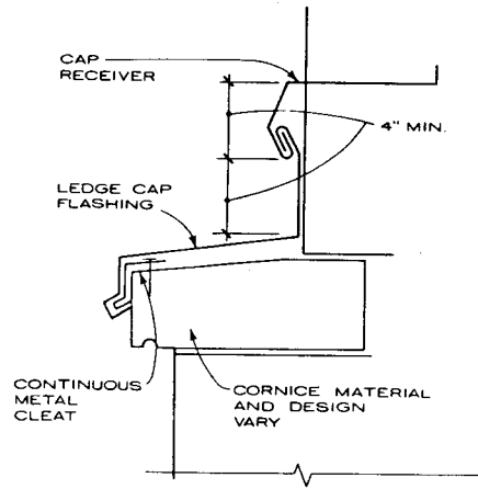
CORNICE LEDGE CAP FLASHING AND RECEIVER
