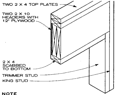
NOTE This detail eliminates cripple studs above opening.
