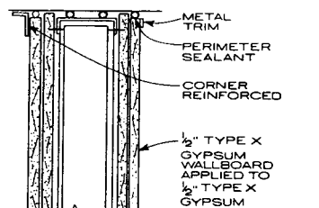
CEILING CONDITION
