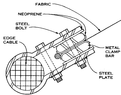
EDGE OR CATENARY CABLE ATTACHMENT DETAIL
