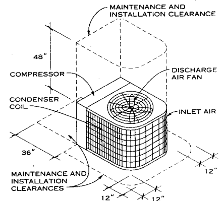
CONDENSING UNIT
