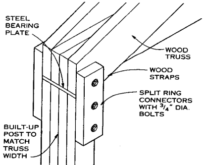
DETAIL—WOOD STRAP AT WOOD COLUMN
