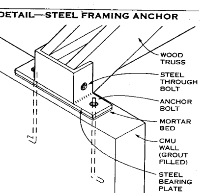
DETAIL—BEARING ON MASONRY WALL
