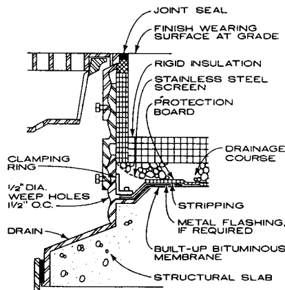
TERMINATION AT DRAIN
