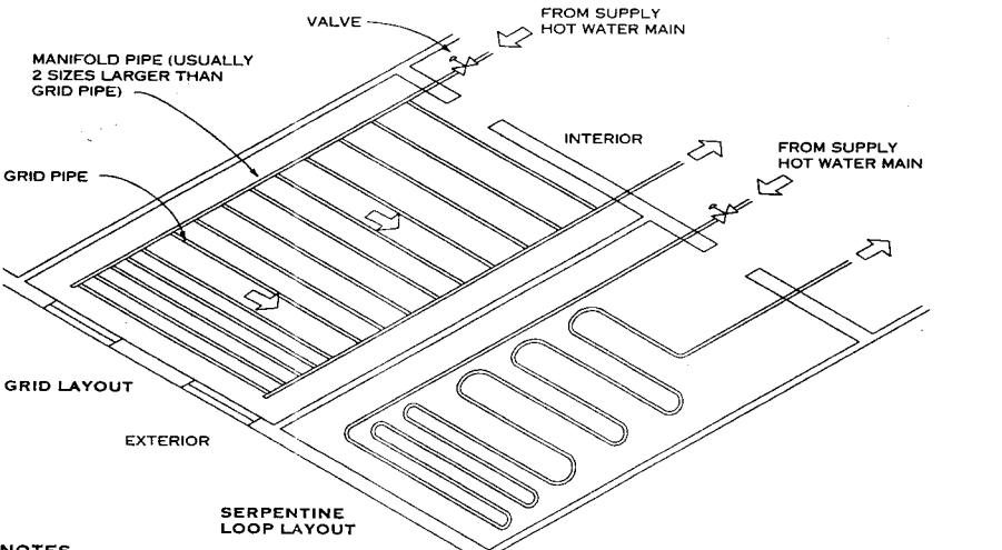
HEAT TRANSFER IN CONCRETE TOPPING SLAB
