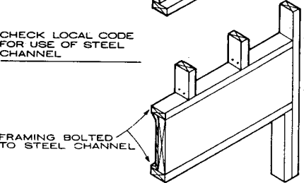
LINTELS FOR WIDE OPENINGS
