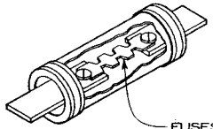
KNIFE BLADE FUSE 1. Rated voltage: 250 and 600 2. Ampere ratings: 70-6000 3. Fuse types: K1, RK1, K5, RK5, J, H, G, and L
