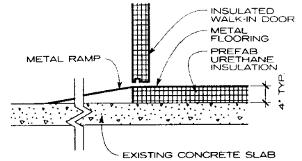
WALK-IN FLOOR OVER BUILDING FLOOR WITH EXTERIOR METAL RAMP
