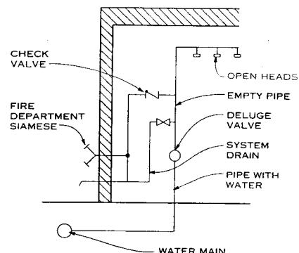
DELUGE SYSTEM
