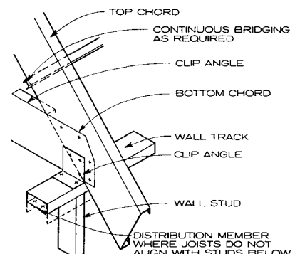
ROOF TRUSS EAVE DETAIL
