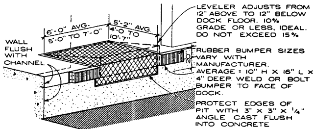
TYPICAL LOADING DOCK BAY
