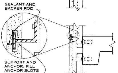
WALL SECTION
