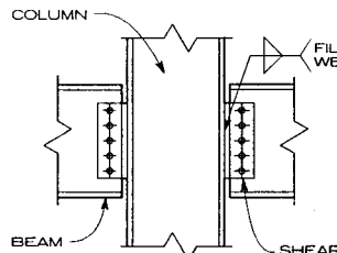
SHOP WELDED TAB FIELD HIGH STRENGTH BOLTED
