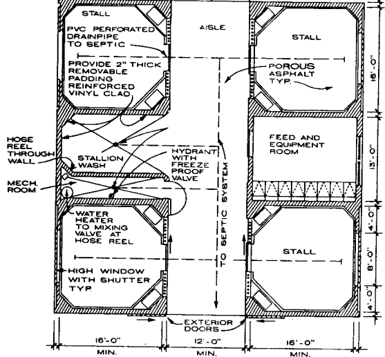
STALLION BARN - 4 STALLS - REFER TO NOTES
