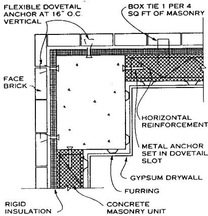
DOVETAIL ANCHORS AT CORNER
