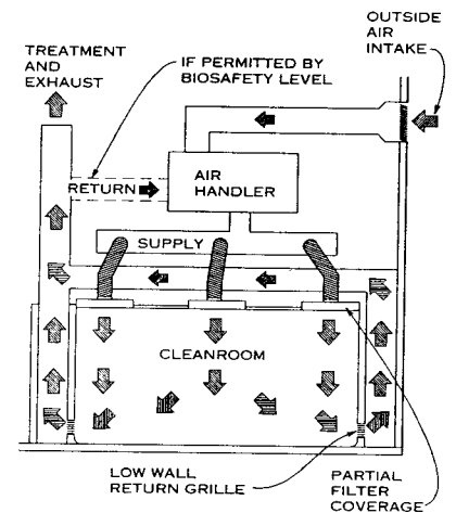
SECTION THROUGH BIOTECHNOLOGY CLEANROOM (CLASS 1000/M4.5)
