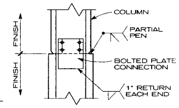
WEB-FIELD H.S. BOLTED FLANGE-PARTIAL PENETRATION
