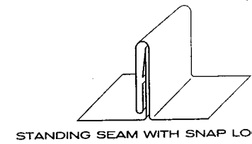
STANDING SEAM WITH SNAP LOCK
