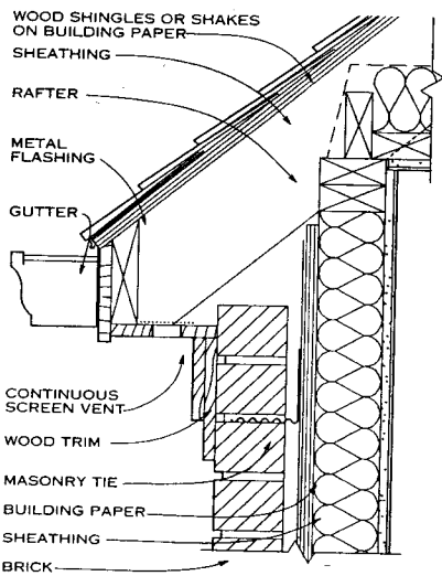
EAVE AT BRICK VENEER
