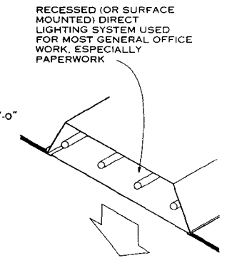
OPEN OFFICE AREA STANDARD 2' X 4' CEILING GRID DIRECT LIGHTING FIXTURE, TYP.
