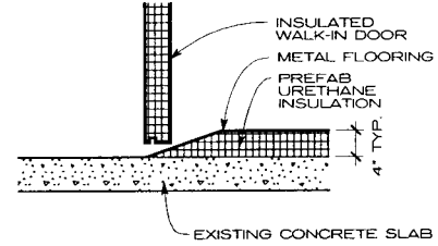
WALK-IN FLOOR OVER BUILDING FLOOR WITH INTERIOR METAL RAMP
