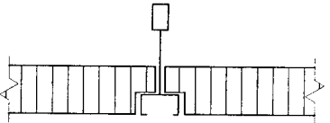
SQUARE-CUT REVEAL TILE, REVEAL T SYSTEM
