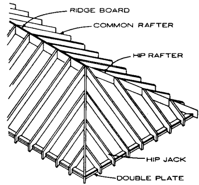
HIP ROOF
