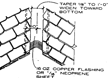
OPEN VALLEY
