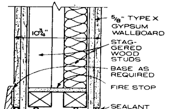
FLOOR CONDITION FIRE RATING 2HR STC 55 TO 59
