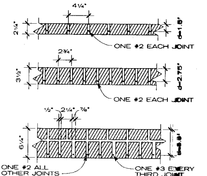
REINFORCED BRICK MASONRY
