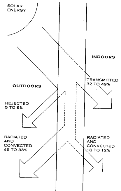
SOLAR PERFORMANCE OF HEAT-ABSORBING OR TINTED GLASS
