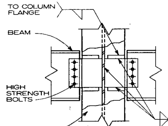
SHOP WELDED TAB TO COLUMN WEB AND PLATES FIELD H.S. BOLTED
