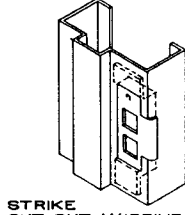
STRIKE CUT-OUT W/REINF AND PLASTER GUARD
