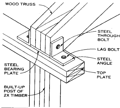
DETAIL—STEEL ANGLE BRACE TO WOOD PLATE
