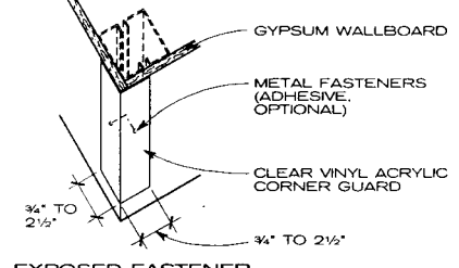
EXPOSED FASTENER
