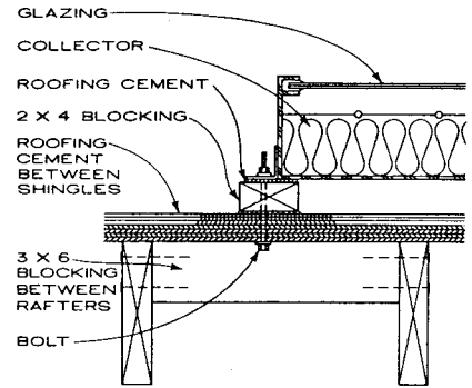
SLOPED ROOF
