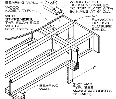
NOTE Joist must be designed to carry the load-bearing wall. LOAD-BEARING CANTILEVER DETAIL
