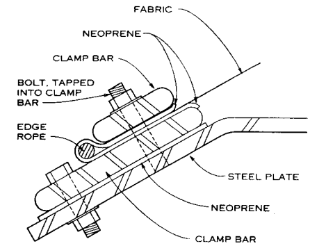
FABRIC EDGE CLAMP ATTACHMENT DETAIL
