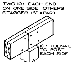
TWO PIECE GIRDER GIRDER JOINTS ONLY AT SUPPORTS STAGGER JOINTS
