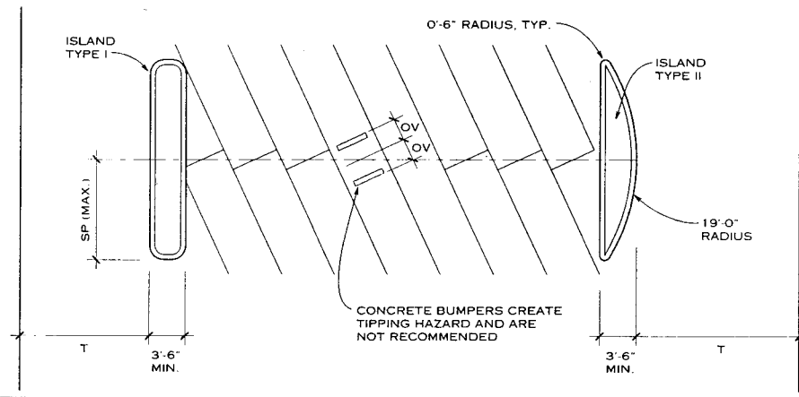
TYPICAL PARKING BAY WITH ISLAND TYPES
