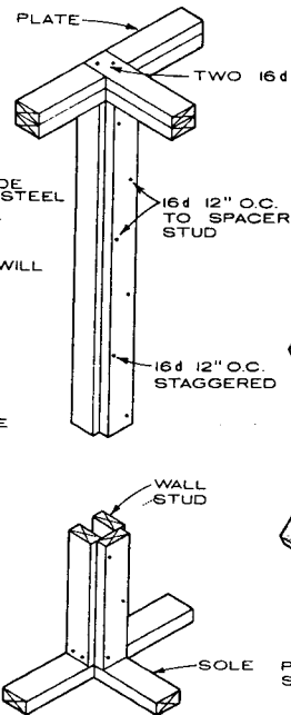
PARTITION TO WALL CONNECTION
