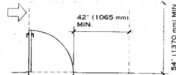
HINGE APPROACH
