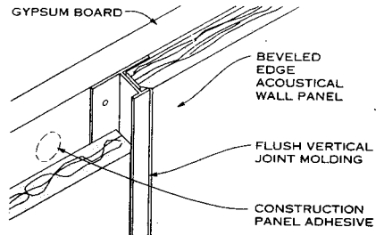
FLUSH VERTICAL JOINT
