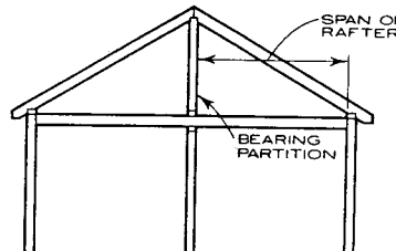
GABLE ROOF (SLOPE UNDER 3 IN 12)
