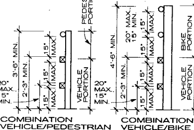
TYPICAL RAIL SYSTEMS
