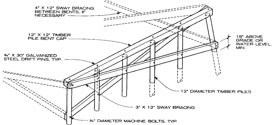
TYPICAL PILE BENT DETAIL
