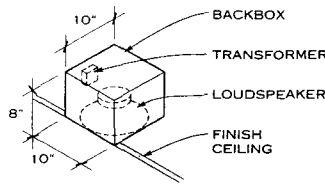
FULL-RANGE CEILING LOUSPEAKER
