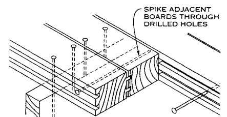
SOLID DECKING
