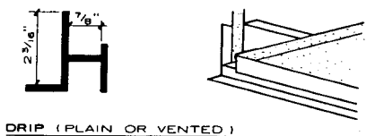
DRIP (PLAIN OR VENTED) SCREEDS
