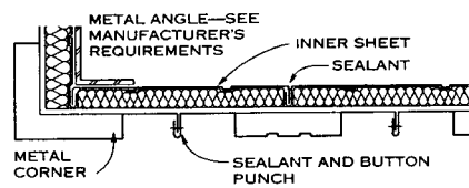
OUTSIDE CORNER
