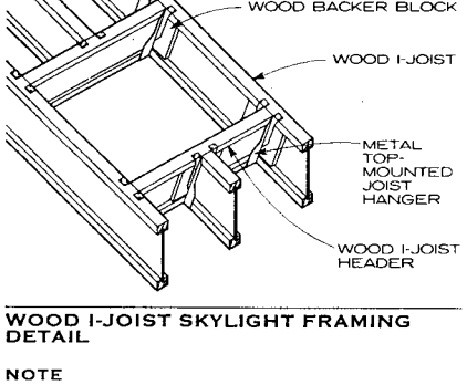
NOTE Check code and manufacturer's requirements for all ventilation hole sizes cut in blocking web.
