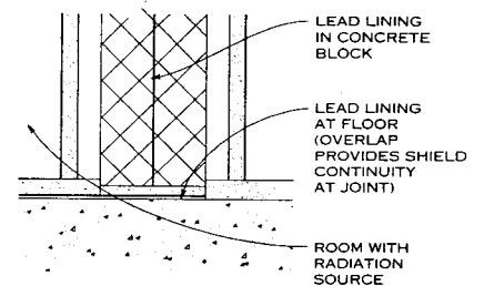
LEAD-LINED BLOCK IN CONCRETE FRAME
