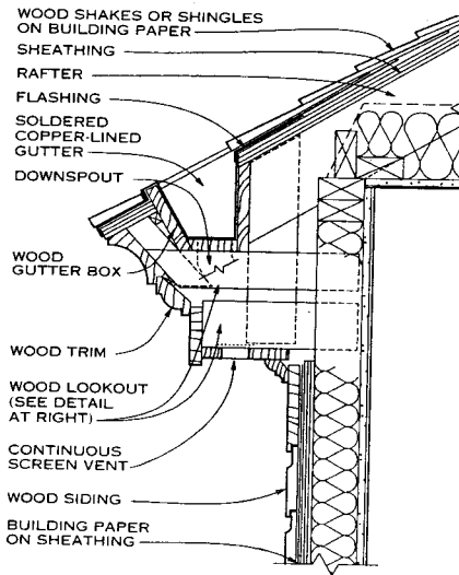
EAVE WITH BUILT-IN GUTTER
