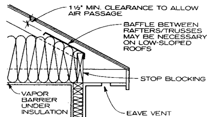
INSULATION BLOCKING AND BAFFLE
