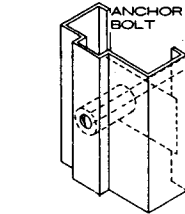
THROUGH BOLT FRAME ANCHOR
