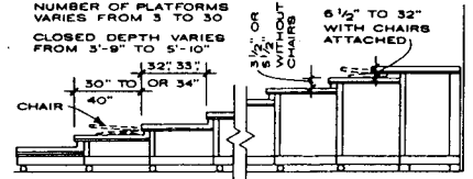
TELESCOPIC PLATFORM
