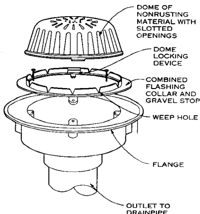
ROOF DRAIN
