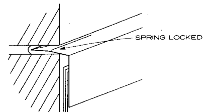
SPRING LOCKED INSERT FLASHING DETAIL
