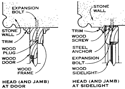
WOOD FRAME DETAILS
