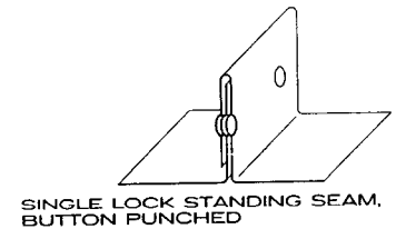
SINGLE LOCK STANDING SEAM
