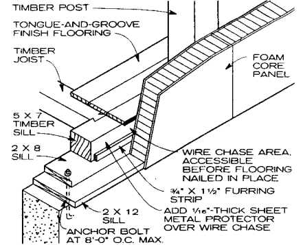
TIMBER-SILL WIRE CHASE DETAIL
