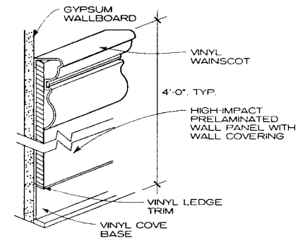
WAINGSOT PANEL WALL GUARD
