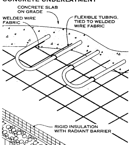
HEAT TRANSFER IN SLAB ON GRADE
