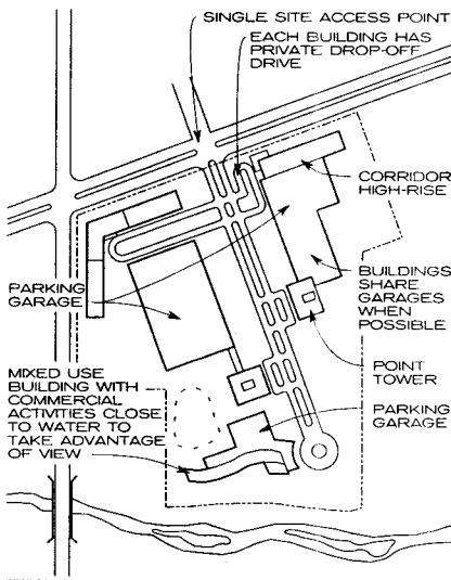
SITE PLAN
