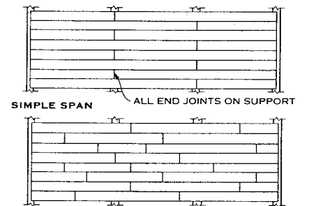
WOOD DECKING JOINT PATTERNS
