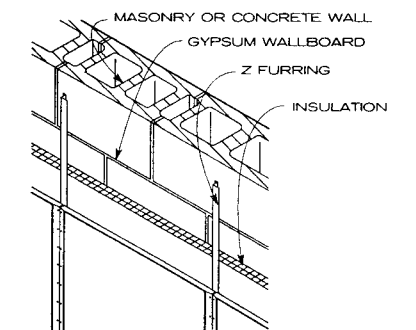
FURRING CHANNELS
