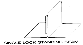
SINGLE LOCK STANDING SEAM
