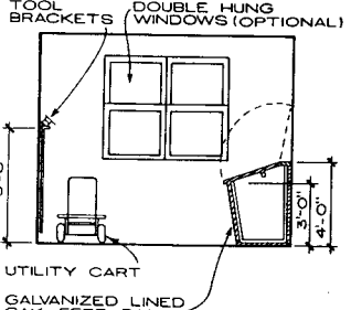
FEED AND EQUIPMENT ROOM ELEVATION CAPACITY OF ONE BIN = 100 LB VENTILATION REQUIRED
