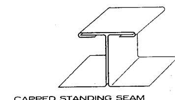
CAPPED STANDING SEAM
