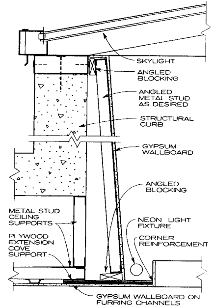
SKYLIGHT
