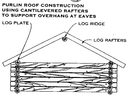
SECTION—LOG RAFTER CONSTRUCTION
