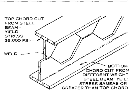
CASTELLATED BEAMS
