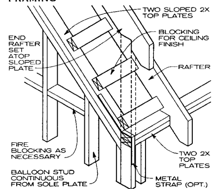
RAKE WALL DETAIL—BALLOON FRAMING
