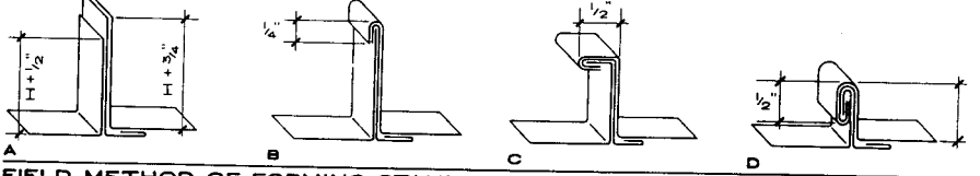
FIELD METHOD OF FORMING STANDING SEAM
