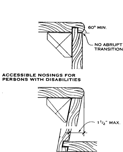
ACCESSIBLE NOSINGS
