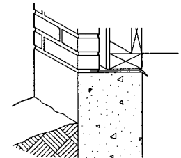
BRICK VENEER WALL
