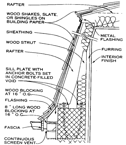
MANSARD ROOF
