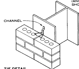
UNIT TIES—STEEL FRAME
