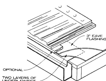
CEMENT WOOD TILE LAYOUT
