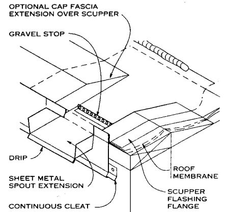
RAINSPOUT DETAIL
