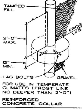
REINFORCED CONCRETE COLLAR
