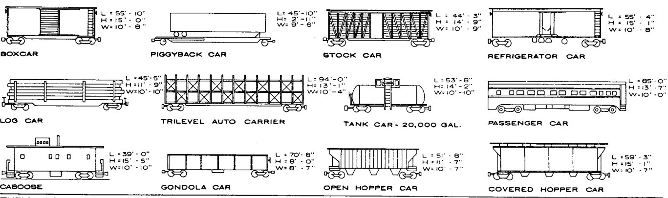
TYPICAL RAILROAD CAR TYPES AND SIZES (ACTUAL CAR SIZES VARY GREATLY EVEN AMONG LIKE CAR TYPES)
