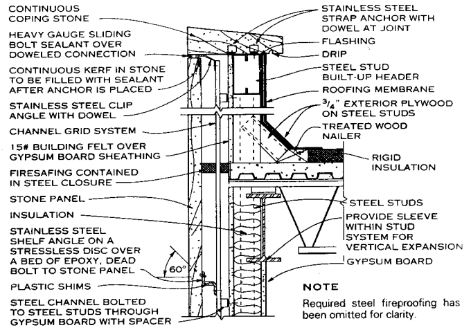
SECTION AT ROOF PARAPET AND WINDOWLESS WALL
