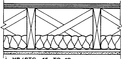
1 HR / STC 45 TO 49 ELECTRIC RADIANT HEAT PANEL
