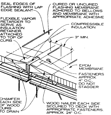
EXPANSION JOINT
