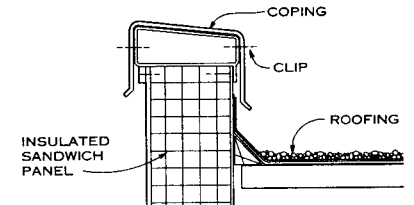
COPING
