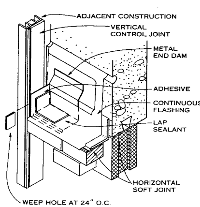
END DAM
