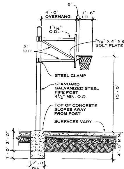
BASKETBALL STANDARDS
