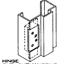
HINGE CUT-OUT W/REINF AND PLASTER GUARD
