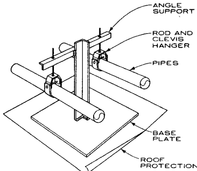
PIPE SUPPORT
