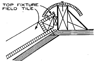
FLAT ROOF MEETS SLOPE TILES
