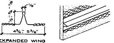
EXPANDED WING BASE SCREEDS
