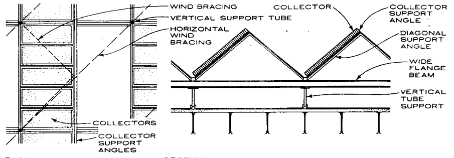
PLAN SECTION COLLECTOR SUPPORT
