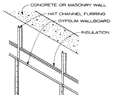
FURRING CHANNELS
