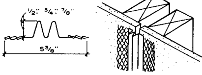
CONTROL JOINTS
