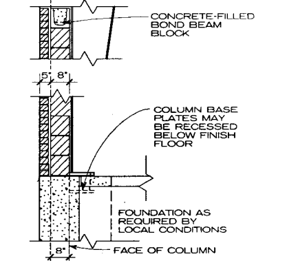
MASONRY AND BRICK VENEER WALL SECTION
