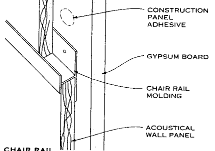
FOAM AND FIBERGLASS PANEL ATTACHMENT DETAILS
