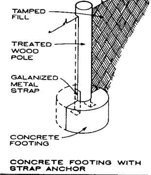
CONCRETE FOOTING WITH STRAP ANCHOR
