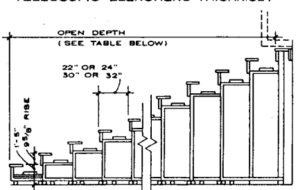
TELESCOPIC BLEACHERS (LOWRISE)
