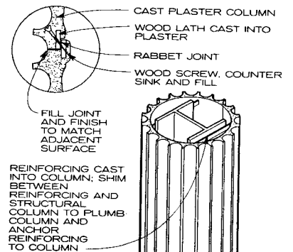
TWO-PIECE GLASS FIBER-REINFORCED GYPSUM COLUMN
