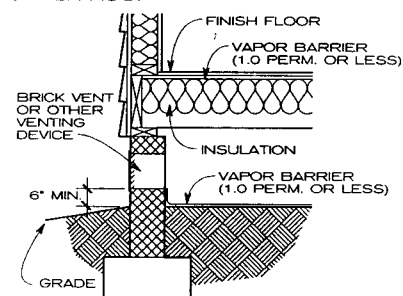
CRAWL SPACE
