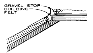
FLASHING OVER TILE AT FLAT ROOF
