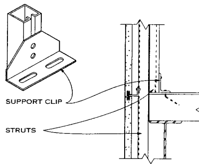
SHEAR WALL SUPPORT
