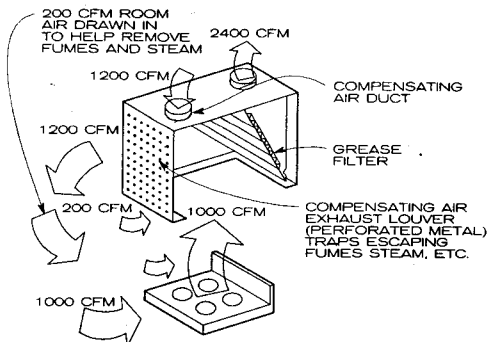
HOOD WITH 50% COMPENSATING AIR
