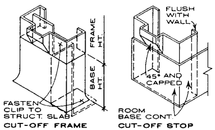
CUT-OFF FRAME CUT-OFF STOP HOSPITAL STOP
