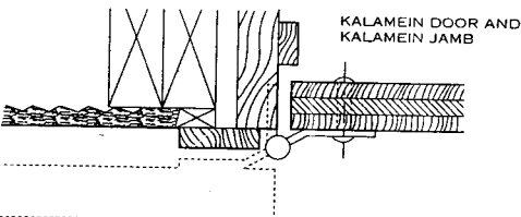
HALF-SURFACE TEMPLATE
