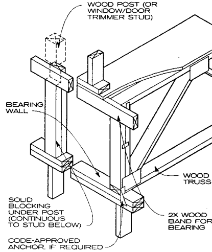
EXTERIOR WALL BEARING DETAIL
