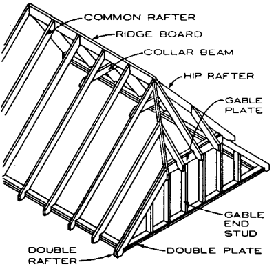
HIP GABLE ROOF
