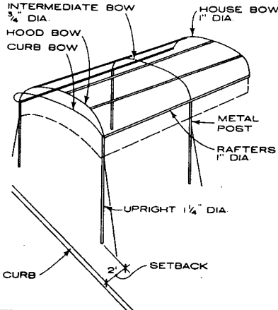
CANOPIES - LOW CURVED BOW SHOWN
