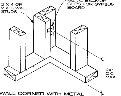
WALL CORNER WITH METAL GYPSUM BOARD CLIPS
