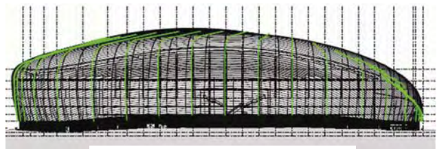
Figure 4: Overlay evaluation.
