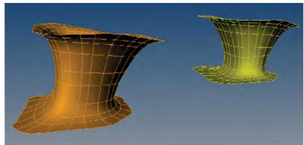
Performed Smoothing
