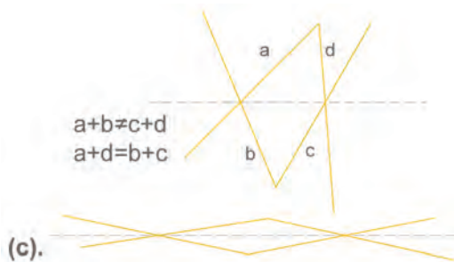
Figure 1: deployability conditions
