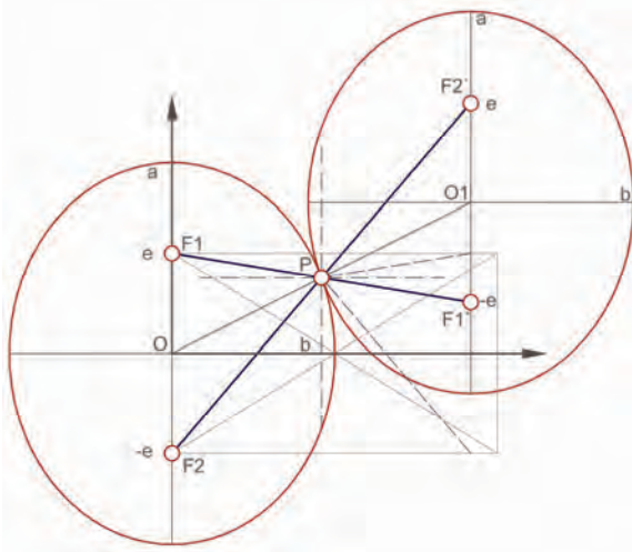
Figure 7: concept for a double-curved SLEs structure
