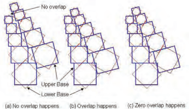
Figure 6: Geometric configurations with different overlap conditions
