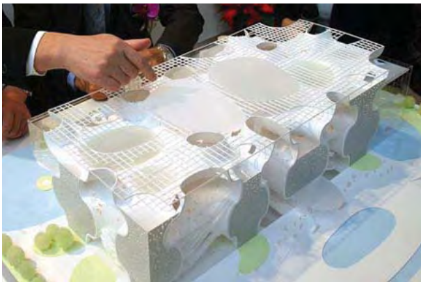
Competition Model
