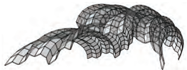
Figure 12: Thickened IFS-surface
