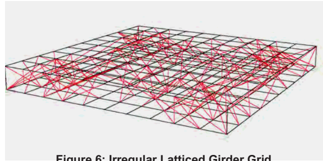
Figure 6: Irregular Latticed Girder Grid
