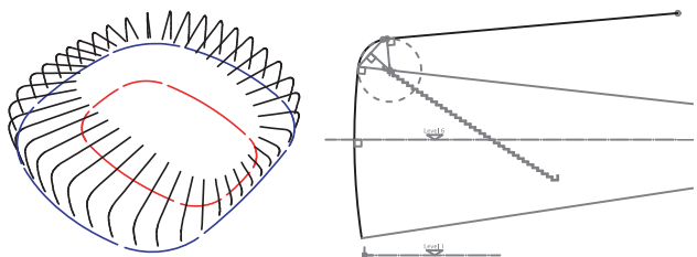
Figure 2: Geometric method.
