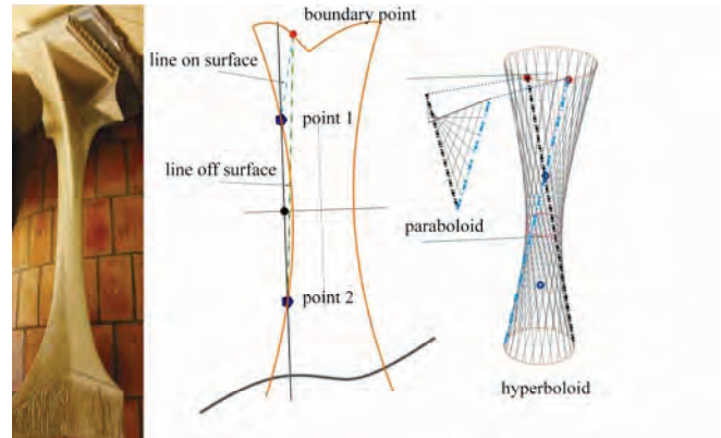
Figure 3: Soft stone prototype at 1:5 scale of one of the columns to show the geometry of the intersecting hyperboloid and paraboloids. There are two possible points of intersection on the surface for the lines of intersection between the hyperboloid and paraboloid, only one of which is ‘correct’ for each combination of variables controlling the surface shape.
