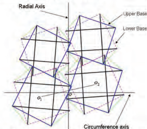
Figure 1: Flat configuration of a 4-unit cluster of a helical structure.
