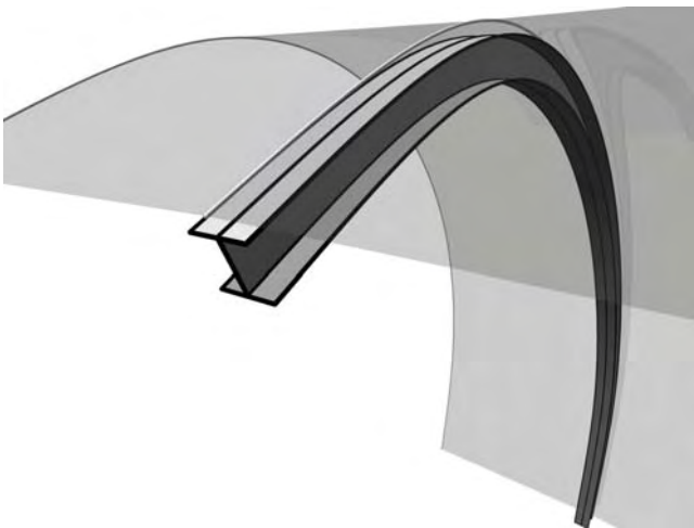
Figure 8: Positioning a curved I-beam with developable stem and developable horizontal bars along the edge curve of a conical model.
