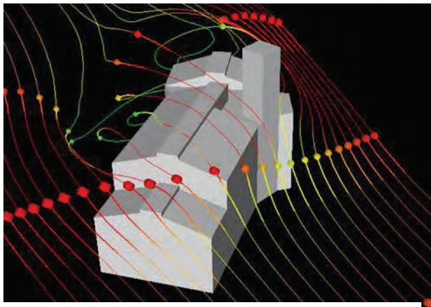
Figure 2: External CFD model
