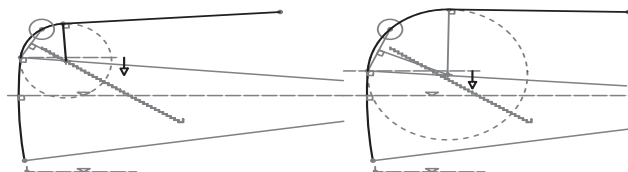
Figure 3: Sectional Curves.
