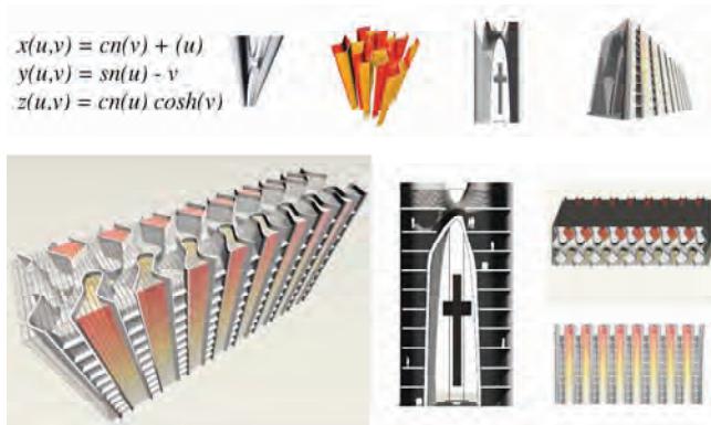
Figure 4: The Hybrid Cathedral with a surface from a gamma function mediating between congregational space and
