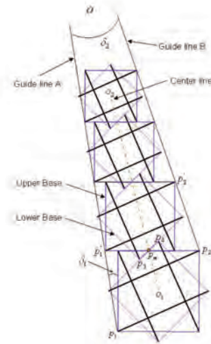
Figure 5 Geometric configuration of a tensegrity column along the radial axis
