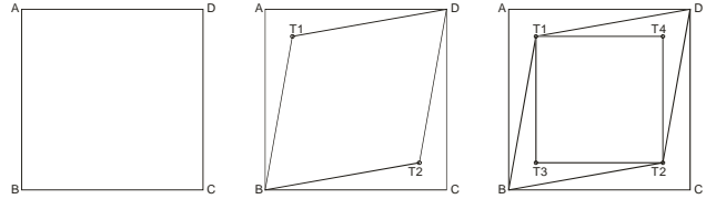
Figure 3: (Left) face:\{A, B, C, D\} ; (Middle) faceSet(3):\{\{face:\{A, B, T_1, D\}, face:\{B, T_2, D, T_1\}, face:\{C, D, T_2, B\}\}\} ; (Right) faceSet(5):\{\{face:\{A, B, T_1, D\}, face:\{B, T_2, T_3, T_1\}, face:\{T_2, T_4, T_1, T_3\}, face:\{D, T_1, T_4, T_3\}, face:\{C, D, T_2, B\}\}\}
