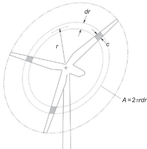
Figure 3.9 Equating blade element and momentum forces. The momentum thrust acting on annular area 2\pi r dr is equated to the thrust on the discrete blade elements (shaded) of combined area Ncd , where N is blade number.
