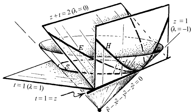
Fig. 18.9 Sections of the light cone t^2 - x^2 - y^2 - z^2 = 0 , by 3-planes (z+t) + \lambda(t-z) = 2 , through the 2-plane t = 1 = z . The coordinate y is suppressed, so dimensions appear reduced by 1. When \lambda > 0 the section S has a 2-sphere d\ell^2 metric, illustrated by the horizontal case \lambda = 1 . When \lambda = 0 we get the flat Euclidean d\ell^2 metric of the paraboloidal section E . When \lambda < 0 we get a hyperbolic d\ell^2 metric, illustrated by the vertical hyperbolic section H , in the case \lambda = -1 .
