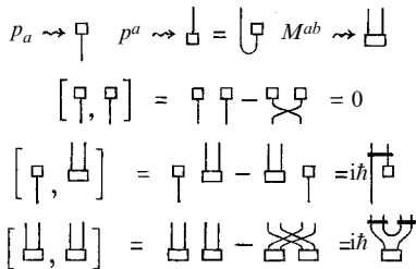
Fig. 22.18 Diagrammatic form of the relativistic 4-momentum and 6-angular momentum quantum commutators [p_a, p_b] = 0 , [p_a, M^{bc}] = i\hbar(g_a^b p^c - g_a^c p^b) , [M^{ab}, M^{cd}] = i\hbar(g^{bc} M^{ad} - g^{bd} M^{ac} + g^{ad} M^{bc} - g^{ac} M^{bd}) .
