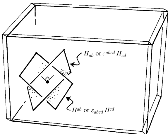
Fig. 19.2 In 4-space, a simple bivector H ( H^{ab} ) represents the same 2-plane element as its ‘dual’ 2-form H^\# ( \frac{1}{2}\epsilon_{abcd}H^{cd} ). But the index-lowered version of H , the simple 2-form H_{ab} , which is equivalent to its ‘dual’ bivector \frac{1}{2}\epsilon^{abcd}H_{cd} , represents the orthogonal complement 2-plane element (see Fig. 18.4). Hence it is the index raising/lowering in the Hodge dual that leads to the passage to the orthogonal complement.
