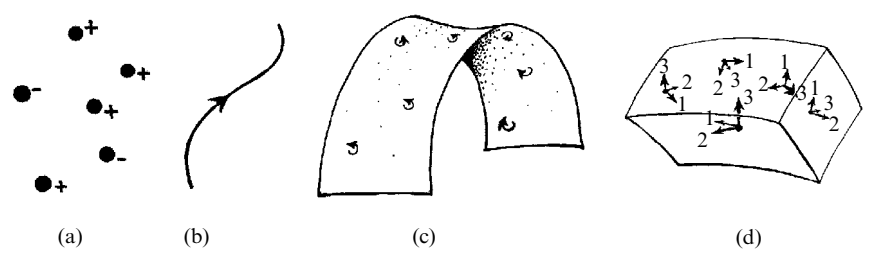
Fig. 12.14 Orientation. (a) A (multi-component) 0-manifold is a set of discrete points; the orientation simply assigns a ‘positive’ (+) or ‘negative’ (–) value to each. (b) For a 1-manifold, or curve, the orientation provides a ‘direction’ along the curve; represented in a diagram by the placement of an arrow on it. (c) For a 2-manifold, the orientation can be indicated by a tiny circular arc with an arrow on it, indicating the ‘positive’ direction of rotation of a tangent vector. (d) For a 3-manifold the orientation specifies which triads of independent vectors at a point are to be regarded as ‘right-handed’ (cf. Fig. 11.1).
