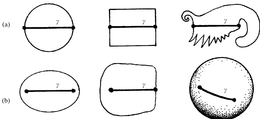
Fig. 9.15 The excision theorem tells us that the notion of a hyperfunction is independent of the choice of open region \mathcal{R} , so long as \mathcal{R} contains the given curve \gamma . (a) The region \mathcal{R} - \bar{\gamma} may consist of two separate pieces (so we get two distinct holomorphic functions f and g , as in Fig. 9.14) or (b) the region \mathcal{R} - \bar{\gamma} may be a single connected piece, in which case f and g are simply two parts of the same holomorphic function.
