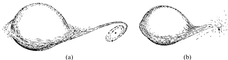
Fig. 27.12 Double star systems, one member of which is a (tiny) black hole. (a) Matter dragged from the larger star by the black hole forms an accretion disc around it, gradually spiralling in and becoming heated until X-rays are emitted before the material actually enters the hole. (b) In some cases there is no accretion disc and the material simply falls ‘straight in’. If the attracting compact object were to have a ponderable surface, in-falling material would heat it up, but no glow is seen, confirming the presence of a black hole.
