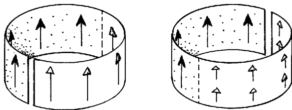
Fig. 15.18 Consider a part \mathcal{B}_p , of \mathcal{B} (of Fig. 15.16) that stands above a ‘trivial’ region S^1 - p of S^1 , and similarly for \mathcal{B}_q , just as in Fig. 15.5a. Take ‘horizontal’ in each patch to mean horizontal in the ordinary sense. In the gluing, however, there is a relative stretching by a factor of 2 between one region of gluing and the other (illustrated in the right-hand patching). This provides the connection illustrated in Fig. 15.16.
