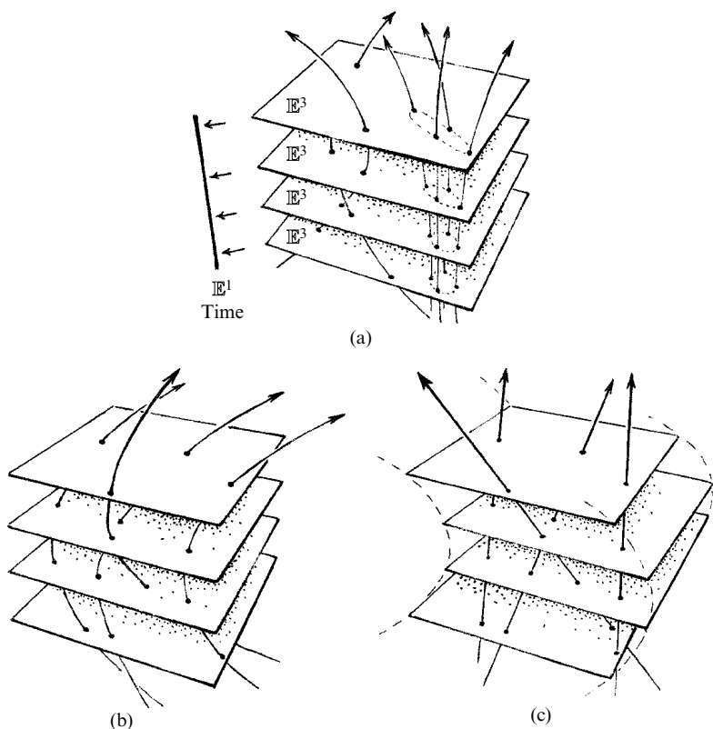
Fig. 17.7 (a) Newton–Cartan spacetime \mathcal{N} , like the particular Galilean case \mathcal{G} , is a bundle with base-space \mathbb{E}^1 and fibre \mathbb{E}^3 . Its structure is provided by the family of motions, ‘inertial’ in Einstein’s sense, of free fall under gravity. (b) The special case of a Newtonian gravitational field constant over all space. (c) Its structure is completely equivalent to that of \mathcal{G} , as can be seen by ‘sliding’ the \mathbb{E}^3 fibres horizontally until the world lines of free fall are all straight.
