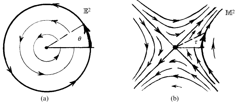
Fig. 30.5 Periodicity in imaginary time, illustrated by Minkowski 2-space \mathbb{M}^2 , complexified to \mathbb{C}\mathbb{M}^2 = \mathbb{C}\mathbb{E}^2 . (a) The Euclidean plane \mathbb{E}^2 is one real section of the complex space \mathbb{C}\mathbb{M}^2 . The Killing vector \partial/\partial\theta generates rotations in \mathbb{E}^2 , where we take polar coordinates (r, \theta) . Any function that is single-valued on \mathbb{E}^2 must be periodic in \theta with period 2\pi . (b) In the Lorentzian real section \mathbb{M}^2 of \mathbb{C}\mathbb{M}^2 , the ‘Rindler’ (uniform-acceleration) time coordinate is \tau = i\theta (an analogue of the Schwarzschild time that is natural for a black hole), and a function that is analytic at the origin O must have an imaginary period in \tau , with period 2\pi i . (Killing vector \kappa = \partial/\partial\tau = -i\partial/\partial\theta .)
