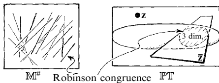
Fig. 33.14 We can obtain a ‘real’ picture of a non-null twistor Z^\alpha by first passing to its complex conjugate \bar{Z}_\alpha , thus defining a complex projective plane in \mathbb{P}\mathbb{T} . This plane is fixed by its intersection with \mathbb{P}\mathbb{N} , which is a 3-real-dimensional locus. This locus defines a 3-parameter family of light rays in \mathbb{M}^\# called a Robinson congruence.
