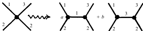
Fig. 32.12 All the nodes of spin networks in loop-variable theory are 4-valent (or more) and need extra ‘intertwining’ information. This can be encoded in ‘X’-type vertex being expressed as a linear combination of ‘H’-type 3-edge vertex pairs. The specific coefficients remove this ambiguity.
