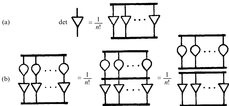
Fig. 13.8 (a) Diagrammatic notation for \det (T^a_b) = \det T = |T| . (b) Diagrammatic proof that \det (ST) = \det S \det T . The antisymmetrizing bar can be inserted in the middle term because there is already antisymmetry in the index lines that it crosses. See Figs. 12.17, 12.18.
