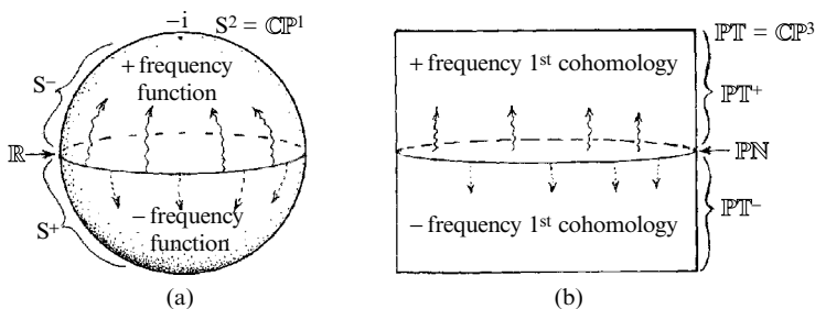
Fig. 33.22 An analogy between the Riemann sphere S^2 (= \mathbb{C}P^1) and projective twistor space \mathbb{P}T (= \mathbb{C}P^3) . (a) A complex function (i.e. a 0th cohomology element), defined on the real axis \mathbb{R} of S^2 , splits into its positive frequency part, extending holomorphically into what is here depicted as the northern hemisphere S^- , and its negative frequency part, extending into the southern hemisphere S^+ . (The Riemann sphere is here drawn so that \mathbb{R} is its equator, but so that -i is at the north pole and i at the south pole; compare Figs. 8.7 and 9.10, §9.5.) (b) A 1st cohomology element, defined on \mathbb{P}N (and representing a massless field) splits into its positive frequency part, extending holomorphically into the top half \mathbb{P}T^+ of projective twistor space, and its negative frequency part, extending into the bottom half \mathbb{P}T^- .
