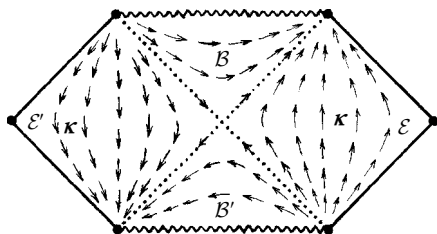
Fig. 30.9 The Killing vector \kappa is timelike in the two external regions \mathcal{E} and \mathcal{E}' , but spacelike in the internal regions \mathcal{B} and \mathcal{B}' . Comparing \kappa in \mathcal{E} and in \mathcal{E}' , we find that it reverses time-orientation, so that the concept of conserved energy density T_{ab}\kappa^a reverses its sign.
