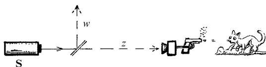
Fig. 29.7 Schrödinger’s cat (modified from original). A photon source S emits a single photon aimed at a beam-splitter, whereupon the photon’s state splits into a superposition of 2 parts. In one of these, the photon encounters a detector, triggering a murderous weapon that kills the cat; in the other, the photon escapes and the cat lives. U -evolution results in a superposition of a dead and a live cat.
