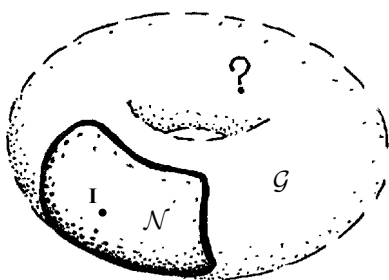
Fig. 13.12 The Lie algebra for a (faithful) representation of a Lie group \mathcal{G} (basically, knowledge of the structure constants \gamma_{\alpha\beta}^{\chi} ) determines the local structure of \mathcal{G} , i.e. it fixes the structure of \mathcal{G} within some (sufficiently small) open region \mathcal{N} surrounding the identity element \mathbf{I} , but it does not tell us about the global nature of \mathcal{G} .
