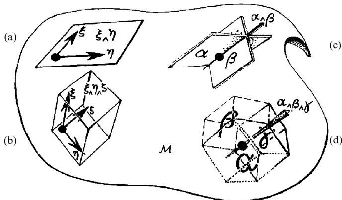
Fig. 12.10 (a) A 2-plane element at a point of \mathcal{M} , being spanned by independent vectors \xi , \eta , is described by the bivector \xi \wedge \eta . (b) Similarly, a 3-plane element spanned by \xi , \eta , \zeta is described by \xi \wedge \eta \wedge \zeta . (c) Dually, an (n-2) -plane element, the intersection of two (n-1) -plane elements specified by 1-forms \alpha , \beta , is described by \alpha \wedge \beta . (d) The (n-3) -plane element of intersection of the three (n-1) -plane elements specified by \alpha , \beta , \gamma , is described by \alpha \wedge \beta \wedge \gamma .
