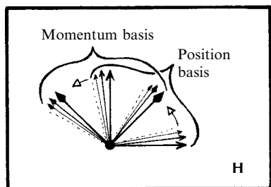
Fig. 22.3 Passing from a position to a momentum representation is just changing the basis in Hilbert space H (although, technically, neither momentum nor position states, being non-normalizable, actually belong to H ).
