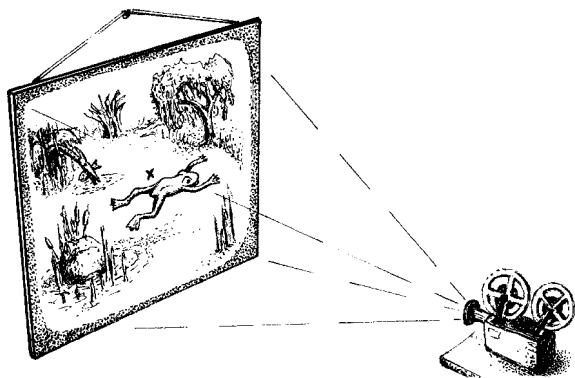
Fig. 17.1 Is physical motion like that perceived on a cinema screen? A particular point on the screen (here marked ‘×’) retains its identity no matter what movement is projected upon it.
