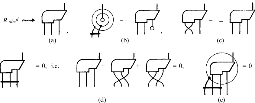
Fig. 14.7 (a) A convenient diagrammatic notation for the curvature tensor R_{abcd} . (b) The Ricci identity (\nabla_a \nabla_b - \nabla_b \nabla_a)\xi^d = R_{abc}{}^d \xi^c . (c) The antisymmetry R_{bac}{}^d = -R_{abc}{}^d . (d) The Bianchi symmetry R_{[abc]}{}^d = 0 , which reduces to R_{abc}{}^d + R_{bca}{}^d + R_{cab}{}^d = 0 . (e) The Bianchi identity \nabla_{[a} R_{bc]d}{}^e = 0 .
