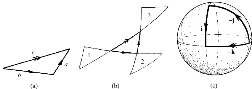
Fig. 11.4 (a) Translations in the Euclidean plane represented by oriented line segments. The double-arranged segment represents the composition of the other two, by the triangle law. (b) For rotations in Euclidean 3-space, the segments are now great-circle arcs drawn on the unit sphere, each representing a rotation through twice the angle measured by the arc (about an axis perpendicular to its plane). To see why this works, reflect the triangle made by the arcs, in each vertex in turn. The first rotation takes triangle 1 into triangle 2, the second takes triangle 2 into triangle 3, and the composition takes triangle 1 into triangle 3. (c) The quaternionic relation \mathbf{ij} = \mathbf{k} (in the form \mathbf{i}(-\mathbf{j}) = -\mathbf{k} ), as a special case. The rotations are each through \pi , but represented by the half-angle \frac{\pi}{2} .
