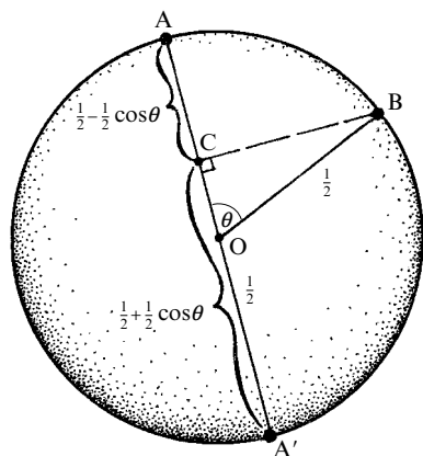
Fig. 22.11 Suppose that the initial state of a 2-state system (like that of Fig. 22.10) is represented by the point B on the Riemann sphere and we wish to perform a YES/NO measurement corresponding to some other point on the sphere, where YES would find the state at A and NO would find it at the point A', antipodal to A. Taking the sphere to have radius \frac{1}{2} , and projecting B orthogonally to C on the axis A'A, we find that the probability of YES is the length A'C, which is \frac{1}{2}(1 + \cos \theta) , and the probability of NO is the length CA, which is \frac{1}{2}(1 - \cos \theta) , where \theta is the angle between OB and OA, the sphere's centre being O.
