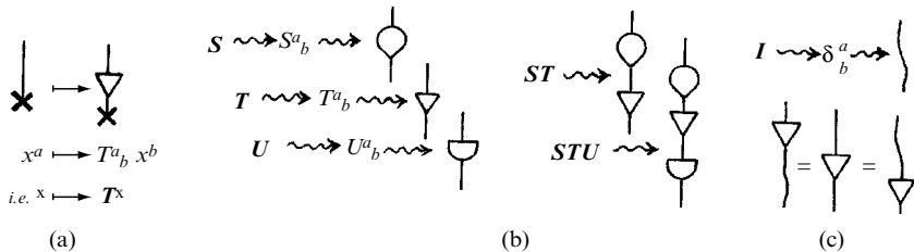
Fig. 13.6 (a) The linear transformation x^a \mapsto T^a_b x^b , or written without indices as x \mapsto T^x (or read with the indices as abstract, as in §12.8), in diagrammatic form. (b) Diagrams for linear transformations S , T , U , and their products ST and STU . In a successive product, we string them in a line downwards. (c) The Kronecker delta \delta^a_b , or identity transformation I , is depicted as a ‘disembodied’ line, so relations T^a_b \delta^b_c = T^a_c = \delta^a_b T^b_c become automatic in the notation (see also Fig. 12.17).
