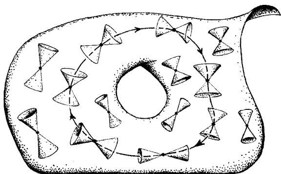
Fig. 17.18 The causality structure of \mathcal{E} is determined by g (as with \mathbb{M} , see Fig. 17.16), so extreme unphysical situations with ‘closed timelike curves’ might hypothetically arise, allowing future-directed signals to return from the past.
