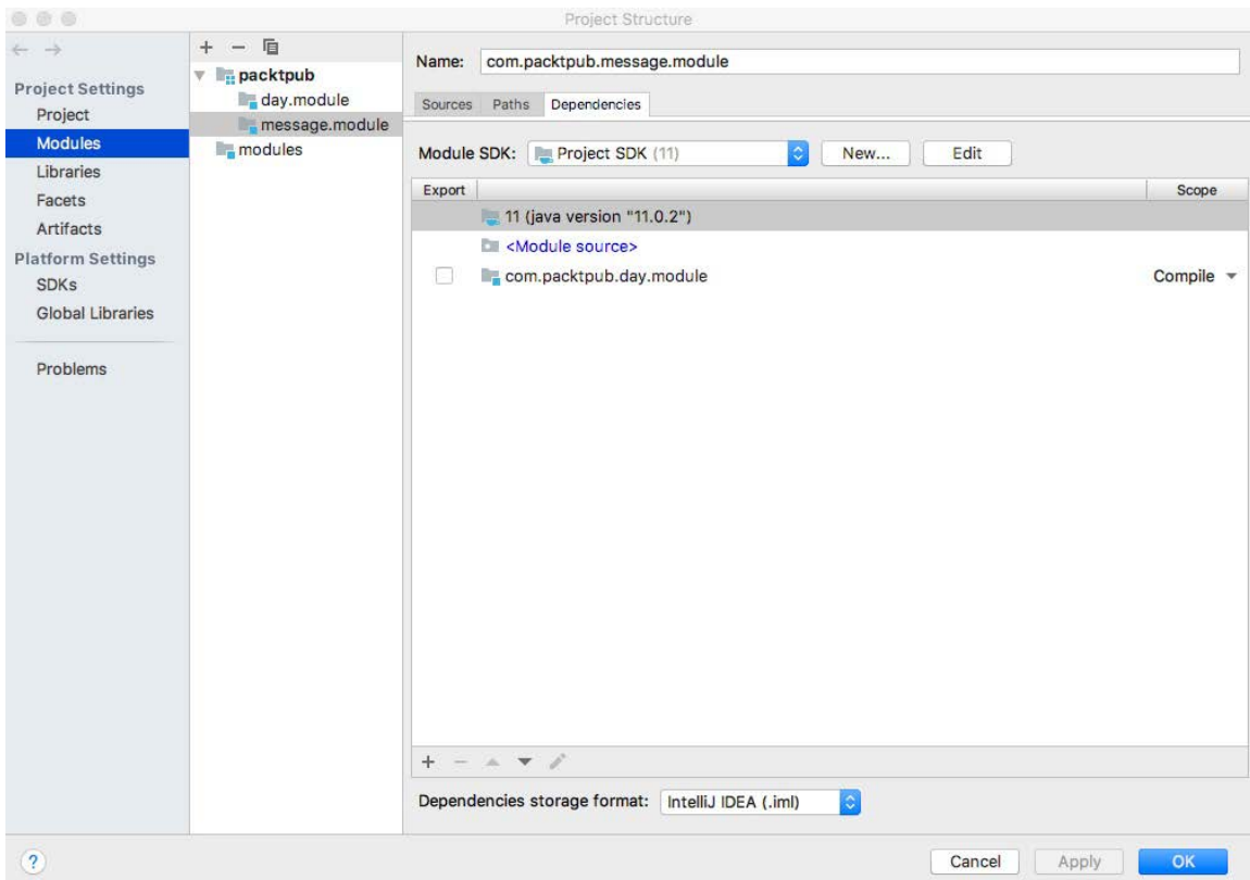
Figure 6.11: The IntelliJ project structure dialog showing the new module dependency on the com.packtpub.day.module module
