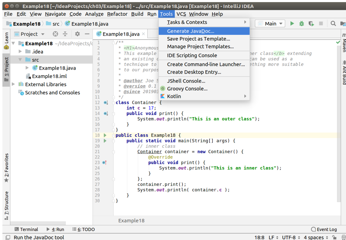
Figure 3.9: Generating JavaDoc
