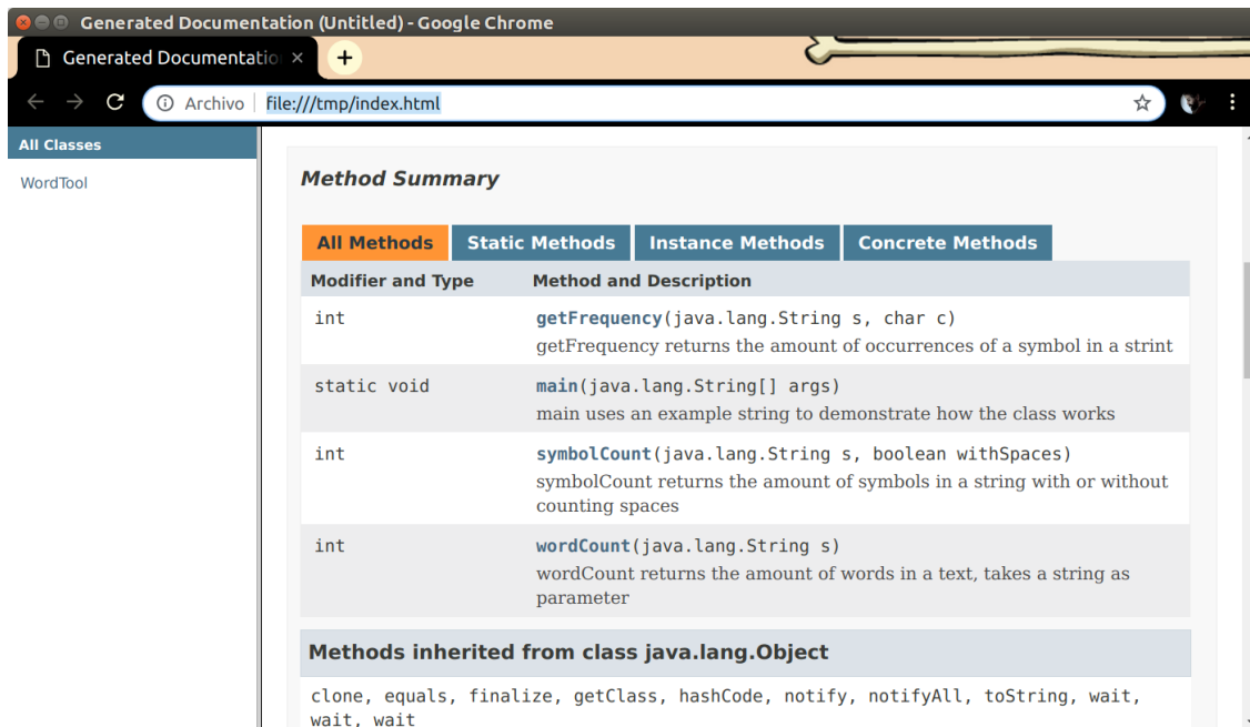
Figure 3.12: Documentation Site
