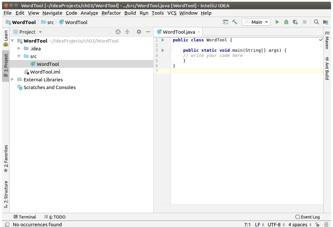
Figure 3.8: WordTool
