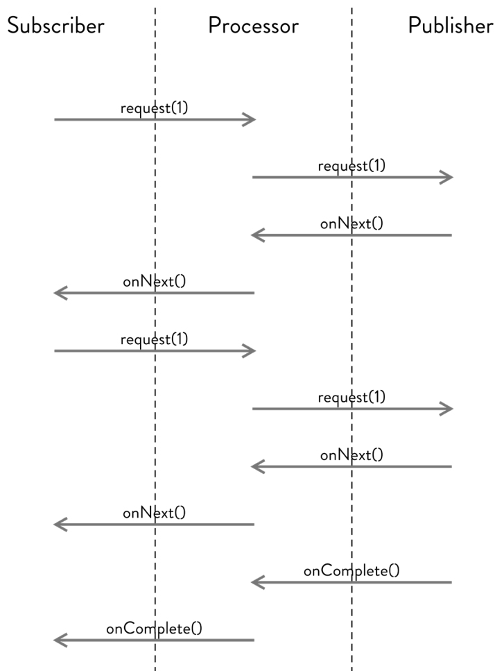
Figure 17.2: Communication between the Subscriber, the Processor, and the Publisher
