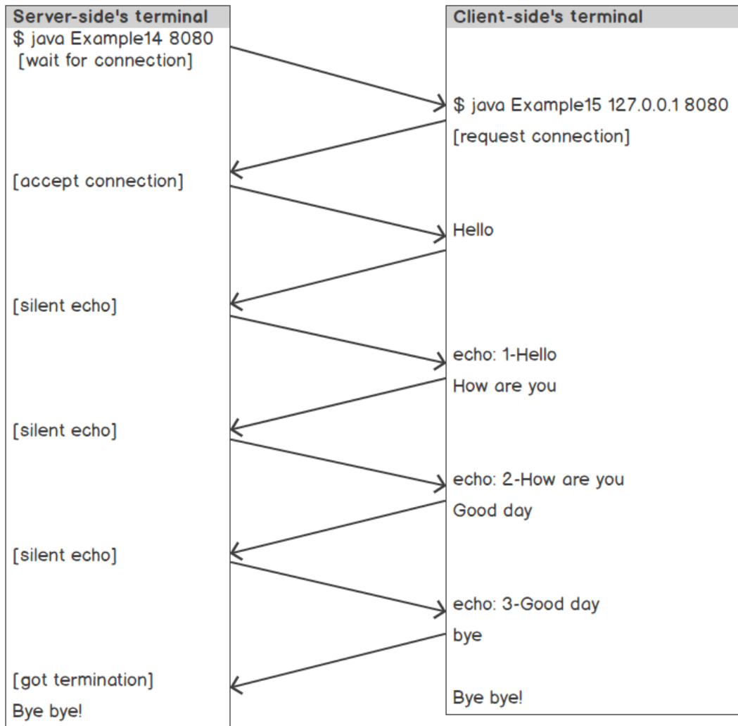
Figure 8.1: The interaction between the client and the server.
