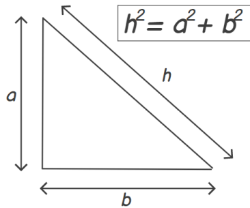
Figure 1.11: A right angled triangle with sides as a and b and h as the hypotenuse
