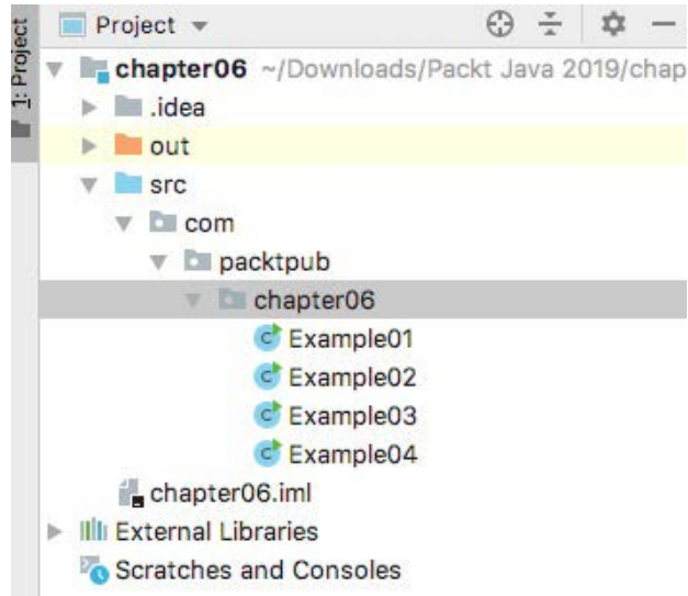
Figure 6.1: IntelliJ's Project pane can show the individual folders that make up a Java package
