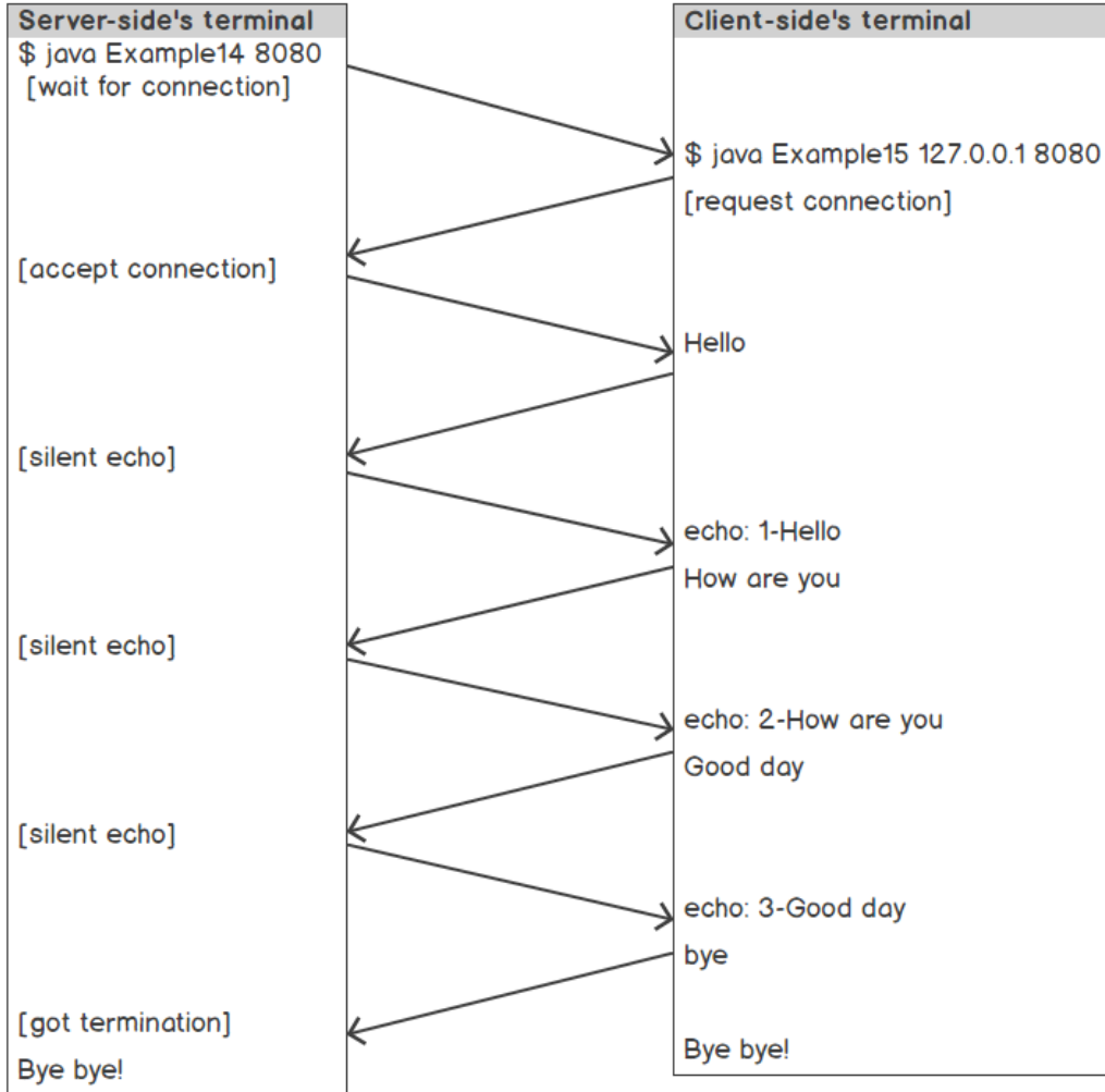
Figure 8:2: Interaction between server and client
