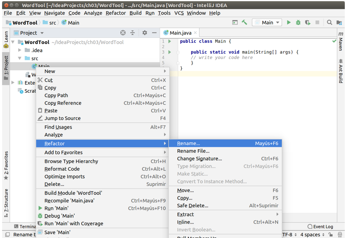
Figure 3.6: Refactoring the Java class
