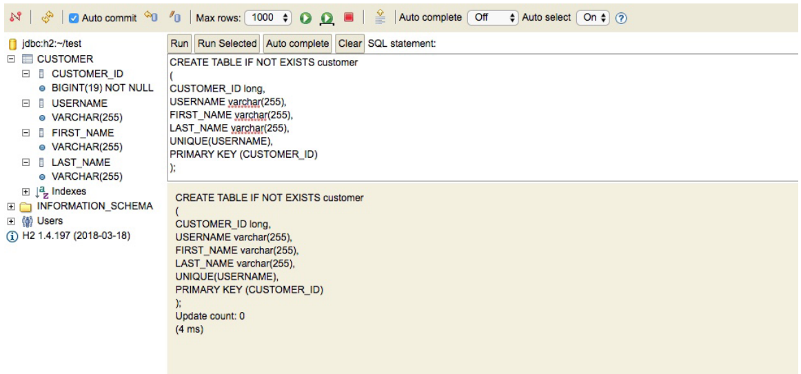
Figure 7.4: The H2 database console after creating a table
