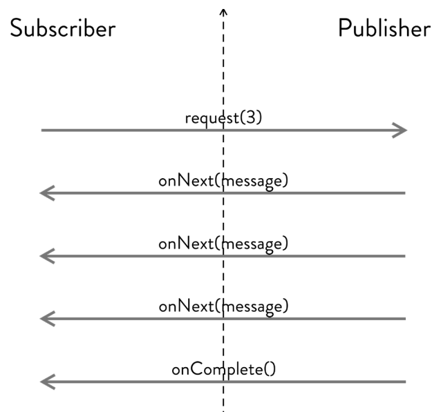
Figure 17.1: Communication between the Subscriber and the Publisher
