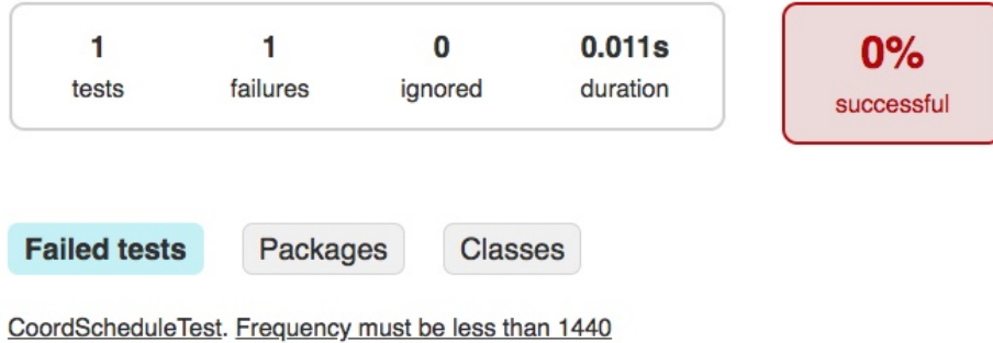
Figure 18.2: The test report as displayed in the browser
