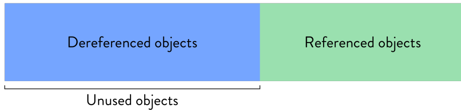
Figure 21.1: An illustration of a healthy heap
