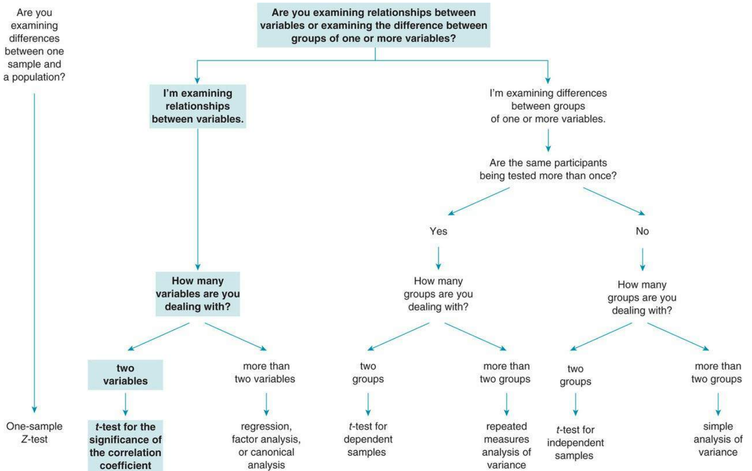
Figure 15.1 Determining That a t -Test for the Correlation Coefficient is the Correct Test Statistic
