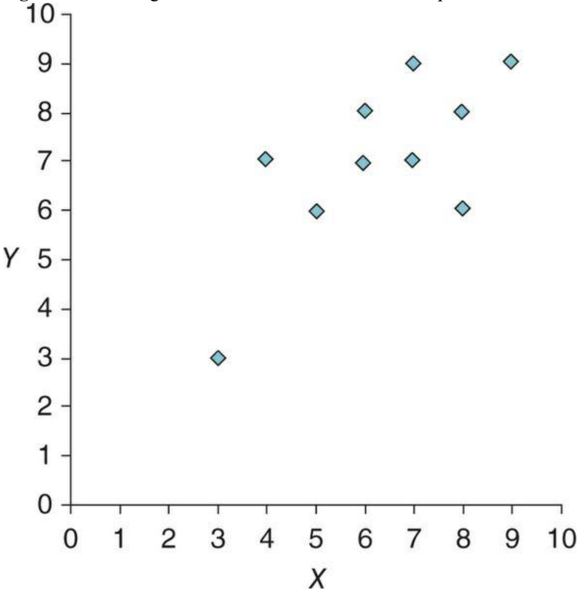
Figure 5.3 A Strong, but Not Perfect, Direct Relationship
