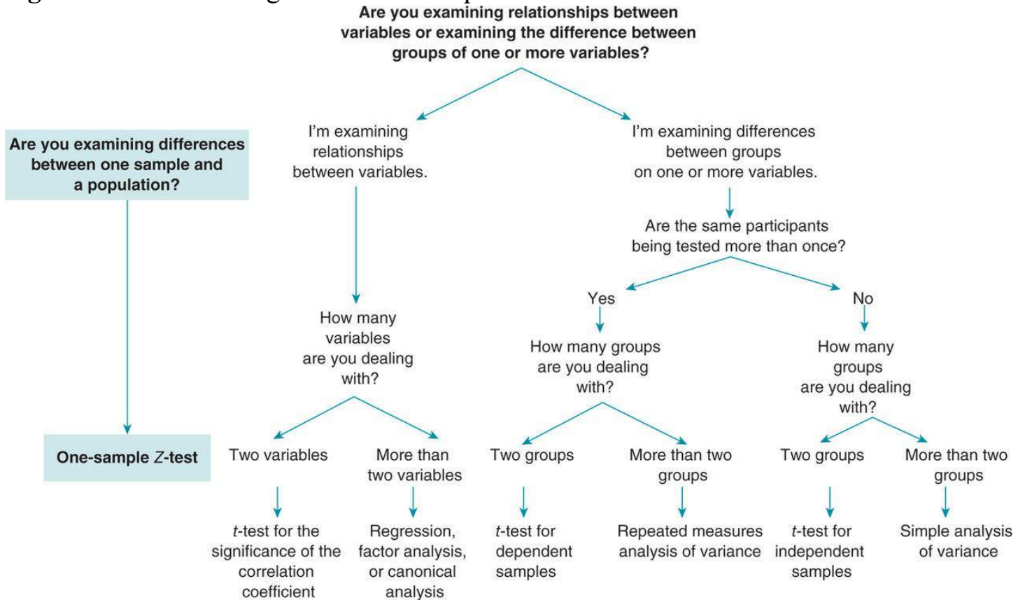
Figure 10.1 Determining That a One-Sample Z-Test is the Correct Statistic
