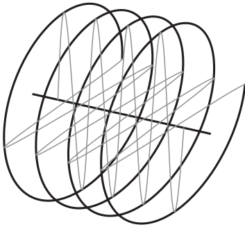
Figure 7.30 A depiction of circularly polarized light as a helix on a three-dimensional plot.
