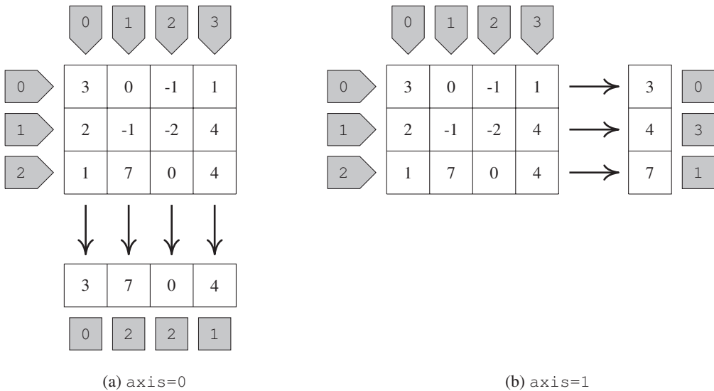
Figure 6.2 (a) a.argmax(axis=0) giving the maximum values and a.argmax(axis=0) giving the indexes of the maximum values of each column in array a (that is, maintaining the row dimension) and (b) The same for axis=1 : maximum values along each row.
