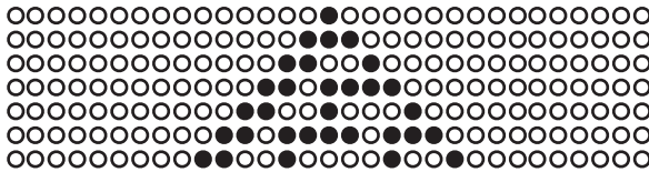
Figure 4.1 Rule 30 of Wolfram’s one-dimensional two-state cellular automata and the first seven generations.
