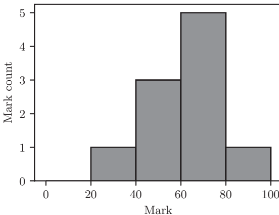
Figure 6.5 An example histogram.
