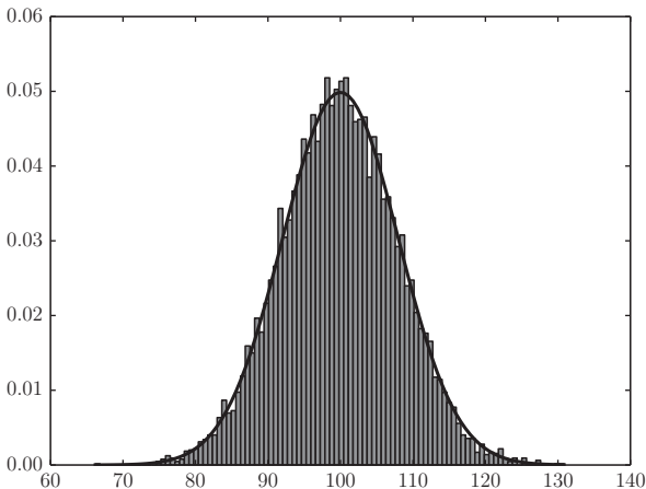
Figure 6.12 Histogram of 10 000 random samples from the normal distribution provided by np.random.normal .
