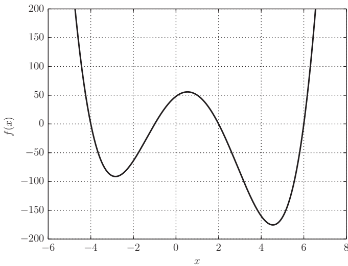
Figure 8.21 The polynomial f(x) = x^4 - 3x^3 - 24x^2 + 28x + 48 .
