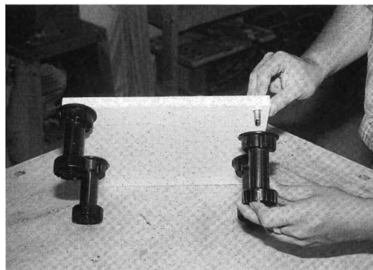
Fig. 6-4 Adjustable legs are secured with special screws through the base board.
