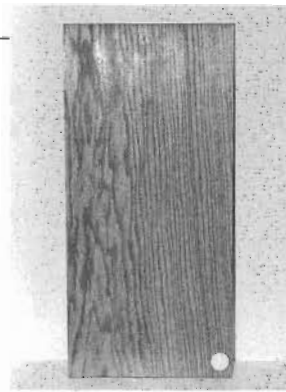
Fig. 1-8 A cabinet door made from 1/16" veneer-covered particle core board with wood veneer edge tape
