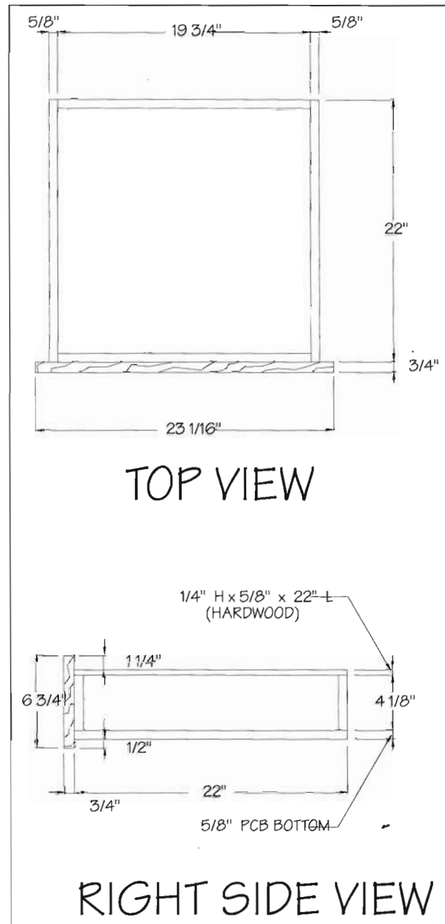
Fig. 9-13 Drawer dimensions for a 24" base cabinet designed in the drawer-over-door style.
