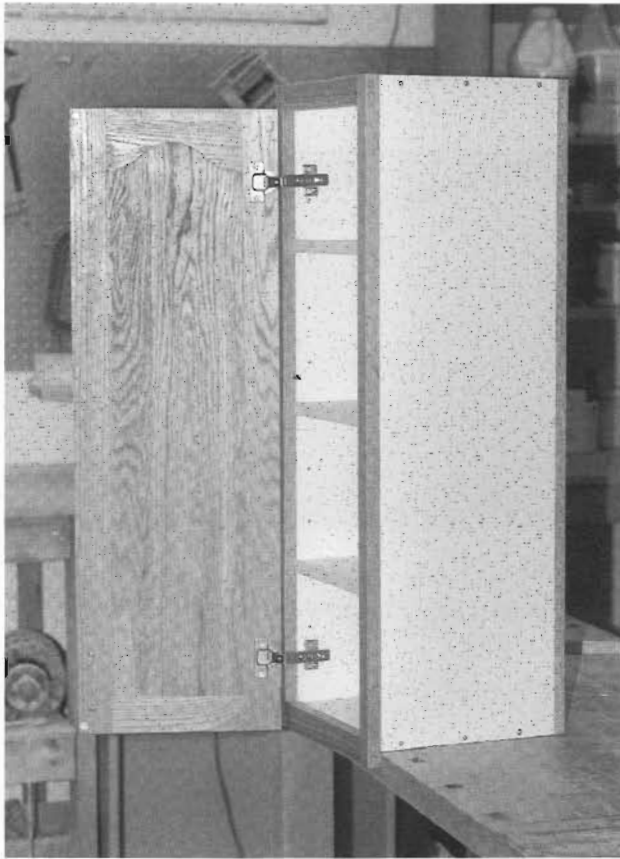
Fig. 4-3 Side view of an upper cabinet box (carcass)
