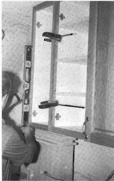
Fig. 17-6 Installing upper cabinets with a shop-made support box
