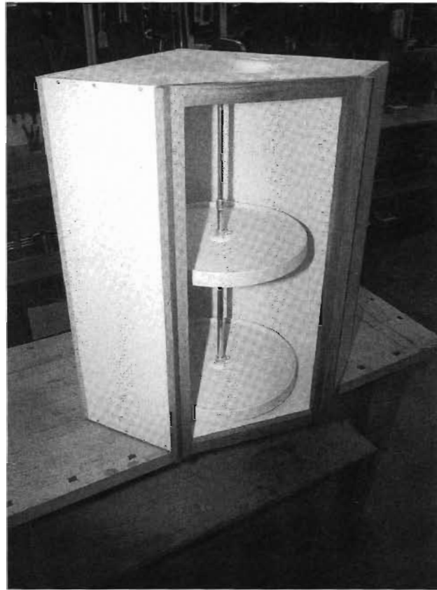
Fig. 5-12 The upper corner cabinet looks complicated to build but it is actually easy to construct.
