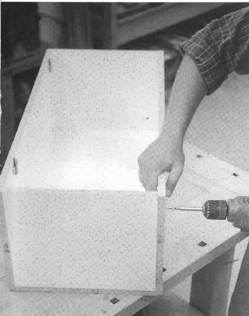
Fig. 1-20 5/8" melamine PCB butt joined with 2" particle core board screws
