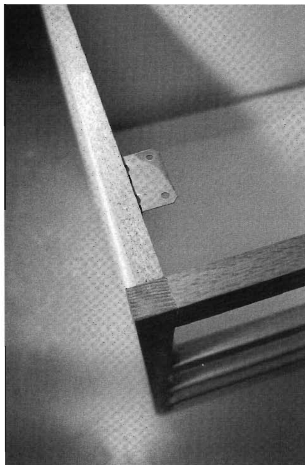
Fig. 6-3 Metal angle clips secure the countertop to the base.
