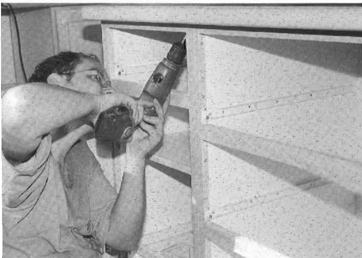
Fig. 17-5 The countertop is secured with \frac{5}{8} " screws through right-angle brackets.
