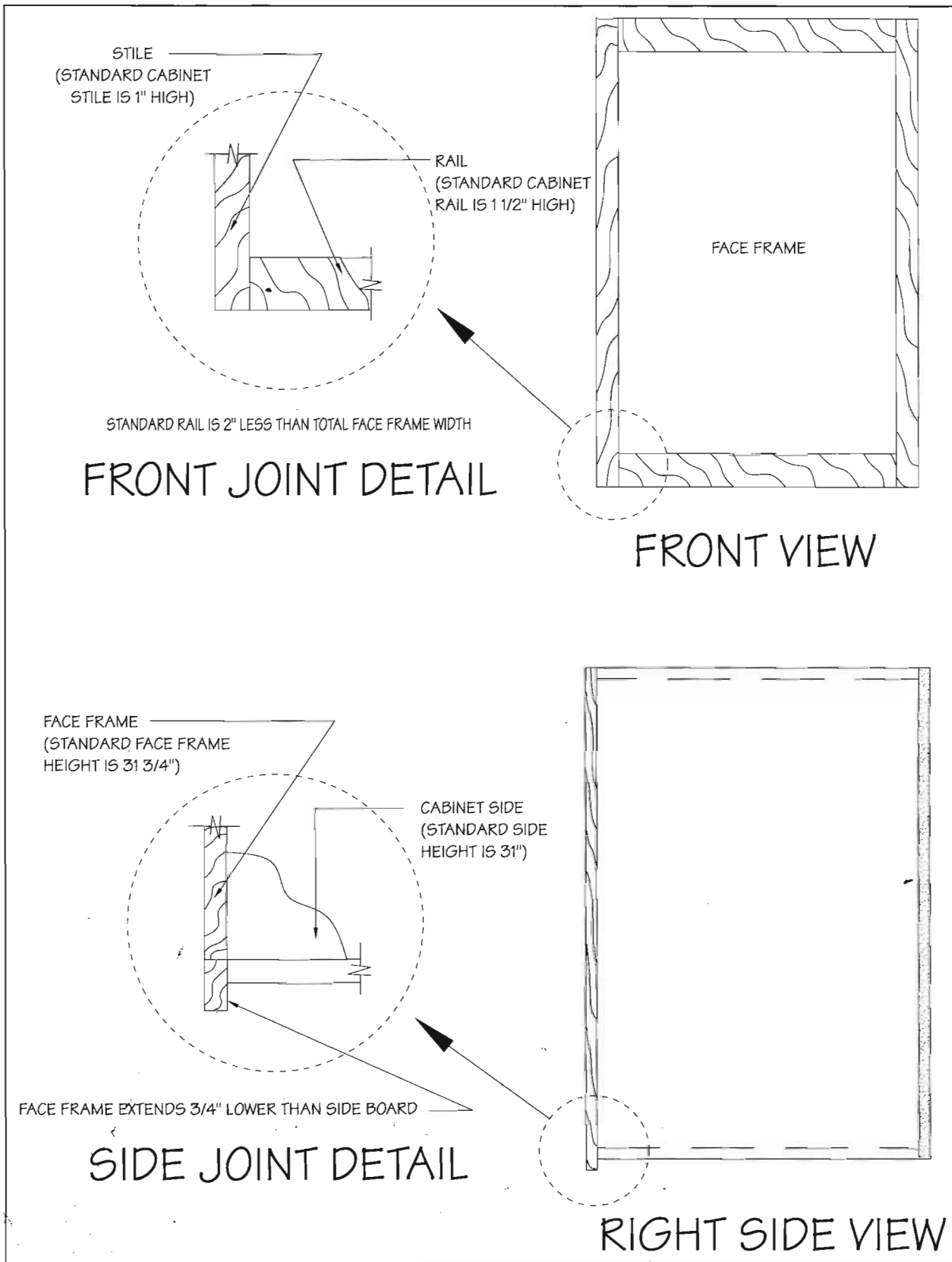
Fig. 4-8 Standard face frame details for both upper and lower cabinets
