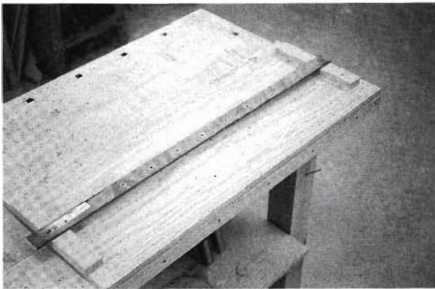
Fig. 5-4 Shelf-pin holes can be drilled with a homemade jig.
