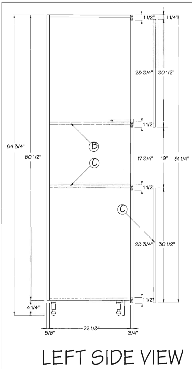
Fig. 7-2 This cabinet is a combination base and upper cabinet with a fixed shelf compartment for the microwave.
