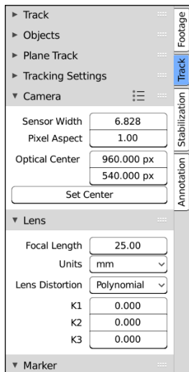
FIGURE 19-10: Use the Camera and Lens panels in the Track tab of the Movie Clip Editor's Sidebar to set values that match the device used to capture your video footage.
