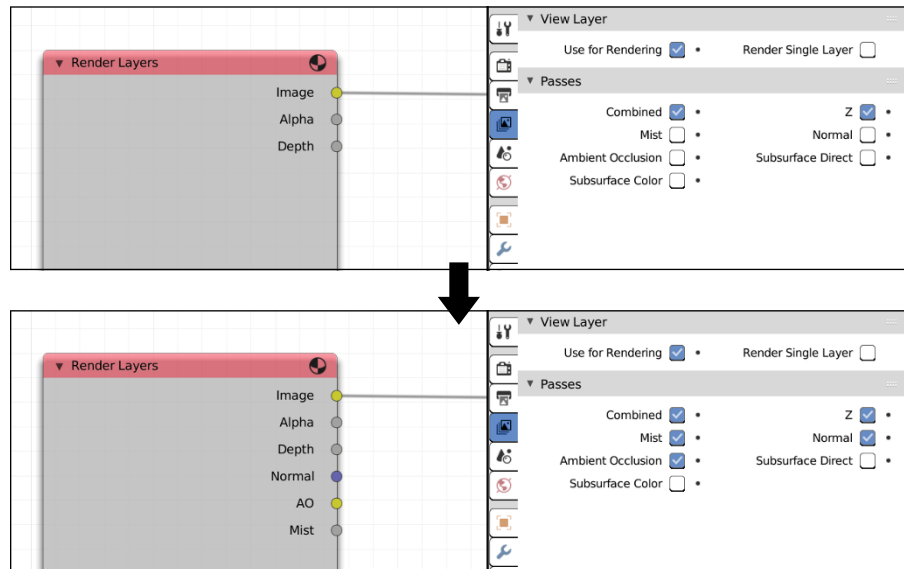
FIGURE 18-6: Enabling passes adds corresponding output sockets on your view layer's node in the Compositor.
