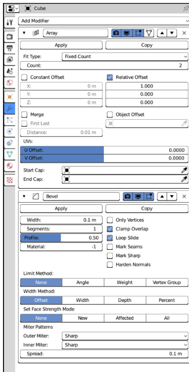
FIGURE 5-16: The Array and Bevel modifiers in Modifier Properties.
