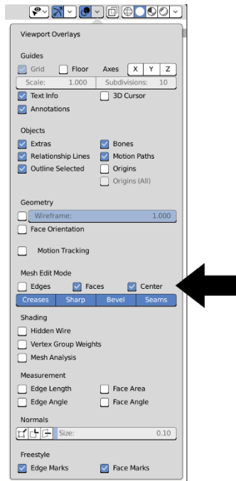
FIGURE 4-5: Use the Viewport Overlays roll-out menu to enable face centers so it's easier to tell what selection mode you're using.
