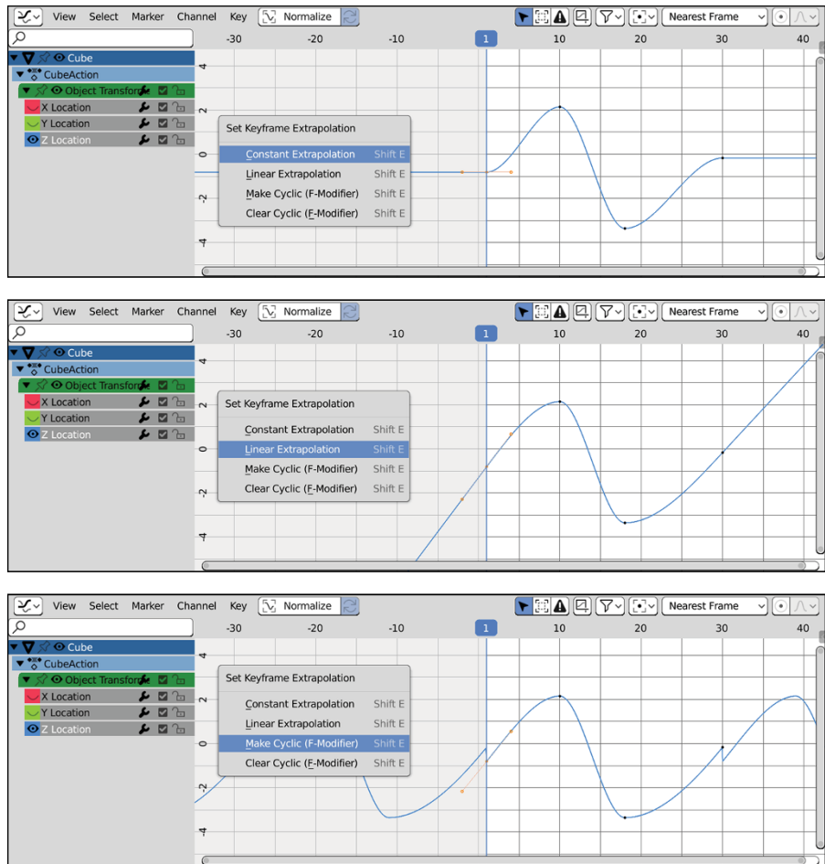
FIGURE 11-8: The four extrapolation modes you can have on f-curves.
