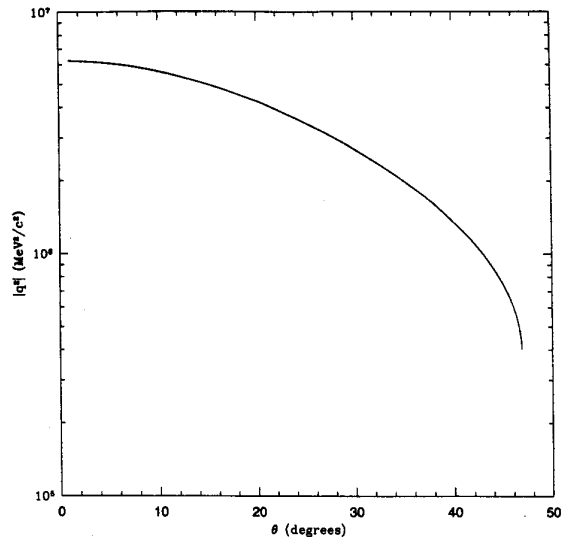
Fig.11 Plot of |q^3| as a function of outgoing laboratory angle of the \Sigma^0 for an incident electron energy of 4.0 GeV.
