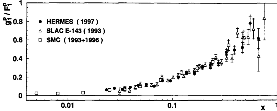
Figure 1. The structure function ratio g_1^p/F_1^p of the proton as a function of x from HERMES 4 is compared with recent results for g_1^p/F_1^p measured at SLAC (E143) 5 and A 1 at CERN (SMC) 6 . The inner error bars show the statistical uncertainties and the outer ones the quadratic sum of the statistical and total systematic uncertainties.
