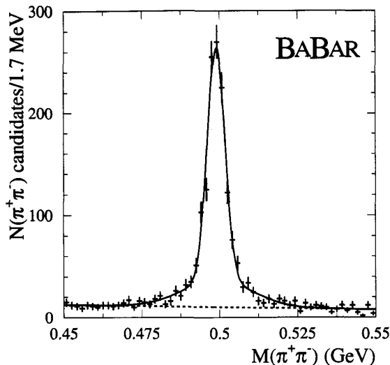
Figure 7. Oppositely charged pions pairs invariant mass distribution
