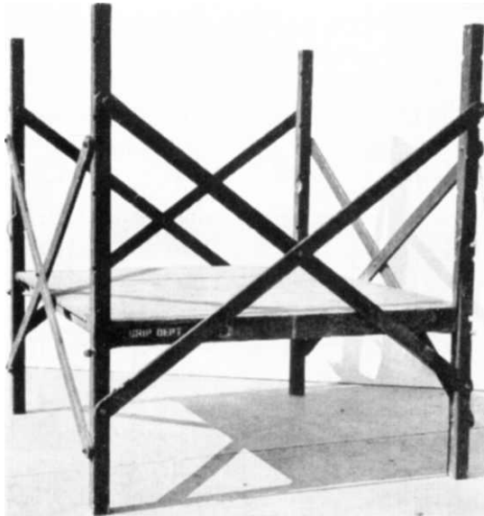
Fig. 7 Adjustable Platform. Low Position
