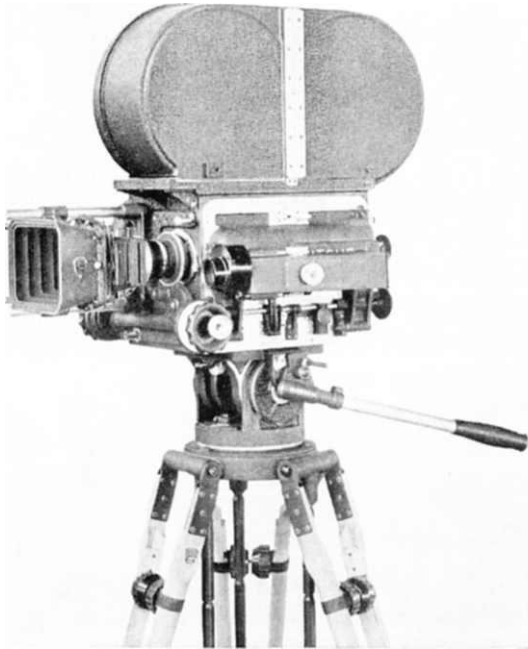
Fig. 1 Mitchell "BNC" 35 mm Studio Camera. (Merriman Photo.)
