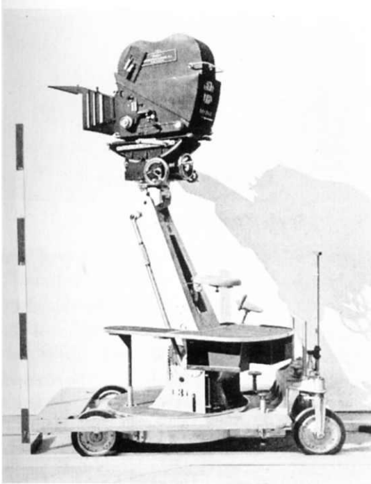
Fig. 4 Camera Dolly with Blimp in High Position
