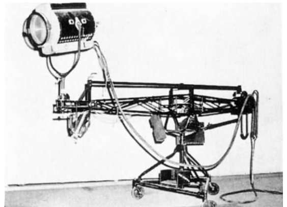
Fig. 64 Swinging Keylight
