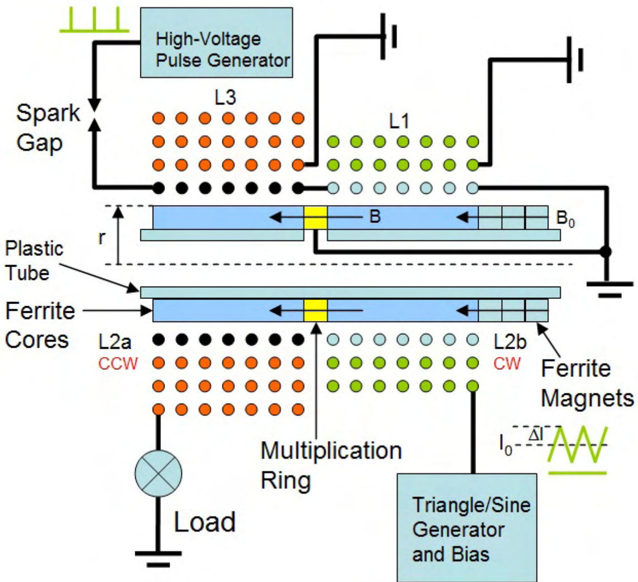
Fig.10 Cross-section of the Michael Meyer-style energy device. Some of the actual implementation details may differ from the arrangement shown above, but that will not alter the operation of device. This diagram is not to scale.
