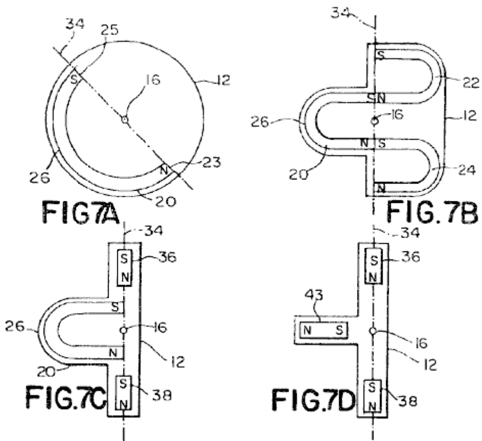
Fig.7A is a schematic plan view of a rotor used in the fourth preferred embodiment and in an eighth preferred embodiment of the motor;
