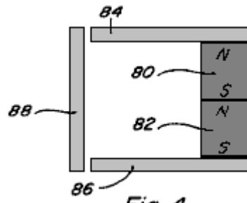
Fig.4 is a side view of two magnetic members arranged in series between pole pieces;
