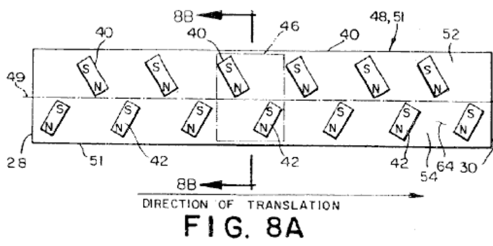
Fig.8A is a schematic plan view of a stator used in the fourth, fifth, eighth and ninth preferred embodiments of the motor;
