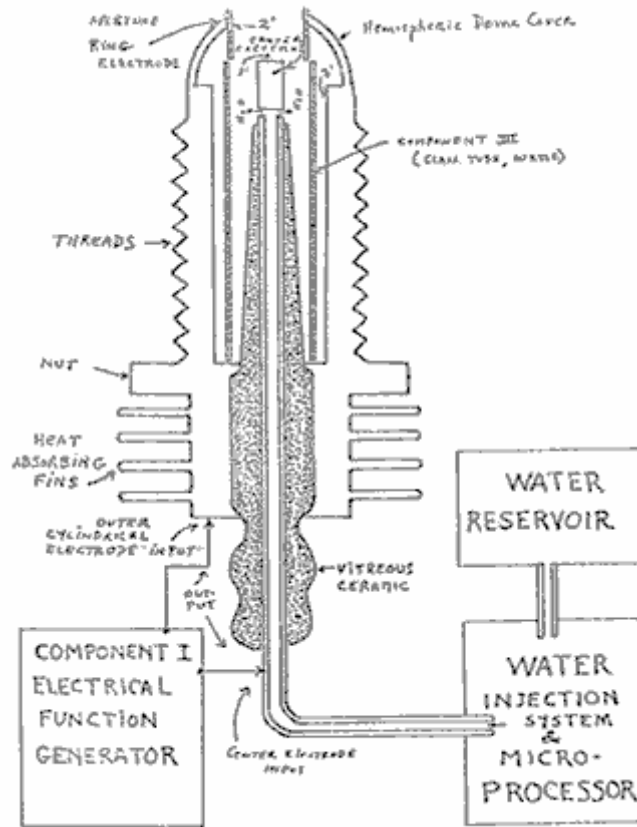
Figure 2: Thermodynamic Device
