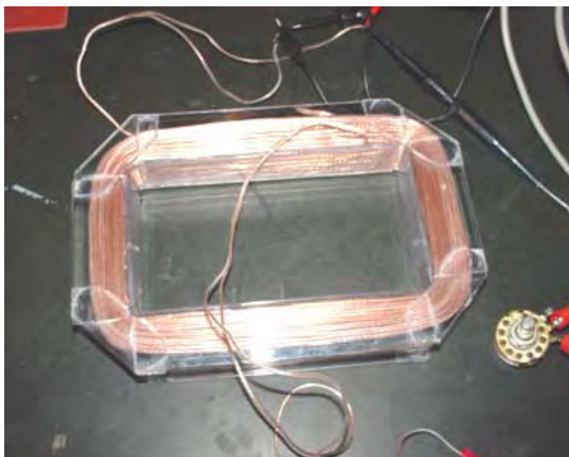
The Mike Motor Coil – 100' #22 Speaker Wire
