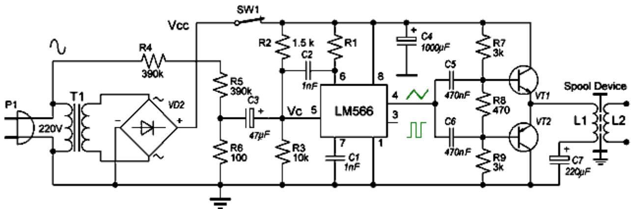
Fig. 9 Schematic of a simplified frequency-modulated signal generator.
