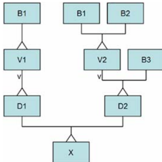
Figure 14-1. Inheritance hierarchy for Example 14-2
