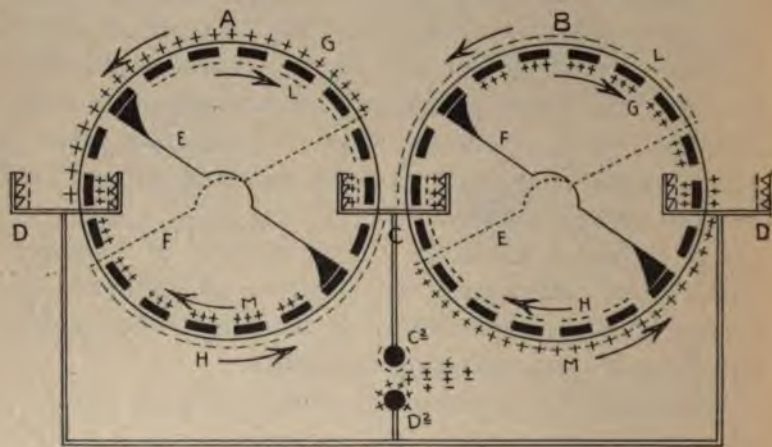
Fig. 32. Influence Machine.
