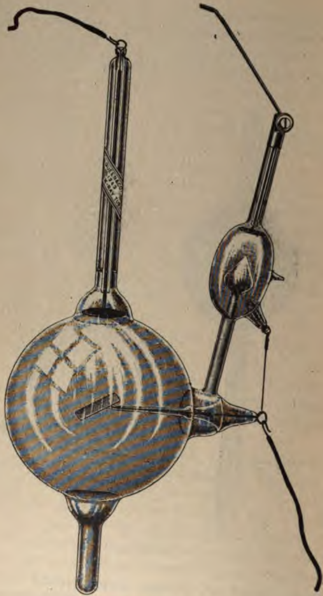
Fig. 58. Queen Self-regulating X-Ray Tube.
