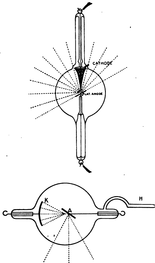
Fig. 56. Typical Tubes.
