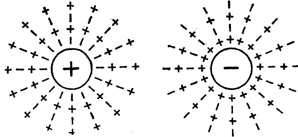
Electric Inductive (primary), and Induced (secondary) Potentials—Electric Analogues of Molecular Potentials in Equilibrium.
