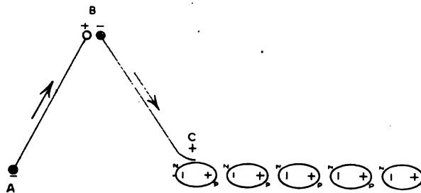
Fig. 105. Gland-cell Polarization.
