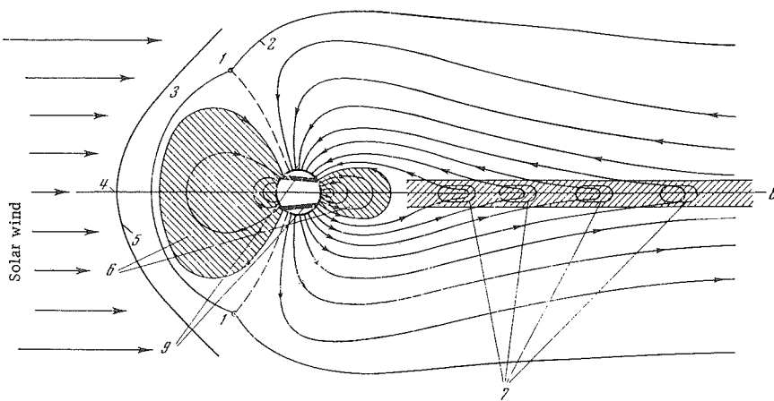
FIGURE 1. Schematic meridional section of earth's magnetosphere:
