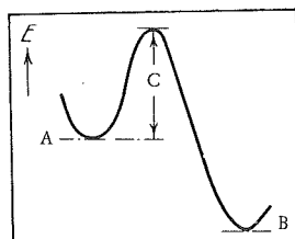
FIGURE 1. Metastable states:
