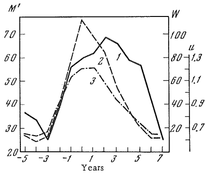
FIGURE 3. Mean cyclic curves of index M' of magnetic disturbance level (1), Wolf numbers (2), and u -measure (3)
