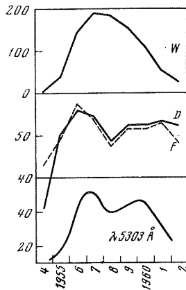
FIGURE 5. Changes in values of chemical F and D tests, in intensity of \lambda 5303 A coronal line, and in sunspot number W for 1954-1962
