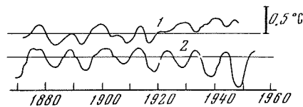
FIGURE 4. Variations in mean annual temperature in tropical zone (1) and Wolf numbers (2) (after Callendar)
