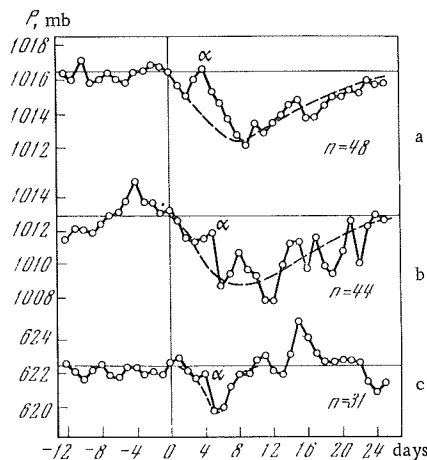
FIGURE 3. Reaction of atmospheric pressure in near-polar regions of earth to entry of high-energy solar protons into earth's upper atmosphere:
