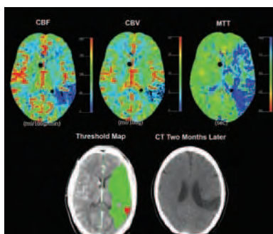
Fig. 9.6 Deconvolution method
