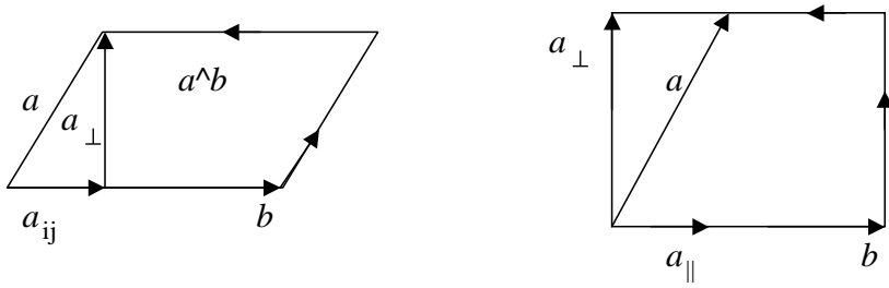
FIGURE 2.1 a_{\parallel} is collinear with b , and a_{\perp} is perpendicular to b .
