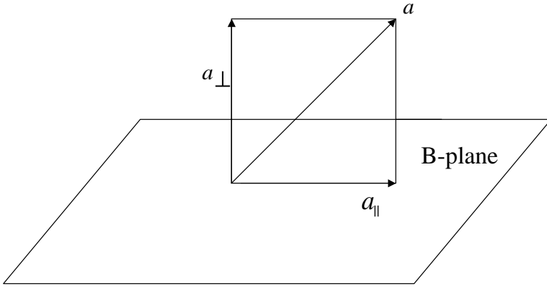
FIGURE 2.2 Projection and rejection of vector by a bivector B.
