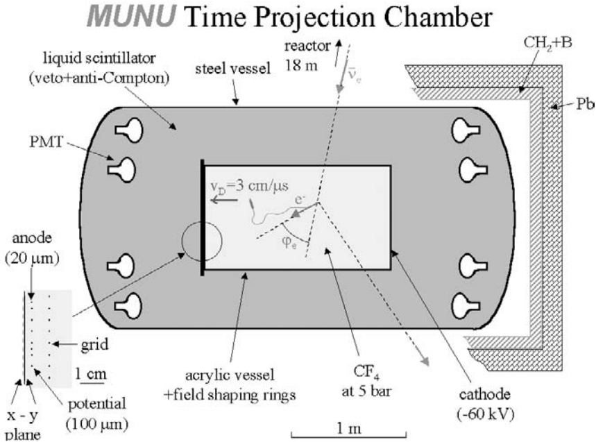
Figure 6.15. Layout of the MUNU TPC to search for magnetic moments at the Bugey reactor (from [Ams97]).
