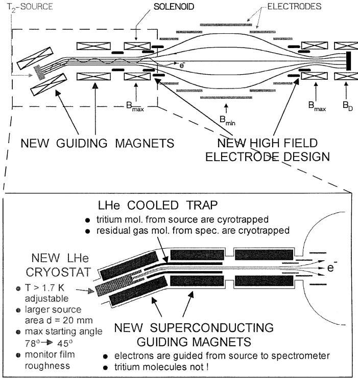
Figure 6.6. Layout of the Mainz electrostatic retarding spectrometer for measuring tritium \beta -decay.
