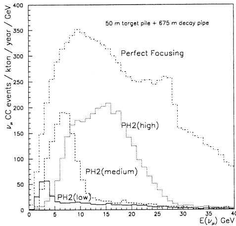
Figure 9.19. Three different options for the neutrino beam (NuMI) used by MINOS at Fermilab. The low-energy version has been chosen. Also shown is the spectrum for perfect focusing of secondary particles.
