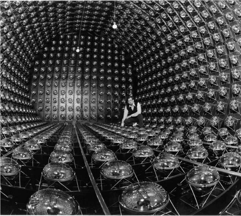
Figure 8.9. Photograph of the interior of the LSND detector (with kind permission of the LSND collaboration).
