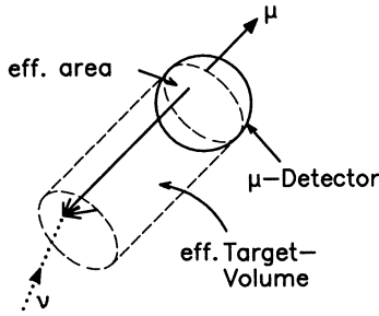
Figure 12.10. Schematic drawing to explain the concept of effective target volume and effective area in a neutrino telescope.
