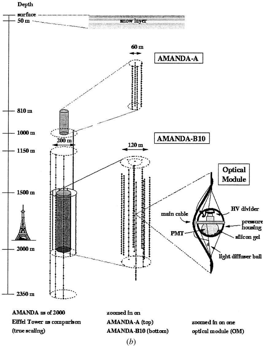
Figure 12.15. (a) Deployment of a string of photomultipliers. (b) Positions of AMANDA-A and AMANDA-B10 in the South Pole Ice (with kind permission of the AMANDA collaboration).
