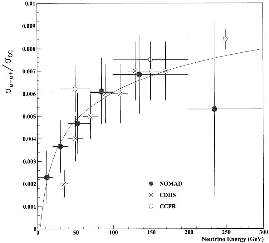
Figure 4.24. Compilation of observed dimuon versus single muon rates as a function of the visible energy E_{\text{vis}} obtained by CDHS, CCFR and NOMAD. The threshold behaviour due to the charm quark mass is clearly visible (from [Ast00]).
