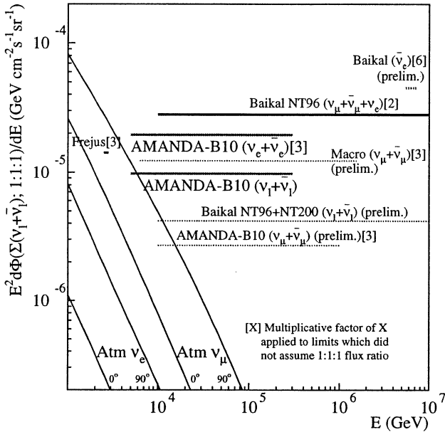
Figure 12.19. Limits on the cascade-producing neutrino flux, summed over the three active flavours, with multiplicative factors applied as indicated to permit comparison of limits derived. Also shown are the predicted horizontal and vertical \nu_e and \nu_\mu atmospheric fluxes (from [Nie03]).
