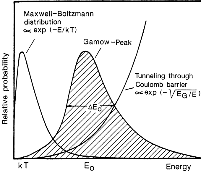
Figure 10.4. The most favourable energy region for nuclear reactions between charged particles at very low energies is determined by two effects which act in opposite directions. The first is the Maxwell–Boltzmann distribution with a maximum at kT , which implies an exponentially decreasing number of particles at high energies. The other effect is that the quantum mechanical tunnelling probability rises with growing energy. This results in the Gamow peak (not shown to true scale), at an energy E_0 , which can be very much larger than kT (from [Rol88]).
