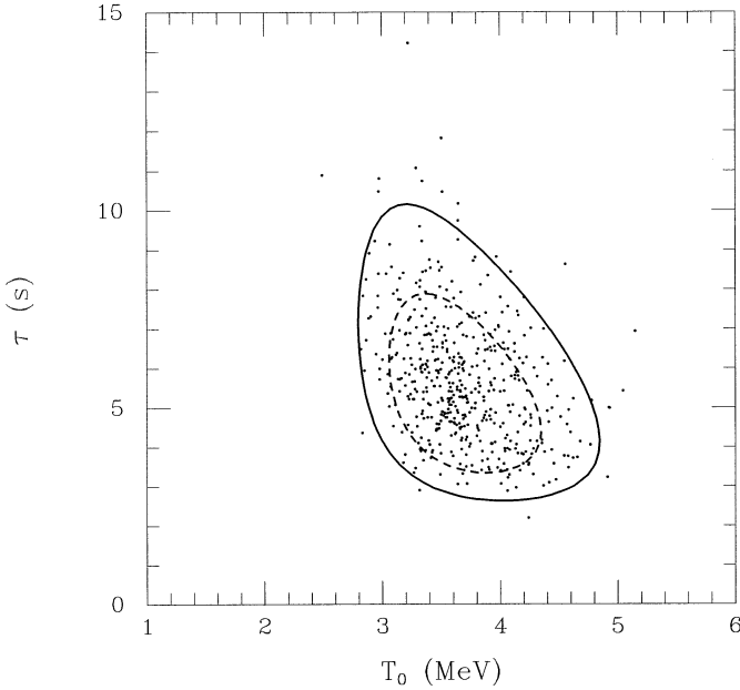
Figure 11.13. Loredo plot of parameter estimation of neutrino mass (from [Lor02]).
