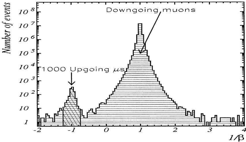
Figure 9.15. MACRO number of events as a function of 1/\beta . Beside the background spike of down-going muons (about 33.8 \times 10^6 events) a clear peak centred around 1/\beta = -1 caused by upward-going muons is seen.
