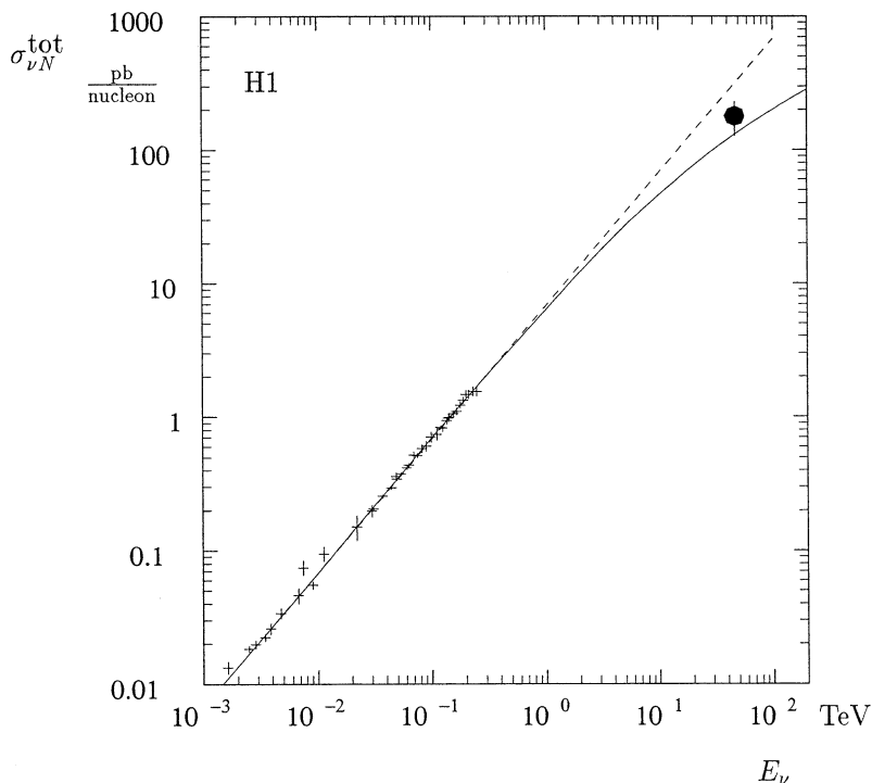
Figure 4.9. Compilation of \sigma(E_\nu) from \nu N scattering (crosses) and from the H1 experiment at DESY. The dotted curve corresponds to a prediction without a W -propagator ( m_W = \infty ), the full line is a prediction with W -propagator ( m_W = 80 GeV) (from [Ahm94]).
