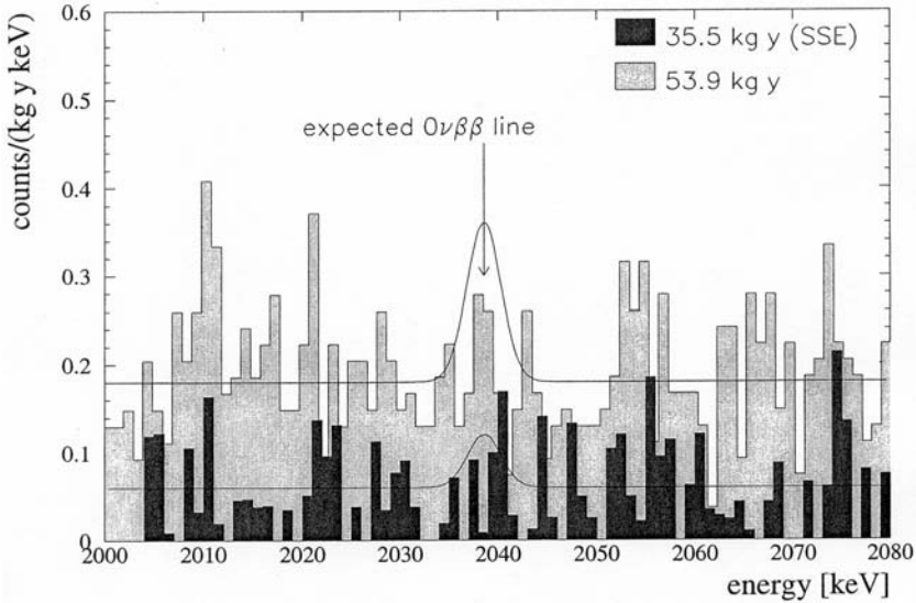
Figure 7.11. Observed spectrum around the expected 0\nu\beta\beta -decay peak of the Heidelberg–Moscow collaboration. No signal can be seen. The two different spectra correspond to measuring periods with (black) and without (grey) pulse shape discrimination (from [Kla01]).
