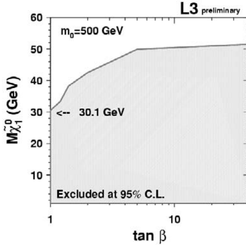
Figure 5.6. Neutralino mass limits as a function of \tan \beta as obtained by the DELPHI and L3 experiments at LEP (from [Kaz00]).
