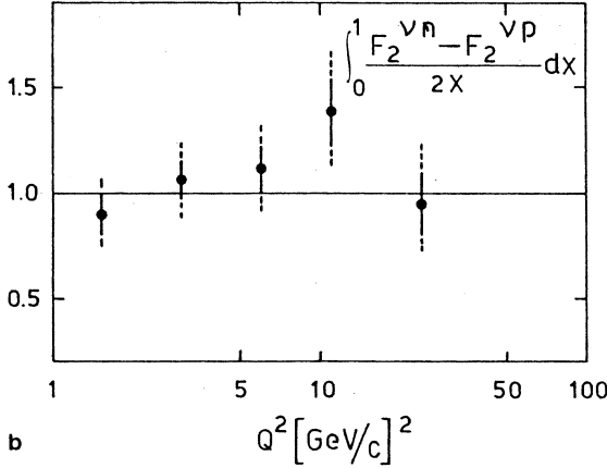
Figure 4.22. Test of Adler sum rule. The estimated uncertainties (dashed lines) are shown separately (from [All85a]).
