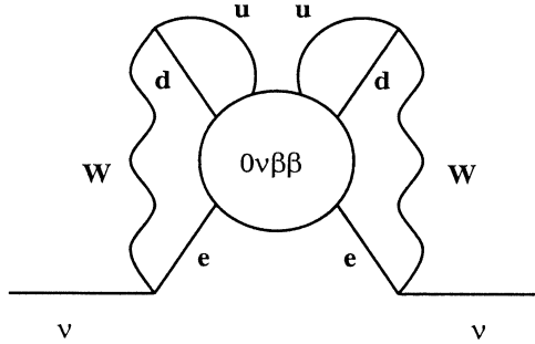
Figure 7.3. Graphical representation of the Schechter–Valle theorem. See text for details.
