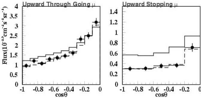
Figure 9.13. Super-Kamiokande upward-going muons flux versus absolute prediction. Left: Flux of through-going muons from horizontal ( \cos \theta = 0 ) to vertical upward ( \cos \theta = -1 ). Right: Upward-going muons which stop in the detector. Also shown are Monte Carlo expectations without oscillations and best-fit values assuming oscillations.
