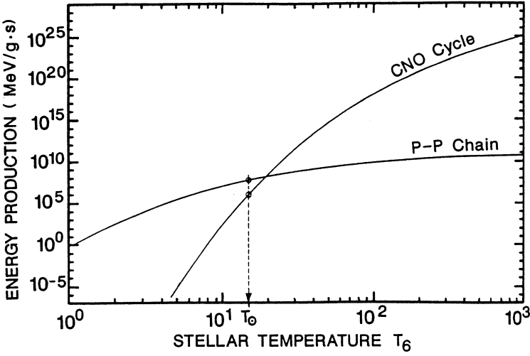
Figure 10.1. Contributions of the pp and CNO cycles for energy production in stars as a function of the central temperature. While the pp cycle is dominant in the Sun, the CNO process becomes dominant above about 20 million degrees (from [Rol88]).
