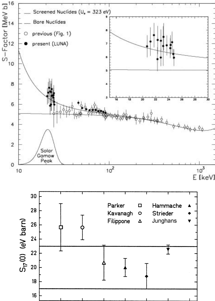
Figure 10.5. Two important cross sections in stellar astrophysics as measured with accelerators: top, compilation of ^3\text{He}(^3\text{He}, 2p)^4\text{He} data (from [Arp98]); bottom, Compilation of S_{17}(0) values of the ^7\text{Be}(p, \gamma)^8\text{B} reaction for various experiments (from [Jun02]).
