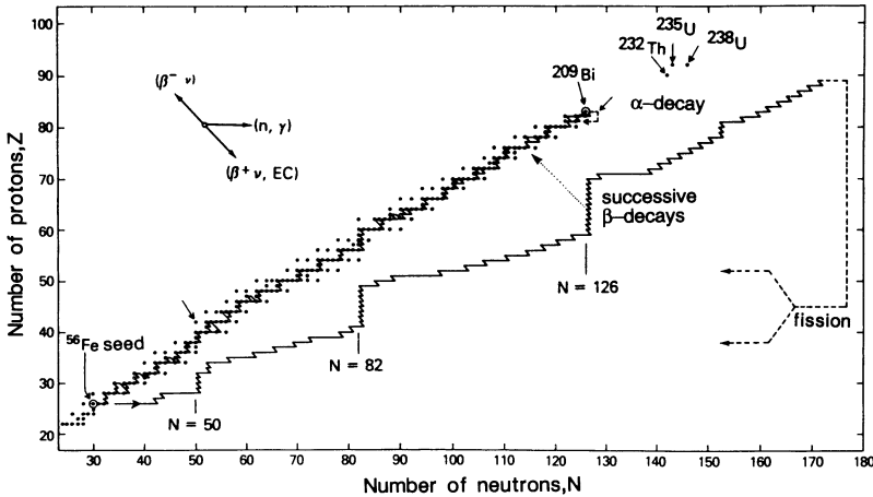
Figure 11.17. Illustration of the s- and r-process paths. Both processes are determined by (n, \gamma) reactions and \beta -decay. In the r-process the neutron-rich nuclei decay back to the peninsula of stable elements by \beta -decay after the neutron density has fallen. Even the uranium island is still reached in this process. The s-process runs along the stability valley (from [Rol88]).
