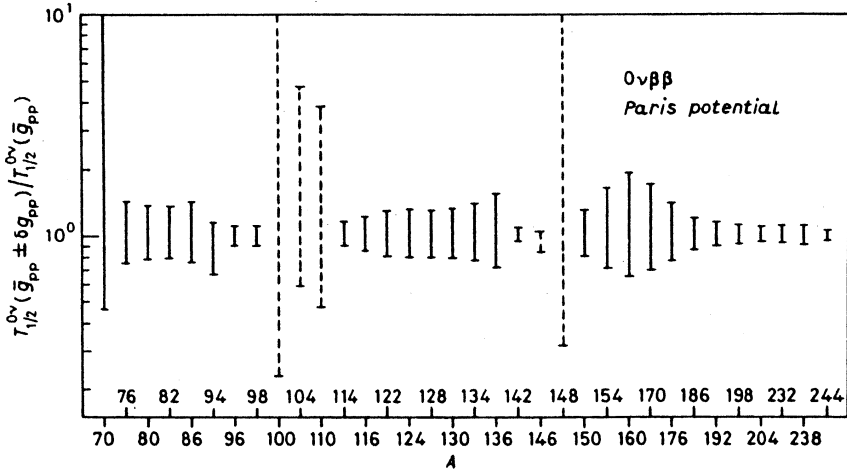
Figure 7.5. The uncertainty of 0\nu\beta\beta -decay half-lives calculated using QRPA, resulting from limited knowledge of the particle–particle force ( g_{pp} ) for potential double- \beta emitters (from [Sta90]).
