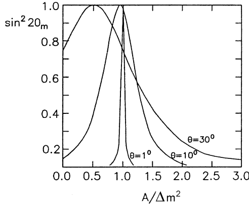
Figure 10.17. Dependence of the oscillation amplitude as a function of A/\Delta m^2 for different values of the vacuum mixing angle \theta ( \theta = 1^\circ, 10^\circ, 30^\circ ).
