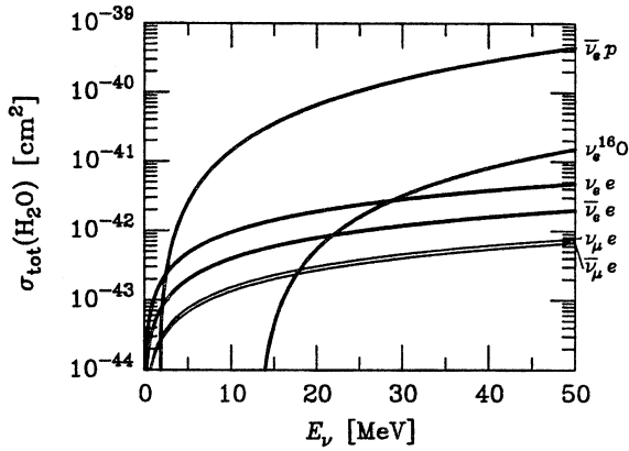
Figure 11.7. Some relevant total neutrino cross sections for supernova detection using water Cherenkov detectors. The curves refer to the total cross section per water molecule so that a factor of two for protons and 10 for electrons is already included (from [Raf96]).
