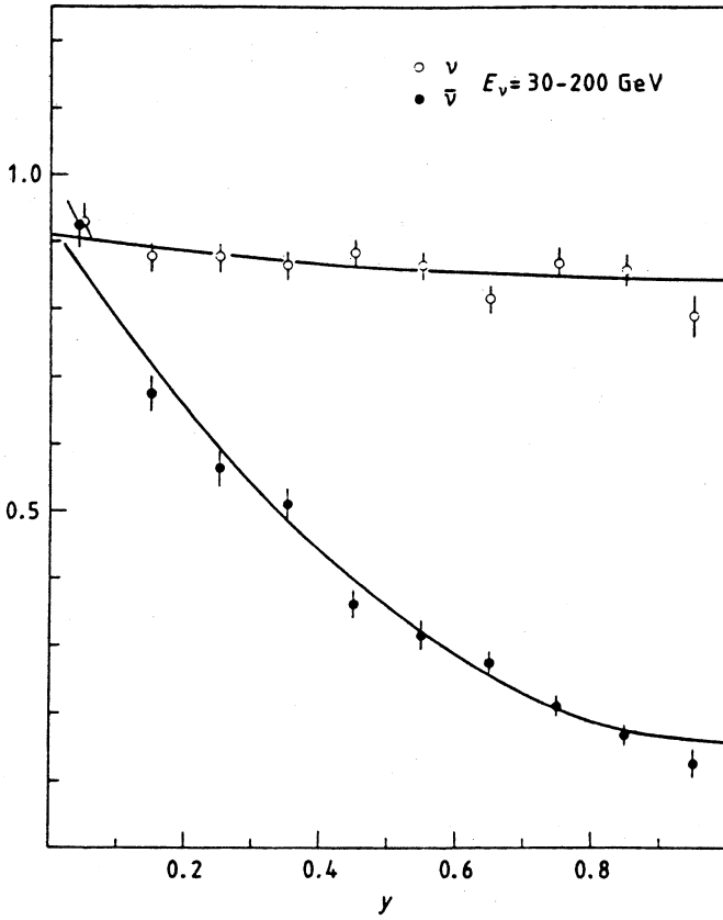
Figure 4.21. The differential cross sections versus y as obtained by CDHS for \nu N and \bar{\nu} N CC scattering. The dominant flat distribution for neutrinos and (1-y)^2 behaviour for antineutrinos show that left- and right-handed couplings are different. The distributions are explained by dominant scattering from valence quarks with left-handed couplings (from [Eis86]).
