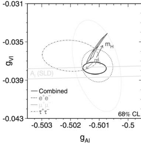
Figure 3.2. Lepton universality as probed in e^+e^- colliders at CERN and SLAC. The measured coupling constants g_V, g_A as obtained in the different flavours as well as the combined value are shown. The flat band shows the pull for varying the Higgs and top mass. This precision measurement indicates a universal coupling of the charged leptons to the weak vector bosons, whose value favours a relatively light Higgs boson (with kind permission of the LEP EW working group).
