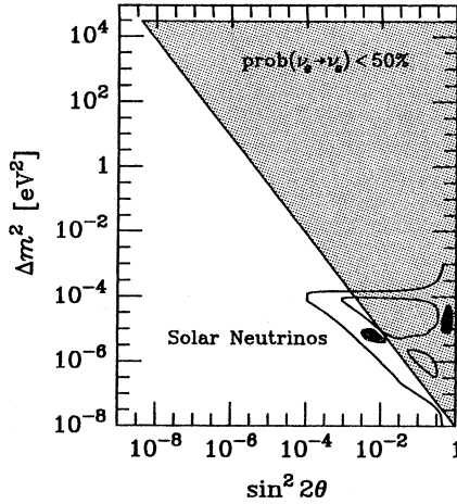
Figure 11.16. MSW triangle for the prompt \nu_e burst from a stellar collapse. In the shaded area the conversion probability exceeds 50% for E_\nu = 20 MeV. The solar LMA and SMA solutions as well as the old Kamiokande allowed range are also shown (from [Raf96]).
