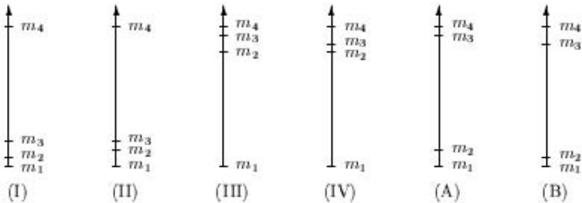
Figure 5.9. Various neutrino mass schemes which can be built on the existence of four different neutrino states to describe current neutrino oscillation evidences. The first four patterns are known as ‘3 + 1’ schemes, because of the one isolated state m_4 , while the remaining two are called ‘2 + 2’ schemes.
