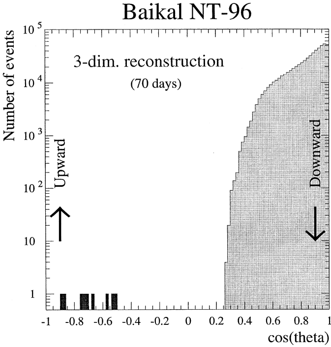
Figure 12.12. Angular distribution of muon tracks in the Baikal NT-96.
