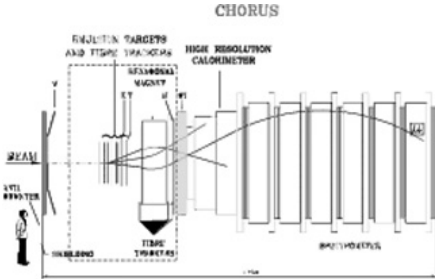
Figure 4.7. Schematic view of the CHORUS detector at CERN.
