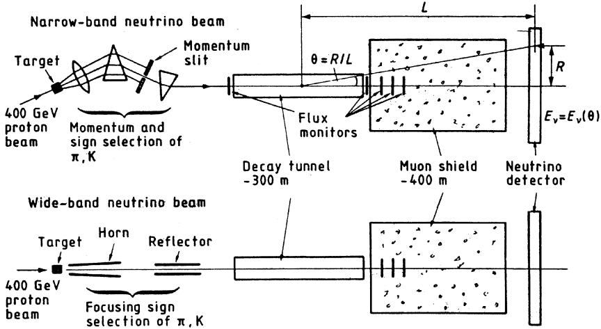
Figure 4.1. Schematic arrangements of neutrino beams: top, narrow-band beams; bottom, wide-band beams (from [Eis86]).
