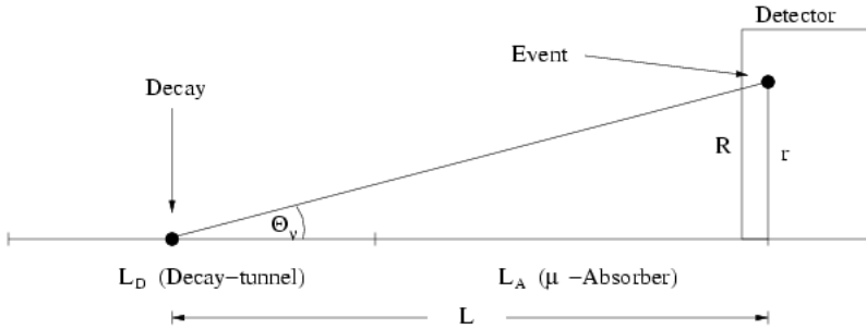
Figure 4.2. Geometric relation in a NBB between the position of meson decay (distance from the detector), decay angle \theta_\nu and radial position of the event in the detector.
