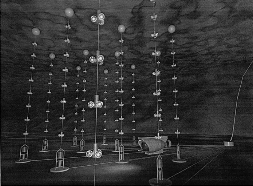
Figure 12.14. Schematic view of ANTARES (picture created by F Montanet, with kind permission of the ANTARES collaboration).
