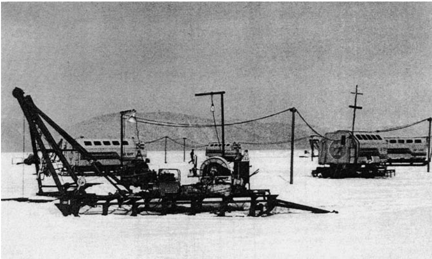
Figure 12.11. Installation of one of the rods of the NT-96 experiment in Lake Baikal. As the lake freezes over in winter, this season is ideal for installation (with kind permission of Ch Spiering).
