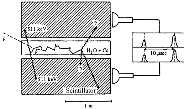
Figure 1.1. Schematic illustration of the experimental set-up for neutrino detections used by Cowan and Reines. A \text{CdCl}_2 loaded water tank is surrounded by liquid scintillators. They are used for a coincidence measurement of the 511 keV annihilation photons and the \gamma -rays emitted by the neutron capture on Cd (from [Rei58]).
