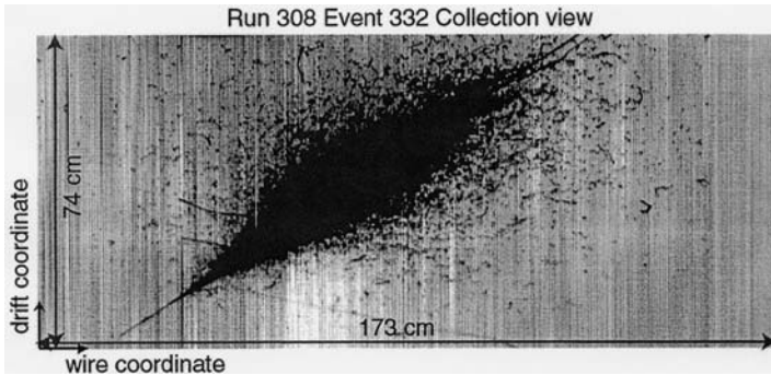
Figure 9.20. A broad electromagnetic shower as observed with the ICARUS T600 test module on the surface. This impressively shows the data quality obtainable with LAr TPCs (with kind permission of the ICARUS collaboration).
