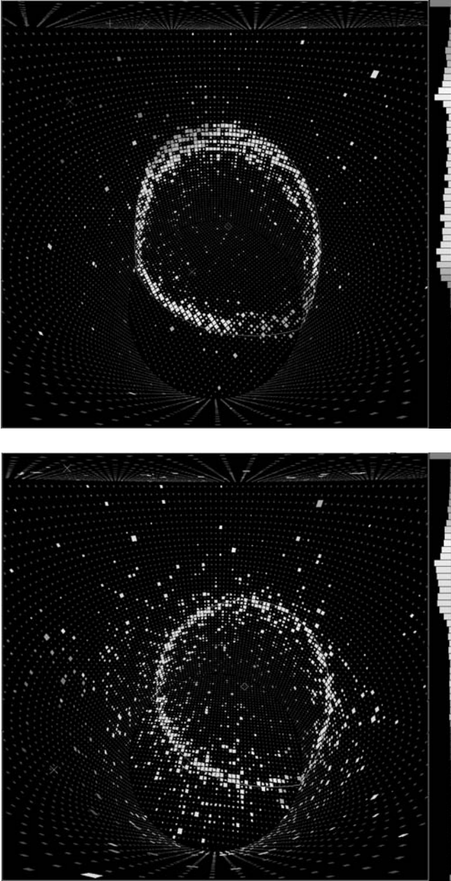
Figure 9.8. Two characteristic events as observed in Super-Kamiokande: top, sharp Cerenkov ring image produced by an muon; bottom, Diffuse Cerenkov ring image produced by an electron (with kind permission of the Super-Kamiokande collaboration).
