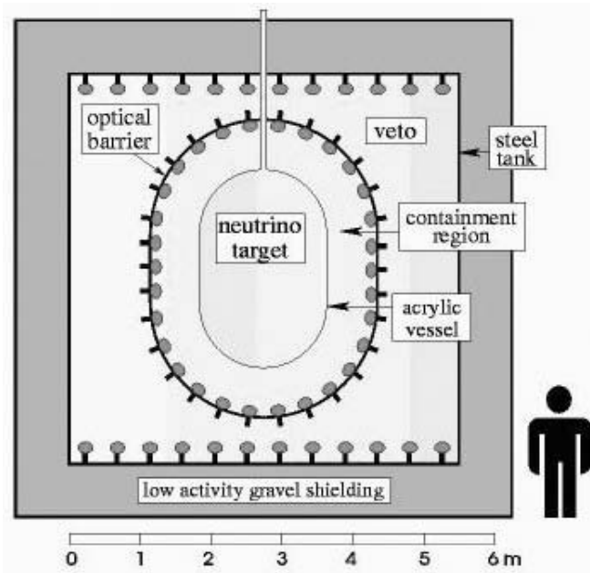
Figure 8.4. Schematic drawing of the CHOOZ detector.
