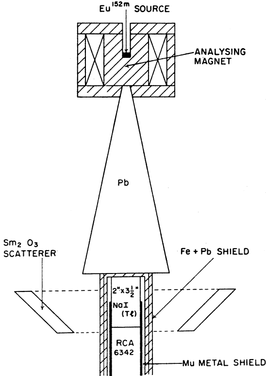
Figure 1.7. Experimental set-up of the Goldhaber experiment to observe the longitudinal polarization of neutrinos in EC reactions. For details see text (from [Gol58]).
