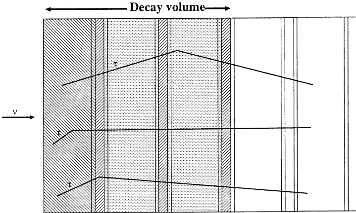
Figure 9.22. The emulsion cloud chamber (ECC) principle which will be used by OPERA. A \tau -lepton produced in a charged current interaction can be detected via two mechanisms. If the \tau -decay happens after the \tau has traversed several emulsion sheets, there will be a kink between the various track segments (upper curve). In a early decay an impact parameter analysis can be done, because the interesting track is not pointing to the primary vertex (lower two curves). For simplicity the additional tracks from the primary vertex are not shown.
