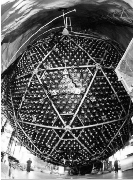
Figure 10.13. Construction of the Sudbury neutrino observatory (SNO) in a depth of 2070 m in the Craighton mine near Sudbury (Ontario). This Cerenkov detector uses heavy water rather than normal water. The heavy water tank is shielded by an additional 7300 t of normal water. The support structure for the photomultipliers is also shown (with kind permission of the SNO collaboration).
