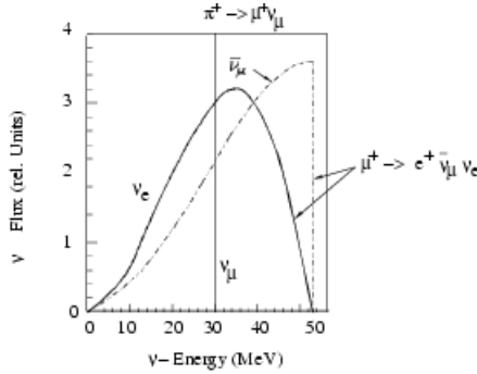
Figure 4.27. Energy spectrum of neutrinos coming from \pi^+ decay at rest. Beside a monoenergetic line of \nu_\mu at 29.8 MeV coming from pion decay there are the continuous spectra of \nu_e and \bar{\nu}_\mu with equal intensity and energies up to 52.8 MeV from muon decay.
