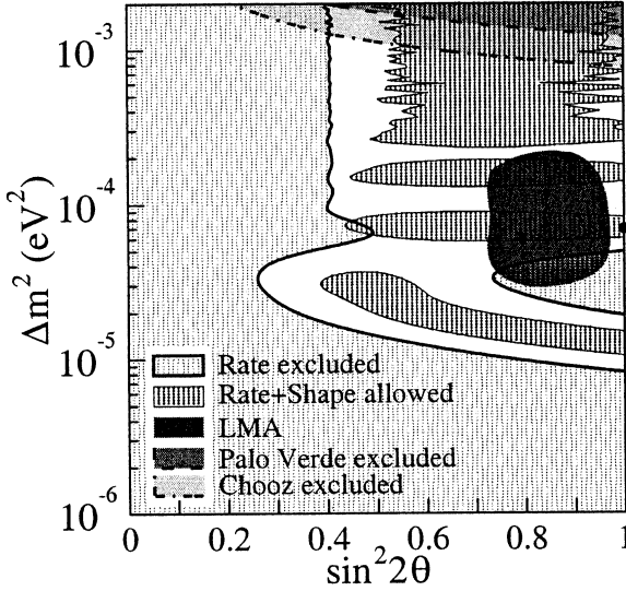
Figure 10.23. Regions in the \Delta m^2 – \sin^2 2\theta plot describing the observed deficit of KamLAND. As can be seen, there is an overlap of allowed parameters with the LMA solution of solar neutrino results (from [Egu03]).
