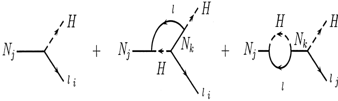
Figure 13.16. Feynman diagrams (tree level and radiative corrections) for heavy Majorana decays.
