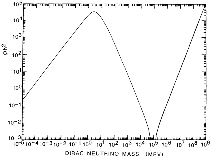
Figure 13.9. The contribution of stable neutrinos of mass m to the matter density of the universe. Only neutrino masses smaller than 100 eV and heavier than several GeV to TeV are cosmologically acceptable. Otherwise neutrinos have to be unstable (from [Tur92a]).
