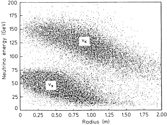
Figure 4.3. Scatter plot of E_\nu with respect to radial event position for CC events as obtained with the CDHS detector at the CERN SPS. The dichromatic structure of the narrow-band beam (NBB) with E_M = 160 GeV is clearly visible and shows the neutrino events coming from pion and kaon decay (from [Ber87]).
