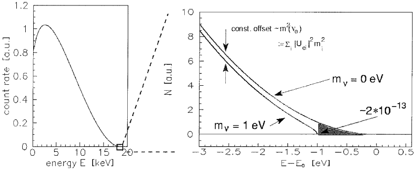
Figure 6.5. Endpoint region of a beta spectrum. The effect of a finite neutrino mass is a reduced endpoint at Q - m_\nu c^2 (from [Wei03]).
