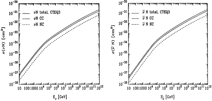
Figure 12.7. Total as well as NC and CC cross sections for high-energy neutrinos (left) and antineutrinos (right) (from [Gan96]).
