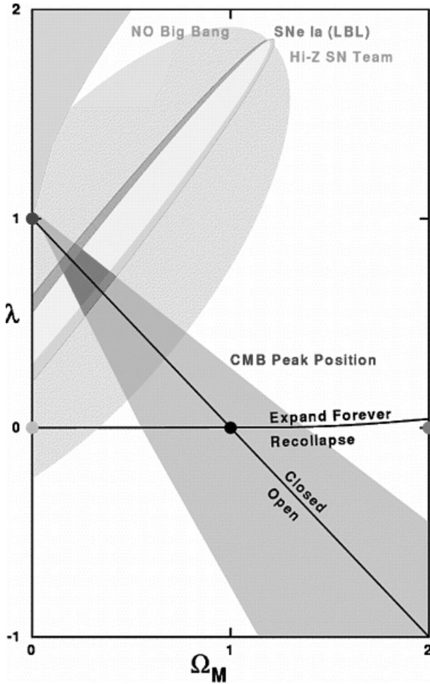
Figure 13.8. \Omega_\Lambda versus \Omega_m plot. The determination of cosmological parameters using high- z supernovae type Ia and the acoustic peak positions in the CMB power spectrum result in quite complementary information. The combined parameter values show with high significance a non-vanishing cosmological constant and an \Omega_\Lambda \approx 0.7 and \Omega_m \approx 0.3 .
