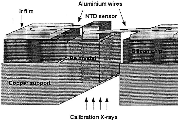
Figure 6.10. Sketch of the rhenium microcalorimeter with an absorbing mass of metallic Re, a neutron-transmutation-doped (NTD) Ge thermistor on top and two aluminium wires for thermal and mechanical connections (from [Meu98]).
