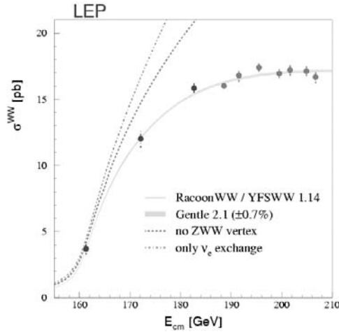
Figure 3.9. Measurements of the cross section ( e^+e^- \rightarrow W^+W^- ) as a function of the centre-of-mass energy obtained while LEP2 was running. The threshold behaviour can be used to determine the W -mass and the behaviour shows the effect of self-coupling of the gauge bosons. Scenarios with no ZWW vertex and pure \nu_e exchange are clearly excluded. Predictions of Monte Carlo simulations are shown as lines (with kind permission of LEP EW working group).
