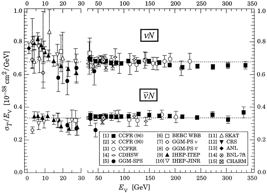
Figure 4.8. Compilation of \sigma/E_\nu in \nu N and \bar{\nu} N scattering as a function of E_\nu obtained by several experiments (from [PDG02]).
