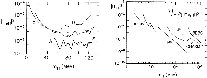
Figure 6.18. Limits on U_{eH} and U_{\mu H} as a function of a heavy neutrino mass m_H . Left: Curves A and B correspond to measurements at TRIUMF [Bri92], curves C and D to earlier experiments from [Bri92]. Right: From [Boe92].
