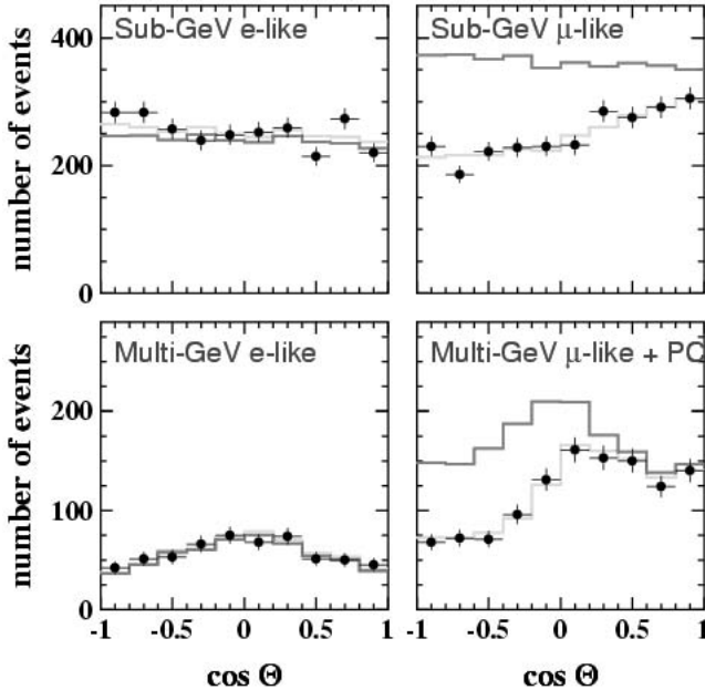
Figure 9.9. Super-Kamiokande zenith-angle distribution for e-like (left) and \mu -like events (right), also divided into sub-GeV (upper row) and multi-GeV samples (lower row). A clear deficit is seen in the upward-going muons. The full curves are the Monte Carlo expectations together with an oscillation fit of \Delta m^2 = 2.4 \times 10^{-3} and \sin^2 2\theta = 1.0 .
