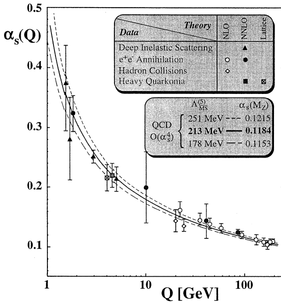
Figure 5.1. Top: Qualitative evolution with Q^2 of the three running coupling constants within the grand unification scale SU(5) . Bottom: The clearest effect of running coupling with achievable energies is observed in the strong coupling \alpha_s . Various experimental quantities can be used for its determination (from [Bet00]).
