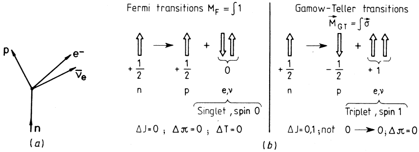
Figure 6.1. Neutron beta decay (a) and spin balance (b) for Fermi and Gamow-Teller transitions.
