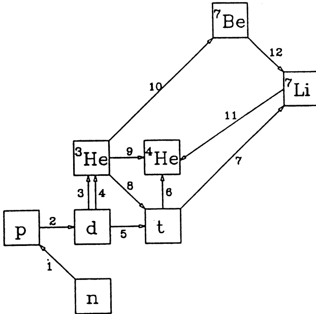
Figure 13.14. The 12 fundamental reactions in the chain of synthesis of the light elements, illustrating which elements can be built up in this way (from [Smi93b]). Labels indicate the following reactions: (1) n \leftrightarrow p , (2) p(n, \gamma)d , (3) d(p, \gamma)^3\text{He} , (4) d(d, n)^3\text{He} , (5) d(d, p)t , (6) t(d, n)^4\text{He} , (7) t(\alpha, \gamma)^7\text{Li} , (8) ^3\text{He}(n, p)t , (9) ^3\text{He}(d, p)^4\text{He} , (10) ^3\text{He}(\alpha, \gamma)^7\text{Be} , (11) ^7\text{Li}(p, \alpha)^4\text{He} , (12) ^7\text{Be}(n, p)^7\text{Li} .
