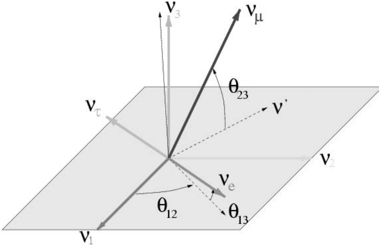
Figure 5.7. Graphical representation of the mixing matrix elements between flavour and mass eigenstates.
