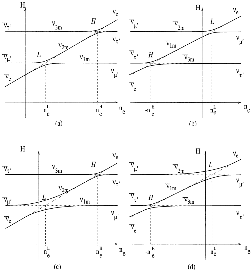
Figure 11.20. Level crossing diagrams for small solar mixing (upper line) and large mixing (lower line) as realized by LMA. The left-hand column corresponds to normal and the right-hand to inverted mass hierarchies. The part of the plot with N_e < 0 is the antineutrino channel.
