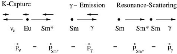
Figure 1.6. Neutrino helicity in the Goldhaber experiment. Long thin arrows are the momenta and short thick arrows are the spin directions in the three processes.
