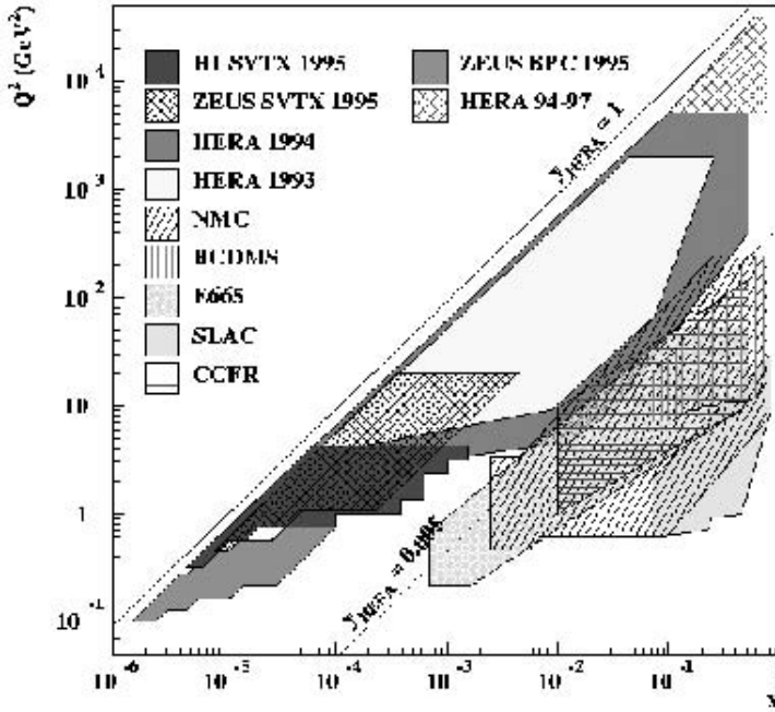
Figure 4.11. Allowed kinematic regions in the (x, Q^2) plane that can be explored by various experiments.
