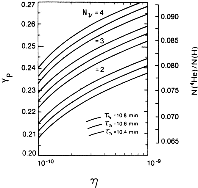
Figure 13.15. A more detailed illustration of the {}^4\text{He} abundance as a function of the baryon/photon ratio \eta = n_B/n_\gamma . The influence of the number of neutrino flavours and the neutron lifetime on the predicted {}^4\text{He} abundance can clearly be seen (from [Yan84]).
