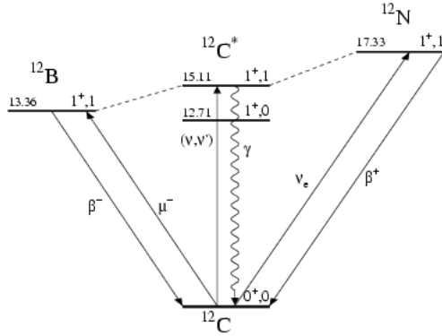
Figure 4.28. The A = 12 isobaric analogue triplet together with various possible transitions involving the ^{12}\text{C} ground state.
