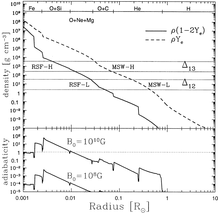
Figure 11.22. Position of the various resonances within the supernova. The two horizontal bands correspond to \Delta_{12} = \Delta m_{12}^2 \cos \theta_{12} / 2\sqrt{2}G_F E\nu and \Delta_{13} = \Delta m_{13}^2 \cos \theta_{13} / 2\sqrt{2}G_F E\nu . The band width comes from the energy range 5–70 MeV. At intersections between the full, broken curves and the horizontal bands, the RSF and MSW conversions occur (from [And03]).
