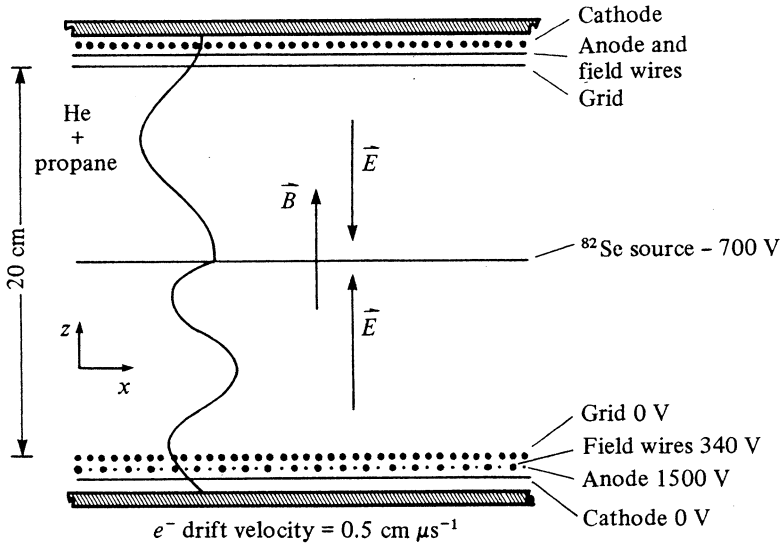
Figure 7.13. Schematic view of the setup of the TPC at UC Irvine, showing the wires, direction of the fields and the ^{82}\text{Se} source. A sample electron trajectory is shown on the left-hand side.
