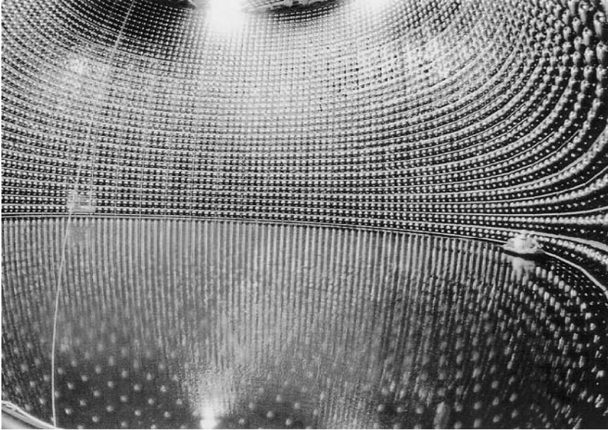
Figure 9.6. Photograph of the Super-Kamiokande detector during filling (with permission of the Kamioka Observatory, ICRR, Tokyo).
