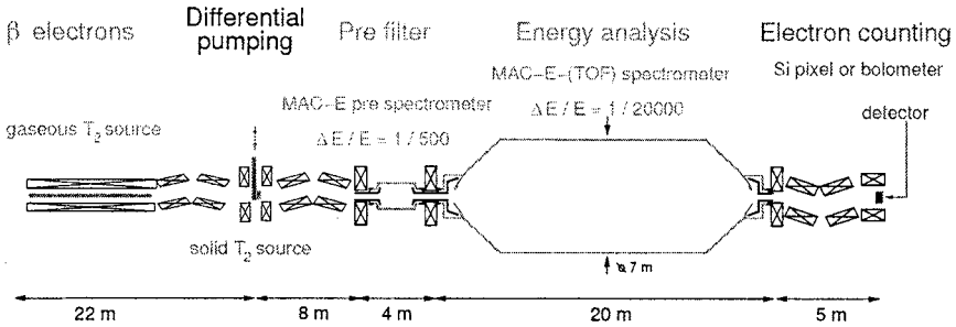
Figure 6.9. Schematic layout of the new proposed KATRIN spectrometer (from [Wei03]).
