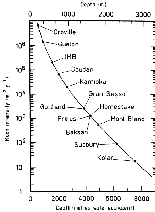
Figure 7.9. Muon intensity versus depth of some of the most important underground laboratories. Their shielding depth is given in metres of water equivalent (mwe) together with the attenuation of the atmospheric muon flux.
