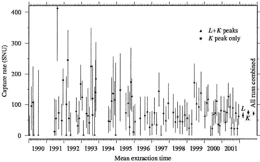
Figure 10.12. Davis plot of 11 years of data-taking with SAGE.
