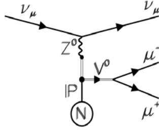
Figure 4.15. Feynman graph for diffractive vector meson production via the exchange of a pomeron \mathcal{P} .
