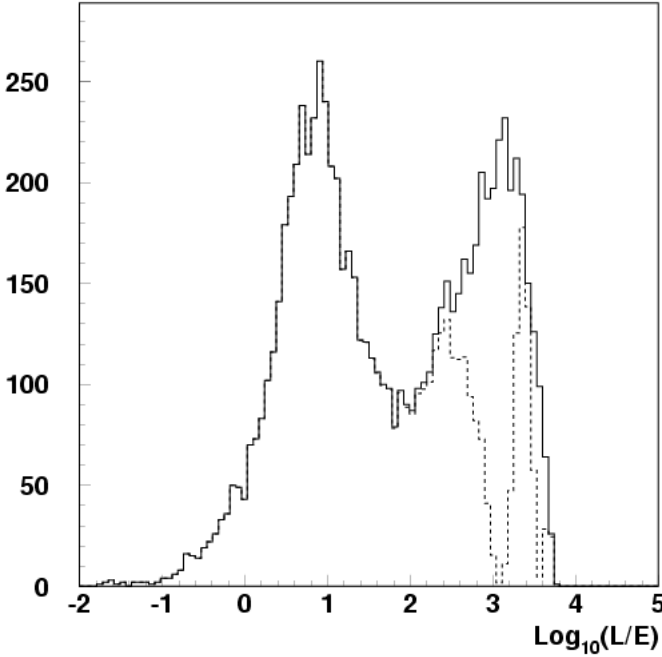
Figure 9.11. L/E double-bump structure. The bump at low values corresponds to downward-going events, the one at high L/E is due to upward-going events (from [Lip01]).
