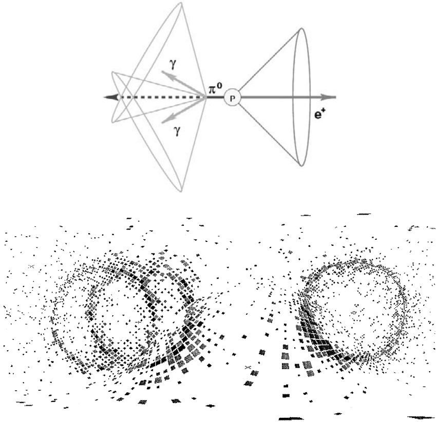
Figure 5.2. Top: Schematic picture of a proton decay p \rightarrow e^+ \pi^0 and the corresponding Cerenkov cones. Bottom: Monte Carlo simulation of such a proton decay for a water Cerenkov detector like Super-Kamiokande from [Vir99].
