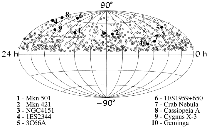
Figure 12.20. Skymap of 815 events from the point-source analysis of AMANDA-B10. The horizontal coordinates are right ascension and the vertical coordinates are declination. Also shown are the sky coordinates for ten potential high-energy neutrino sources (from [Ahr03]).
