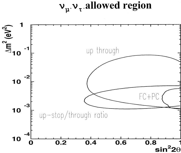
Figure 9.10. Allowed \Delta m^2 versus \sin^2 2\theta regions of the various Super-Kamiokande atmospheric neutrino signals by \nu_\mu - \nu_\tau oscillations.
