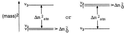
Figure 5.8. Normal and inverted mass hierarchies for three neutrinos. The inverted scheme is characterized by a \Delta m_{23}^2 = m_3^2 - m_2^2 < 0 .
