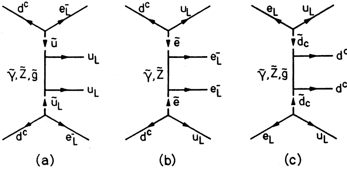
Figure 7.15. Dominant Feynman graphs from R -parity-violating SUSY contributing to double \beta -decay (from [Moh86]).
