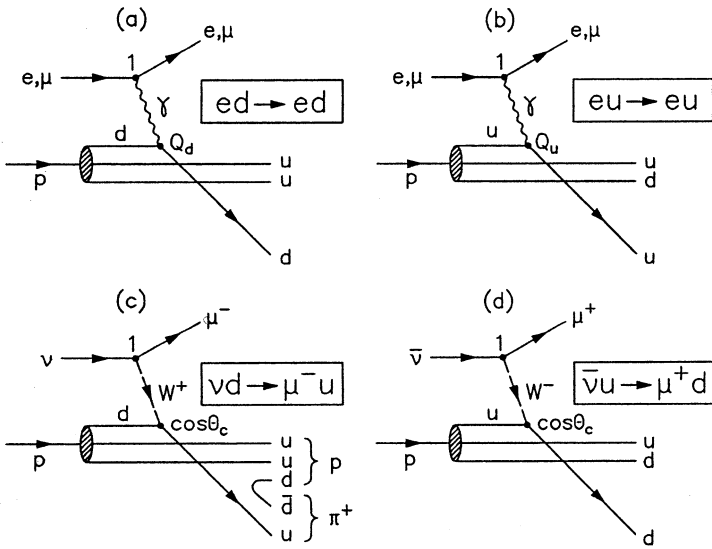
Figure 4.16. Graphs for the dominant processes in DIS in ep/\mu p scattering (a, b), \nu p scattering (c) and \bar{\nu} p scattering (d).
