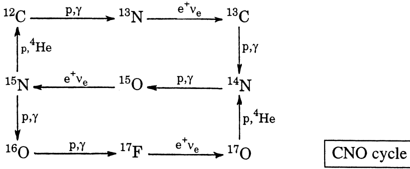
Figure 10.3. Representation of the CNO process. This also burns hydrogen to helium with C, N and O acting as catalysts and is responsible for 1.6% of the solar energy.
