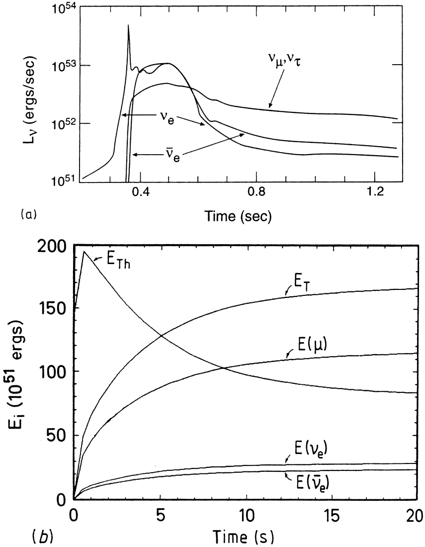
Figure 11.6. (a) Calculated luminosity of a 2M_\odot 'Fe' core of an \approx 25M_\odot main sequence star as a function of the time from the start of the collapse for the various neutrino flavours (from [Bru87]). (b) Cooling of a hot proto-neutron star of 1.4M_\odot in the first 20 s after gravitational collapse. E_{Th} denotes the integrated internal energy, E_T is the total energy released and E_{\nu_e} and E_{\bar{\nu}_e} are the total energies emitted as \nu_e and \bar{\nu}_e , respectively. E_\mu is the energy emitted as \nu_\mu , \bar{\nu}_\mu , \nu_\tau and \bar{\nu}_\tau . All energies are in units of 10^{51} erg (from [Bur86]).
