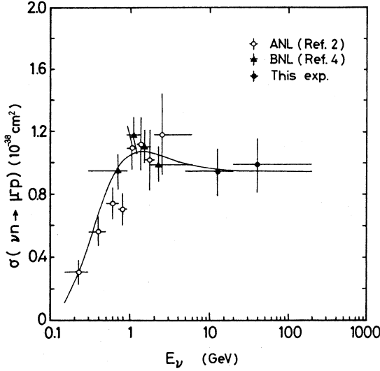
Figure 4.12. Compilation of results for \sigma(\nu_{\mu}n \rightarrow \mu p) of various experiments. The curve shows the prediction of V-A theory with M_A = 1.05 GeV (from [Kit83]).
