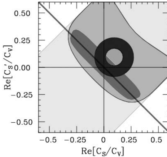
Figure 3.1. Comparison of constraints on scalar couplings in weak interactions. Limits included are from neutron decay alone (light shaded) and in combination with results from the polarization of electrons in ^{14}\text{O} and ^{10}\text{C} decay. The constraints obtained on Fierz terms coming from ^{22}\text{Na} and on the quantity a (see chapter 6) from ^6\text{He} the dark grey region results (see also chapter 6 for more explanations) are also added. The black circle corresponds to positron–neutrino correlation measurements in ^{32,33}\text{Ar} . The narrow area along the line at -45 degrees results from constraints on Fierz terms from 0^+ \rightarrow 0^+ transitions (from [Adl99]).
