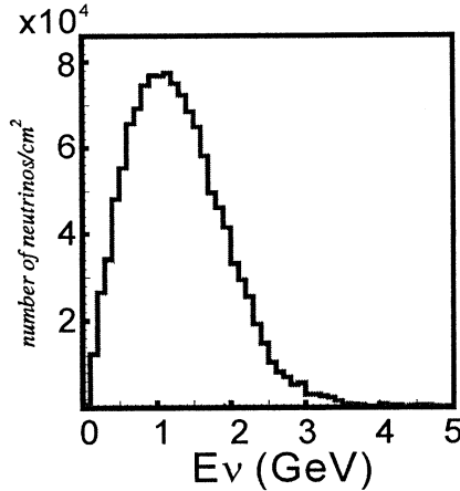
Figure 9.17. Neutrino energy spectrum of the K2K neutrino beam. Because of the relatively low beam energy no \nu_\tau appearance searches can be performed.
