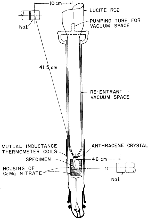
Figure 1.3. Schematic diagram showing the demagnetisation cryostat used in the measurement of the angular distribution of the electrons from the \beta -decay of ^{60}\text{Co} nuclei (from [Wu57]).
