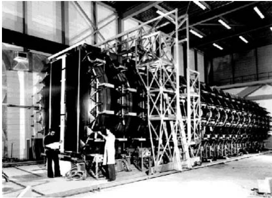
Figure 4.5. Photograph of the CDHS detector at CERN (with kind permission of CERN).
