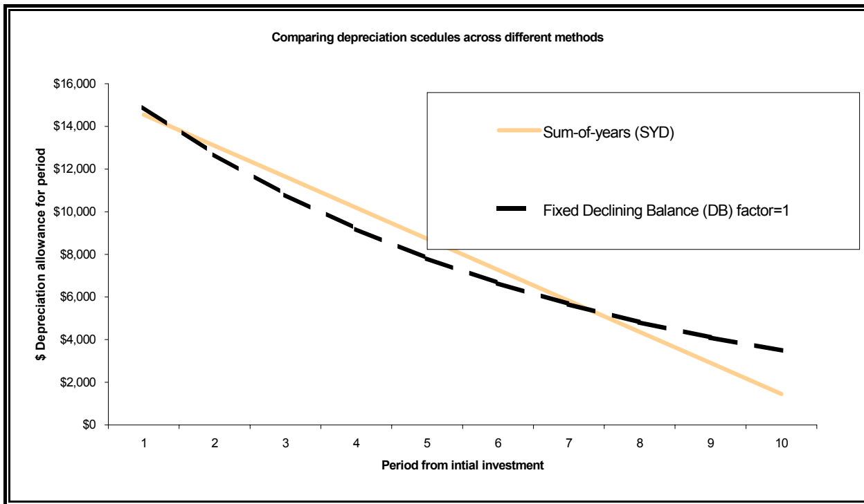
Figure 102: Comparing SYD and DB
