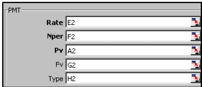
Figure 86: The function PMT
