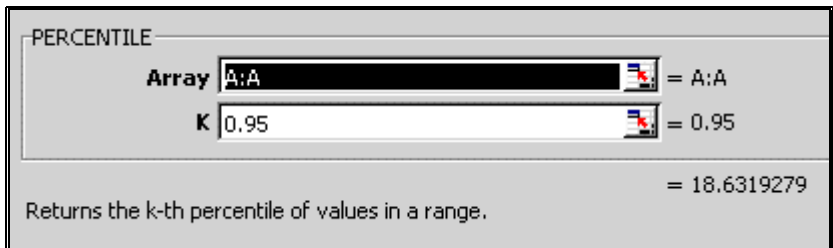
Figure 119: Estimating the 95th percentile
