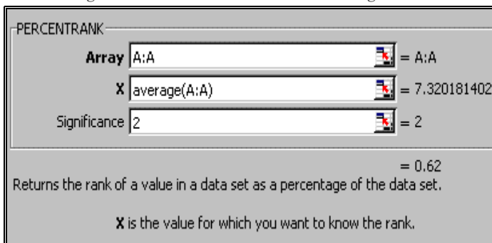
Figure 121: Percentrank of the average/mean
