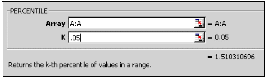
Figure 118: Estimating the 5th percentile. K is the percentile value in the range 0 to 1.
