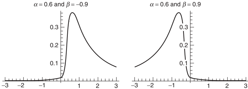
Figure 4.4.10 Stable Pareto density (mass in tails increases as \alpha decreases)
