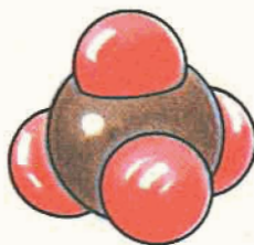
TWO LABORATORY MODELS SHOWING THE METHANE MOLECULE.
