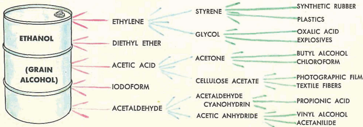
THE "FAMILY TREE" OF ETHANOL—WITH SOME OF ITS CHILDREN, GRANDCHILDREN, AND GREAT-GRANDCHILDREN.
