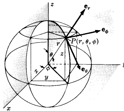
Fig. 22-13. Spherical coordinates.
