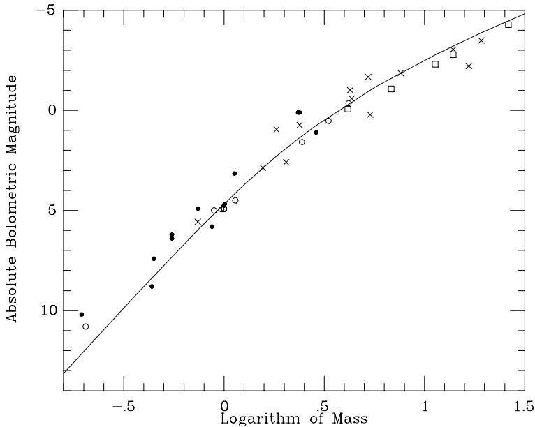
FIG. 7.6. The ‘Mass–Luminosity Curve’ re-drawn from Eddington (1926). Here he plotted his theoretical curve (the line on the diagram) against the luminosities and masses (in terms of the mass of the sun) of the few stars for which these quantities were then known. The vertical axis is related to the logarithm of the wattage of the star, which increases upwards. ‘Bolometric’ means summed over all wavelengths. Circles represent well-studied binary stars, dots less well-studied binaries, crosses eclipsing binaries and squares Cepheids.
