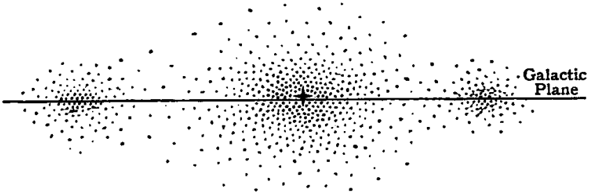
FIG. 7.3. Eddington's idea of the cross-section of the Universe given in his 1914 book, Stellar Movements and the Structure of the Universe . The sun is at the centre of the system and is marked by a cross symbol in the diagram. A few years later, Shapley's discovery completely altered this simple picture.
