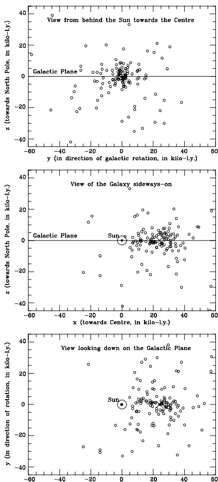
FIG. 8.2. The distribution of globular clusters in space, derived from modern data (Harris 1996). The positions of the sun \odot and the Galactic Centre \times are marked in the bottom and middle panels. Both are in the centre of the top panel. Using diagrams of this kind, Shapley guessed that the centre of the globular cluster system is the centre of the Milky Way galaxy. Each diagram is about 120,000 \times 90,000 light years. The middle panel can be compared with the Herschel (Fig. 4.4) and Eddington (Fig. 7.3) sun-centered diagrams.
