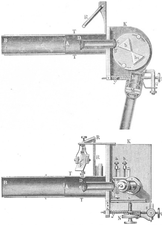
FIG. 5.5. Plan (top) and elevation (bottom) of Huggins' first spectroscope. The tube B to the left was inserted into the telescope and the star was focussed onto the slit at D. The light passed through the collimator lens g into the prisms h. The spectrum was viewed through the small telescope L. The arrangements around R were for introducing light from a comparison lamp. (From Lockyer 1874.)
