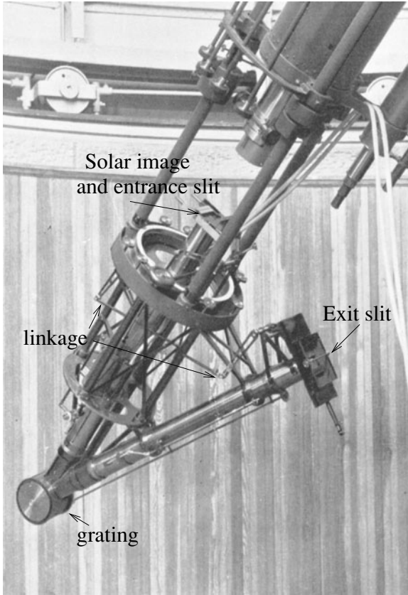
FIG. 6.1. First successful spectroheliograph attached to the telescope at Hale's Kenwood Observatory. Only light from a narrow part of the image that fell on the entrance slit could enter the spectrograph. The grating at the bottom reflected a specific wavelength range to the exit slit, beneath the photographic plate at the output of the instrument. By moving the entrance and exit slits together through a linkage, a complete picture of the sun at a single wavelength could be built up. (From Hale 1908.)
