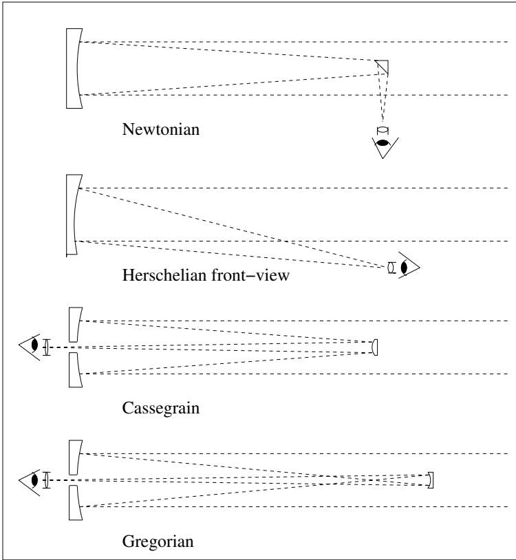
FIG. 3.3. The optics of various reflecting telescopes. At the top is Newton's design, with a paraboloidal and a flat mirror. Herschel invented the 'front view' to avoid the substantial losses associated with a second reflection; however, its image quality is poor except in very long instruments. The Cassegrain combines a paraboloidal primary with a hyperboloidal secondary. The design of James Gregory, a friend of Newton, is similar, but with an ellipsoidal secondary. Most modern telescopes are Cassegrains or variants thereof.
