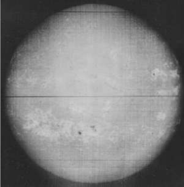
FIG. 6.3. Early spectroheliogram from Kenwood Observatory, dated 23 June 1892. It shows dark sunspots and white cloudy faculae. For this photograph the instrument was tuned to the wavelength of calcium, which is very hot in the faculae and therefore shows up as bright patches. (The horizontal dark lines were caused by the imperfectly coordinated movements of the entrance and exit slits.) (SAAO).
