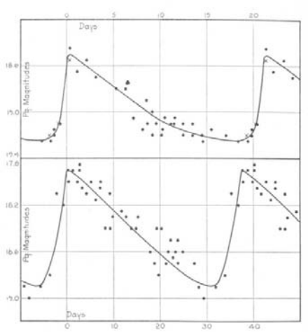
FIG. 9.2. The light curves of two Cepheid variables in the galaxy NGC 6822, from Hubble (1925). The upper star has a period of about 21 days and the lower about 37 days. From their average stellar magnitudes (brightnesses) and Shapley's calibration work, Hubble could derive the distance of NGC 6822, showing that it was far beyond the confines of our own galaxy, the Milky Way.
