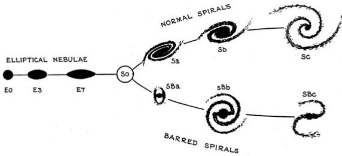
FIG. 9.4. The Hubble 'Tuning Fork' diagram of galaxies, from his book of 1936, The Realm of the Nebulae .
