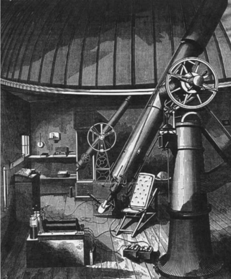
FIG. 5.4. The interior of Huggins's dome as it appeared in the 1860s. The telescope is his 8-in. Clarke/Cooke and his first spectroscope (see Fig 5.5) is shown mounted on the eye end. In the foreground is an induction coil, used to generate the high voltages needed to make spark spectra for comparison purposes. (Woodcut by J. Swain, courtesy Prof R. French, Whitin Observatory, Wellesley College, Massachusetts.)
