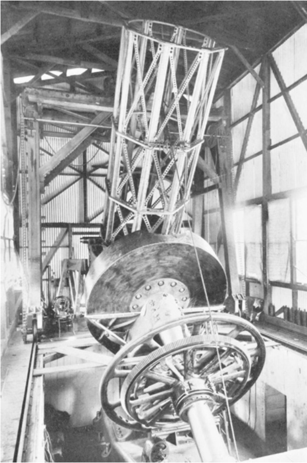
FIG. 6.5. The 60-in. telescope under construction in Pasadena. The large circular structure near the telescope tube contained a mercury flotation system to relieve the weight on the bearings (Hale 1908).
