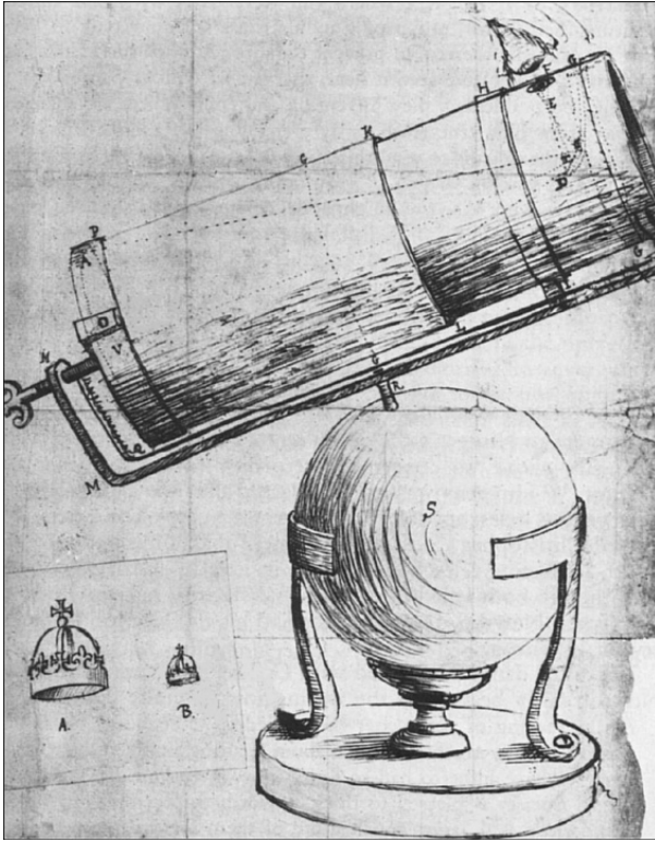
FIG. 3.2. Reflecting telescope made by Newton and presented to the Royal Society (see Turnbull 1959 for details). The light was collected by the main mirror A, of about 6\frac{1}{3} in. (16 cm) focal length at the left end of the tube and passed via a flat mirror DE to the eyepiece F of about \frac{1}{6} in. (4.2 mm) focal length (see also Fig 3.3). The magnification was about 37 times. Focusing was achieved by turning the screw at the end to shorten or lengthen the tube. The large and small crowns were images of a distant weathercock as seen through this telescope and a refractor 25 in. (64 cm) long. (Illustration used by permission of the Royal Society.)
