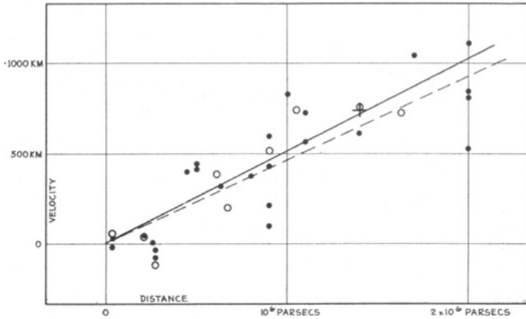
FIG. 9.5. Hubble's first diagram of the velocity–distance relation for galaxies, from his paper of 1929. The horizontal axis is the distance of the galaxy in parsecs ( 1\text{pc} \sim 3 light years) and the vertical axis is the velocity in km/s. The black dots are individual galaxies; the open circles are the same data averaged into nine groups. Hubble gave two solutions—the two lines—one for each set of data, viz 465 \pm 50 and 513 \pm 60 km/s per megaparsec (1 megaparsec \sim 3,000,000 light years). The cross is an estimated mean value for twenty-two additional galaxies without measured distances.
