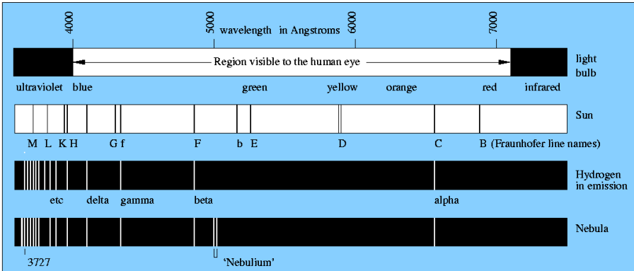
FIG. 5.6. Examples of spectrographic images. A pure hot source, such as a household light bulb, gives a rainbow-like continuous spectrum as in the top panel. The sun's spectrum, next from the top, is crossed by dark lines, caused by cool absorbing gases high in its atmosphere. Its most important lines were found and named by Fraunhofer. The third spectrum shows the lines of hot hydrogen gas. The last spectrum is that of a typical nebula, showing hydrogen as well as the mysterious 'nebulium' lines to the right of H-beta and the 3727 Å line. A wavelength scale in Ångstrom units is given at the top of the diagram. Blue is on the left and red on the right.
