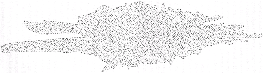
FIG. 4.4. Cross-section of the Milky Way according to Herschel (1785). The position of the solar system is given by the asterisk near the middle. The distances to the borders in each direction are estimated from star counts, assuming that all stars are equally luminous. The fork on the left side is the apparent rift in Sagittarius.
