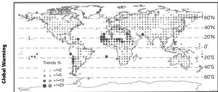
15. Changes in precipitation over land a) 1955–1974 to 1975–1994 and b) 1900 to 1994
