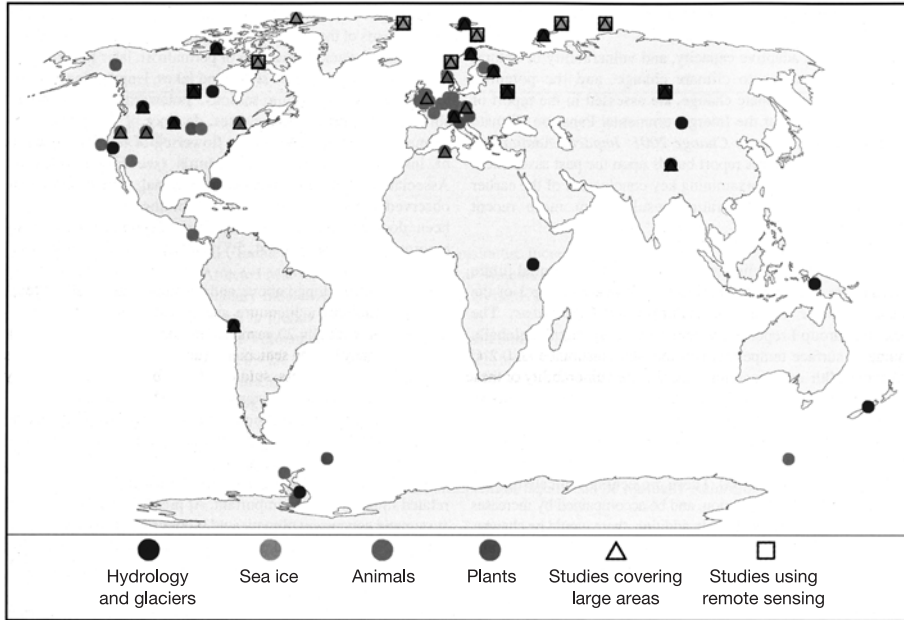
21. Locations at which systematic long-term studies meet stringent criteria documenting recent temperature-related regional climate change impacts on physical and biological systems
