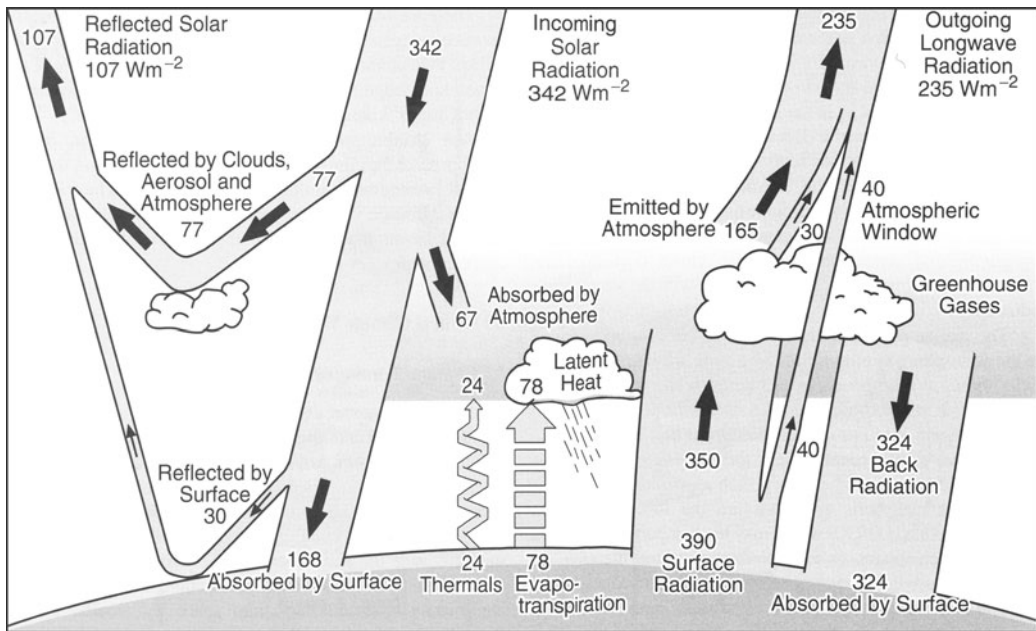
1. The Earth's annual global mean energy balance
