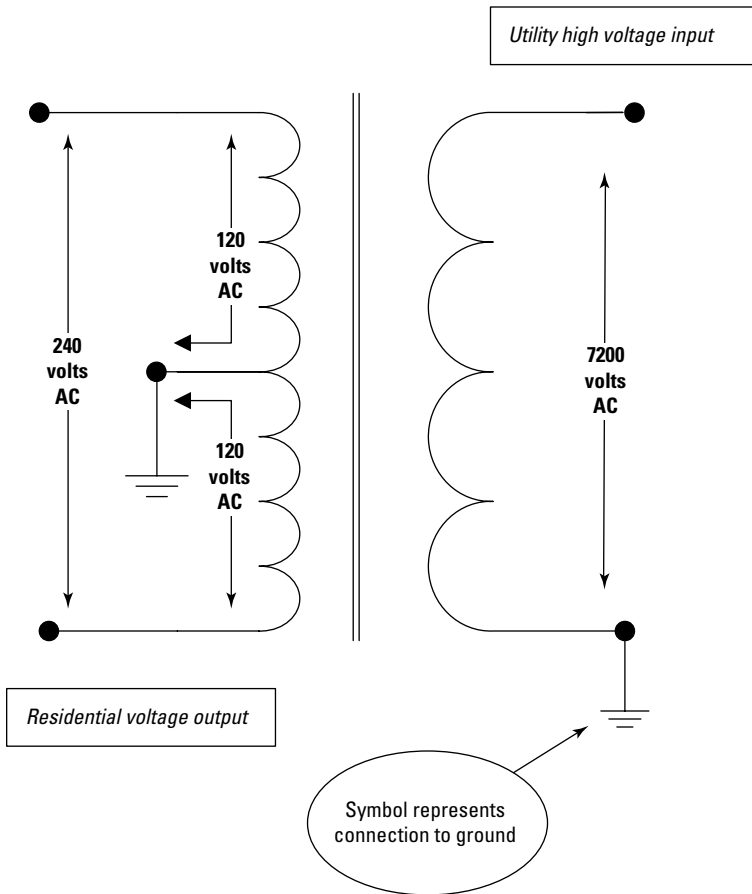
Figure 2-7: Transformers like this feed most residences in the United States.
