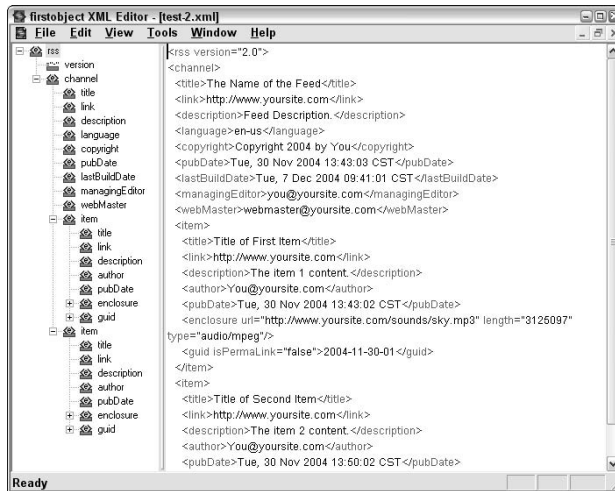
Figure 7-5: You can use an XML editor, such as firstobject XML Editor, to create your RSS feeds.
