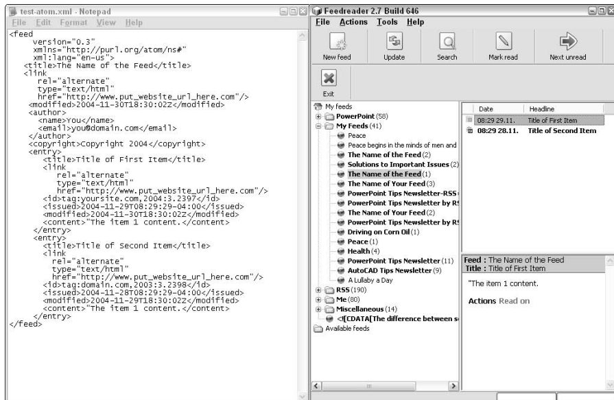
Figure 7-4: An Atom feed in Feedreader.
