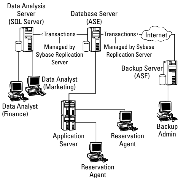
Figure 3-3: Evergreen's dedicated server for marketing and financial analysts.
