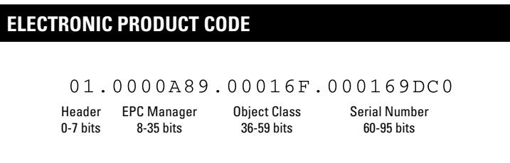
Figure 2-3: The EPC data structure.
