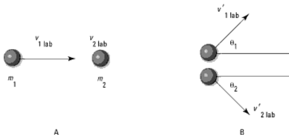
Figure 12-2: Scattering in the lab frame.
