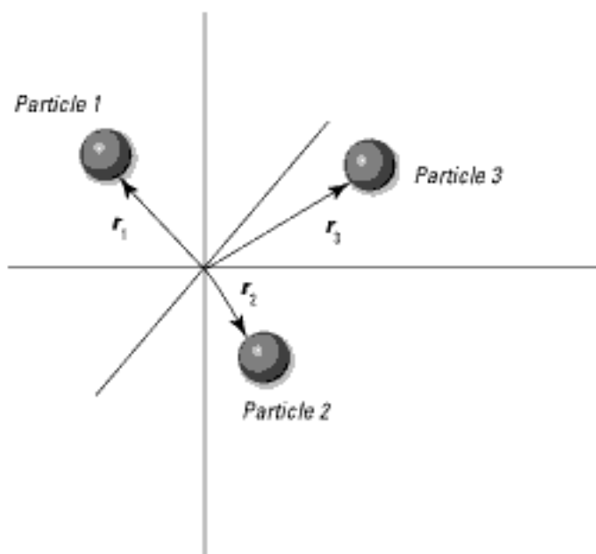
Figure 10-1: A multi- particle system.
