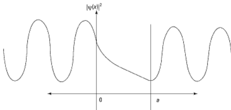
Figure 3-11: |\psi(x)|^2 for a potential barrier E < V_0
