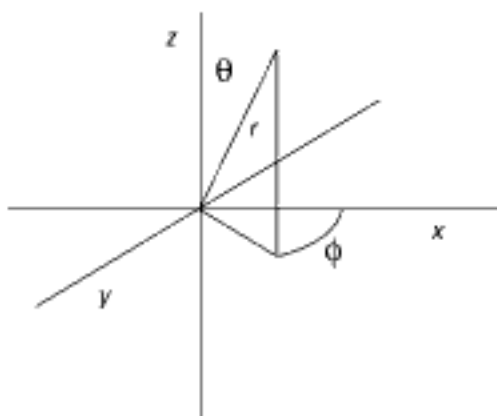
Figure 5-4: The spherical coordinate system.
