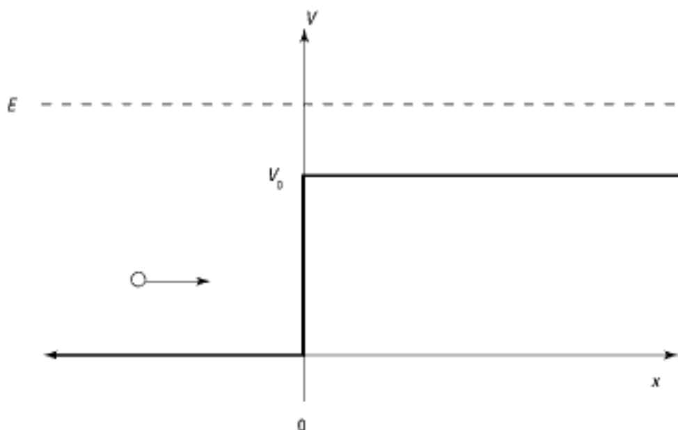
Figure 3-4: A potential step, E > V_0 .
