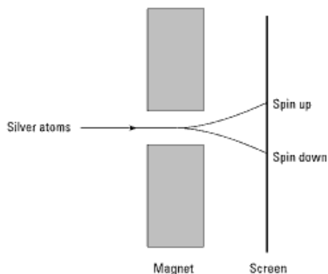
Figure 6-1: The Stern- Gerlach experiment.
