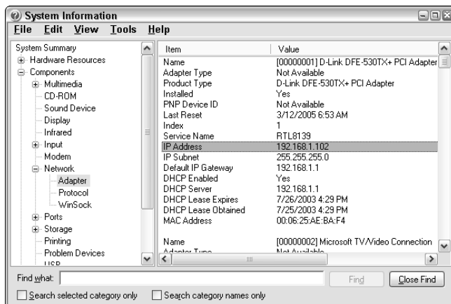
Figure 2-3: Using the System Information command to display network information.
