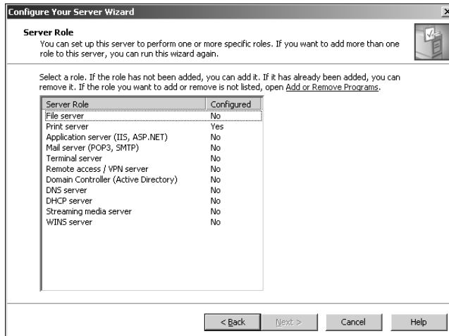
Figure 5-2: The Server Role page.
