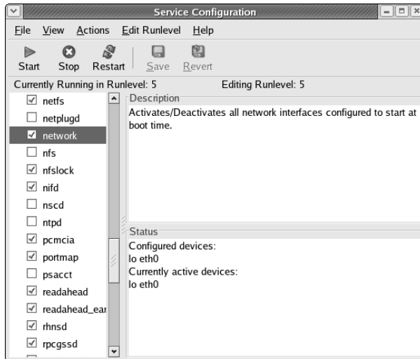
Figure 3-4: The Service Configu- ration window.
