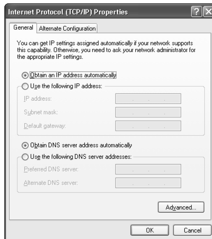
Figure 4-5: Configuring a Windows client to obtain its DNS address from DHCP.
