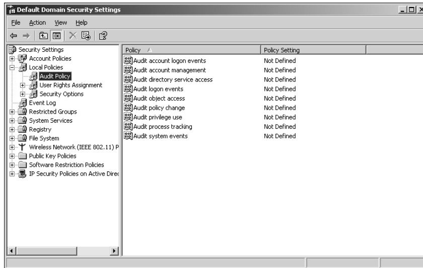
Figure 6-6: Setting the security audit policies.
