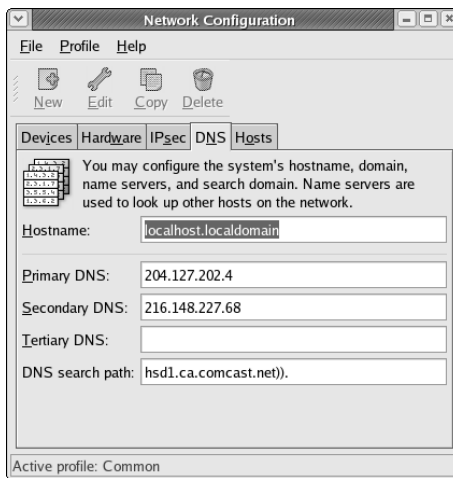
Figure 3-3: Configuring the DNS.
