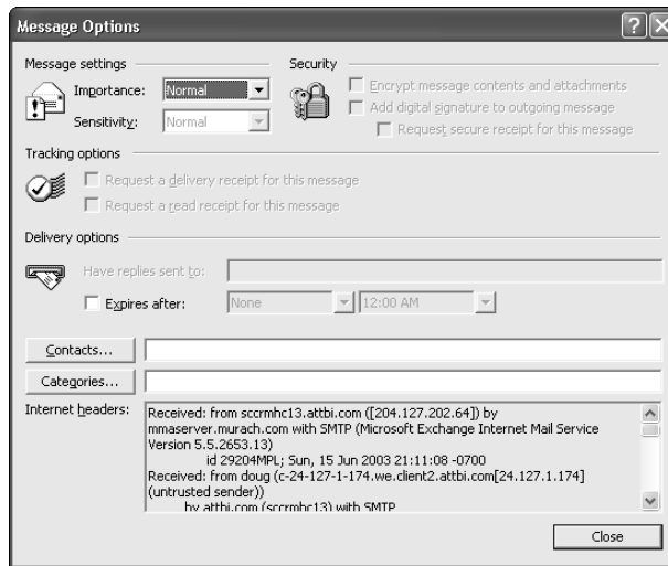
Figure 5-3: Viewing message headers in Outlook.
