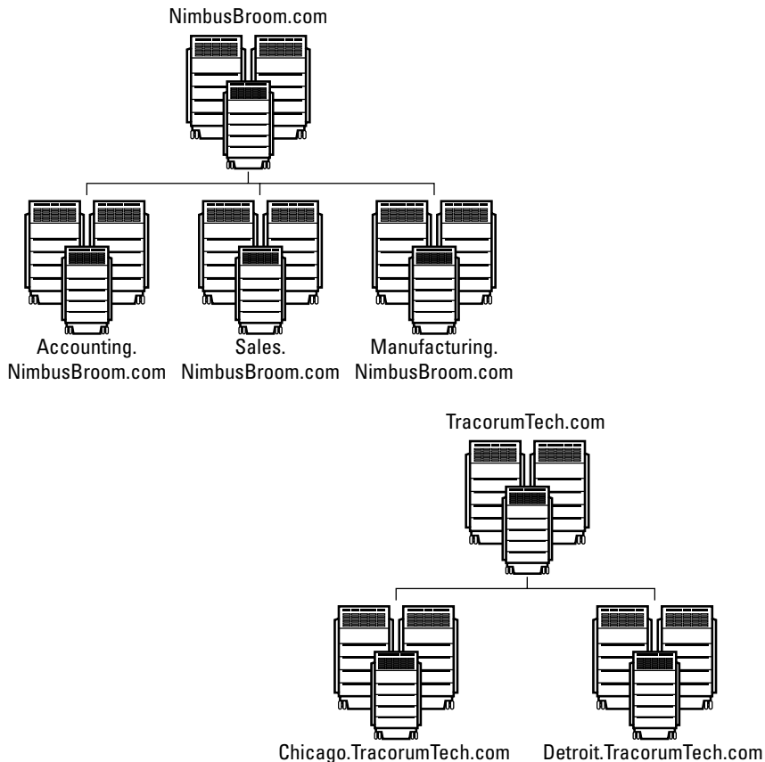
Figure 3-3: A forest with two trees.
