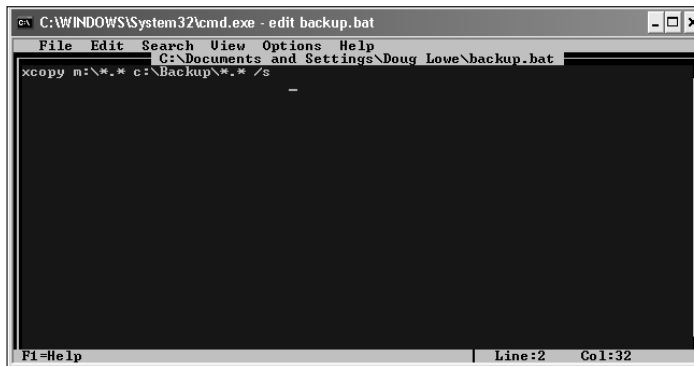
Figure 9-2: Using the Edit command to create a batch file.
