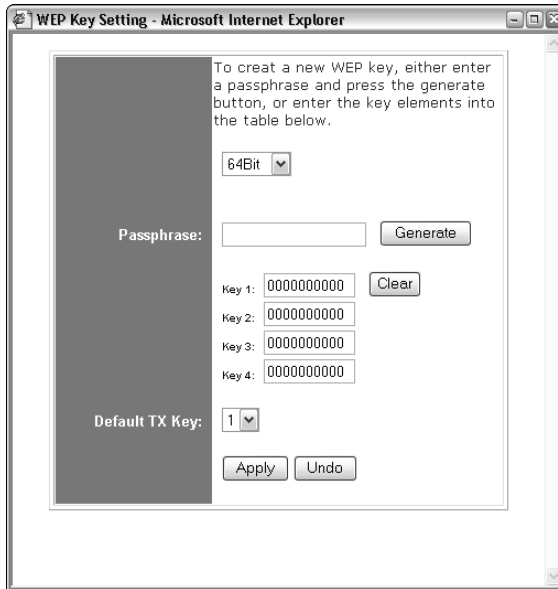
Figure 2-2: Changing WEP settings on a Linksys wireless access point.
