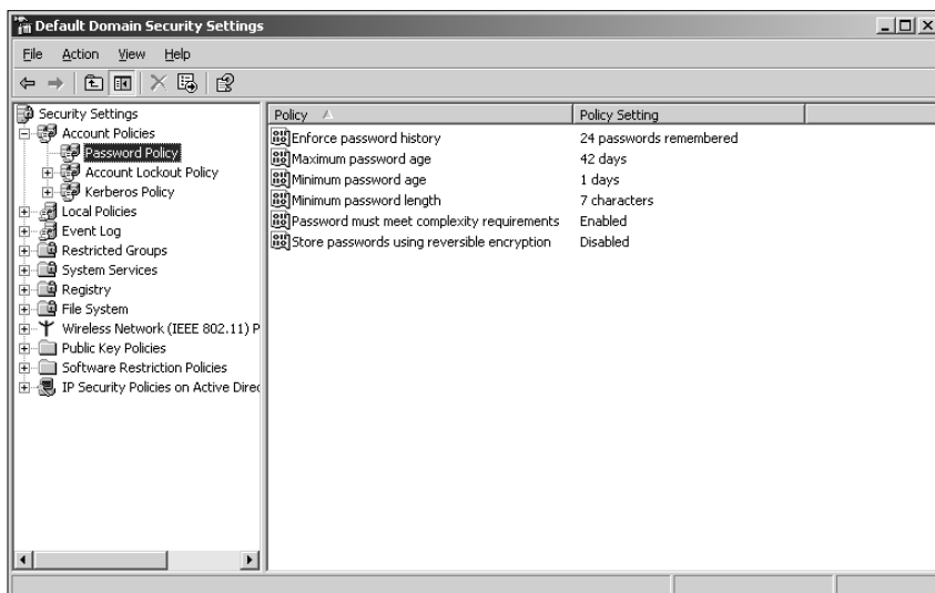
Figure 6-1: Editing the password policies.
