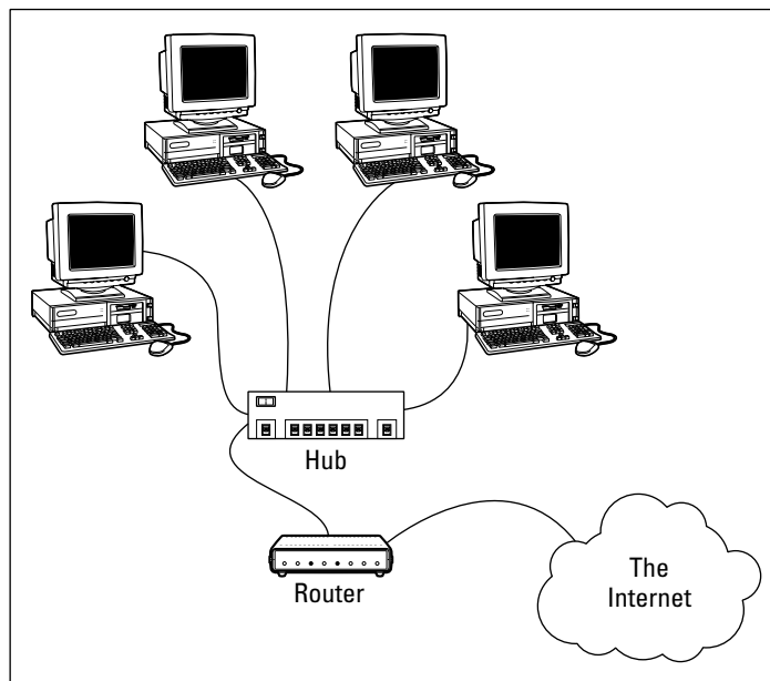
Figure 3-5: Using a router.
