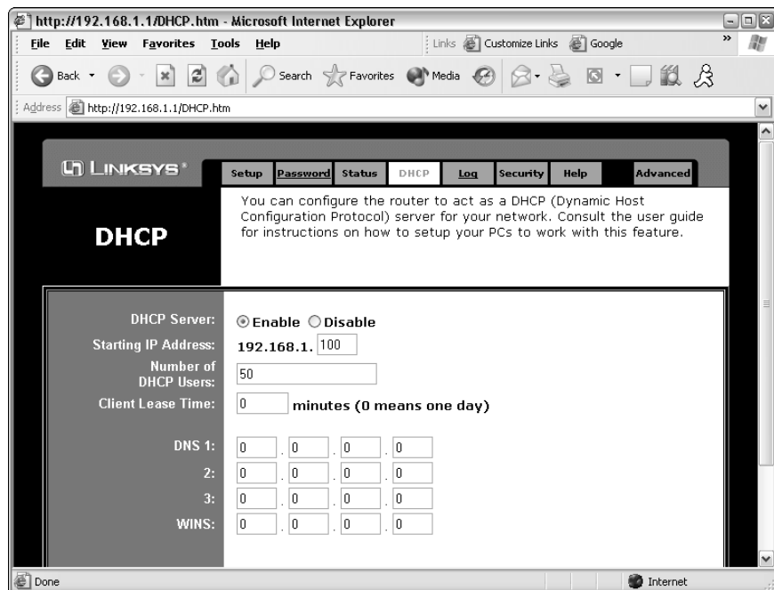
Figure 1-7: Configuring DHCP for a Linksys wireless access point router.
