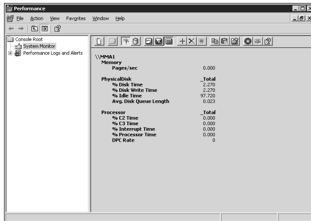
Figure 8-7: Performance Monitor in Report mode.
