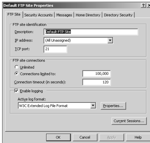
Figure 5-2: The FTP Site Properties dialog box.
