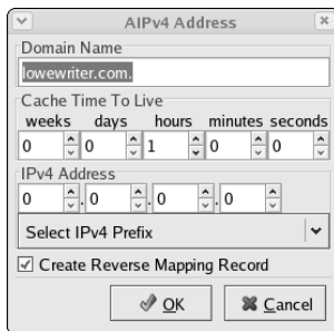
Figure 4-7: Creating an A record.
