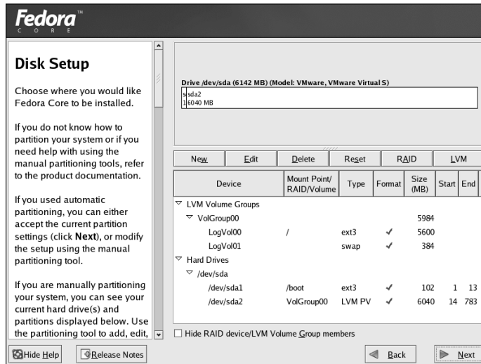
Figure 1-8: The Disk Setup screen.
