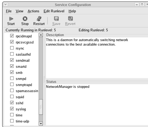
Figure 5-1: Using the Service Configura- tion tool.
