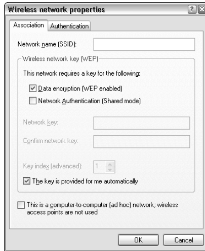
Figure 1-9: Configuring wireless networking in Windows XP.
