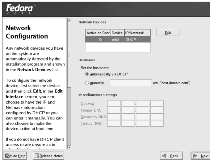
Figure 1-10: The Network Configu- ration screen.
