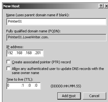
Figure 4-4: The New Host dialog box.
