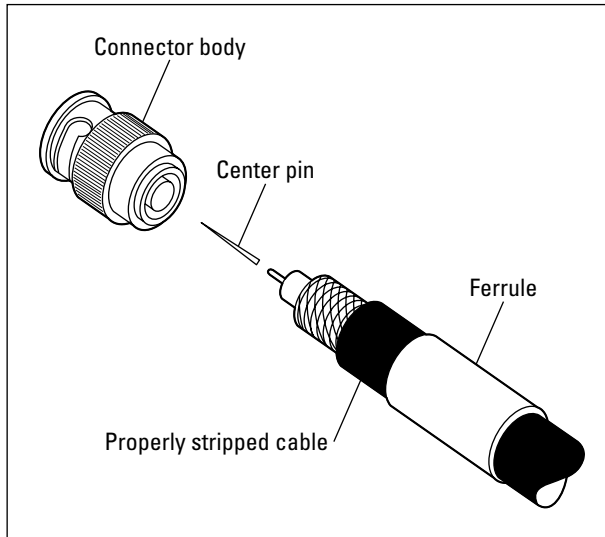
Figure 2-4: Attaching a BNC con- nector to coaxial cable.
