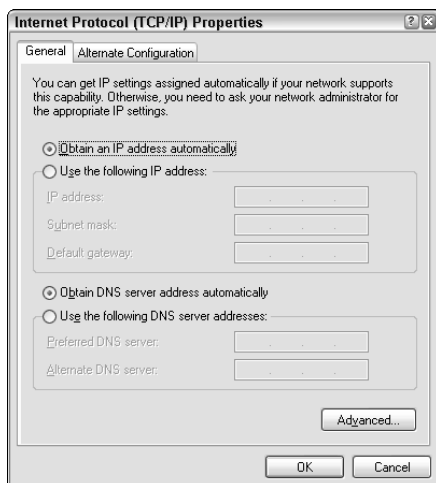
Figure 4-4: Configuring TCP/IP (Windows XP).
