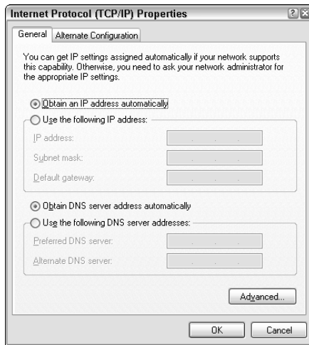
Figure 5-6: Making sure that TCP/IP is configured for DHCP.
