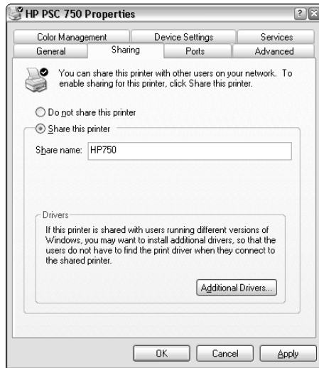
Figure 3-9: The Properties dialog box for a shared printer.
