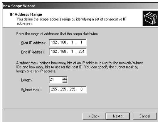
Figure 3-2: Specifying the scope's address range and subnet mask.
