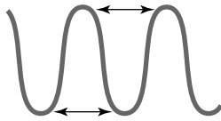
Figure 3-3: Light waves measured in wave- lengths.
