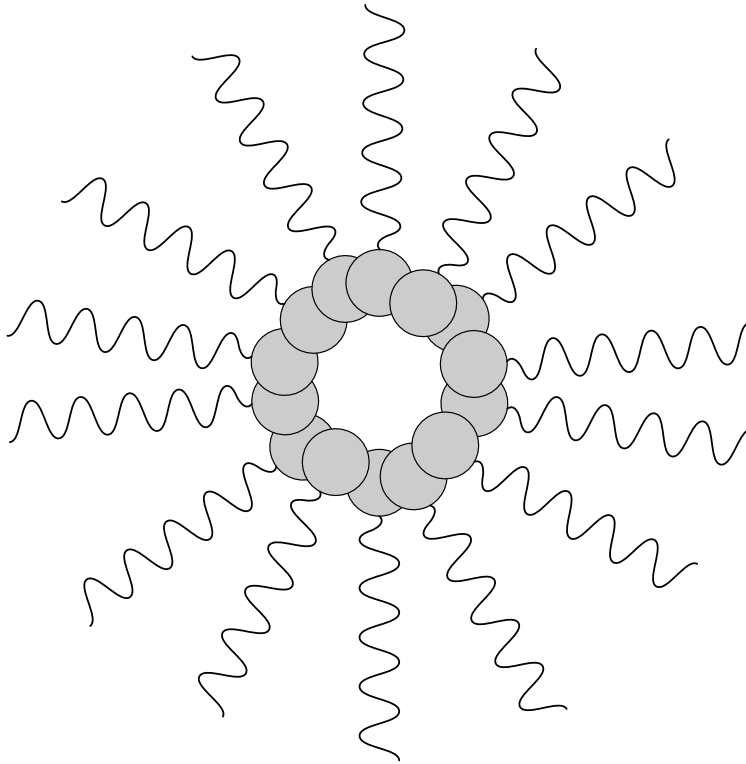
Figure 11-4: A reverse micelle with the hydrophobic heads in the center.
