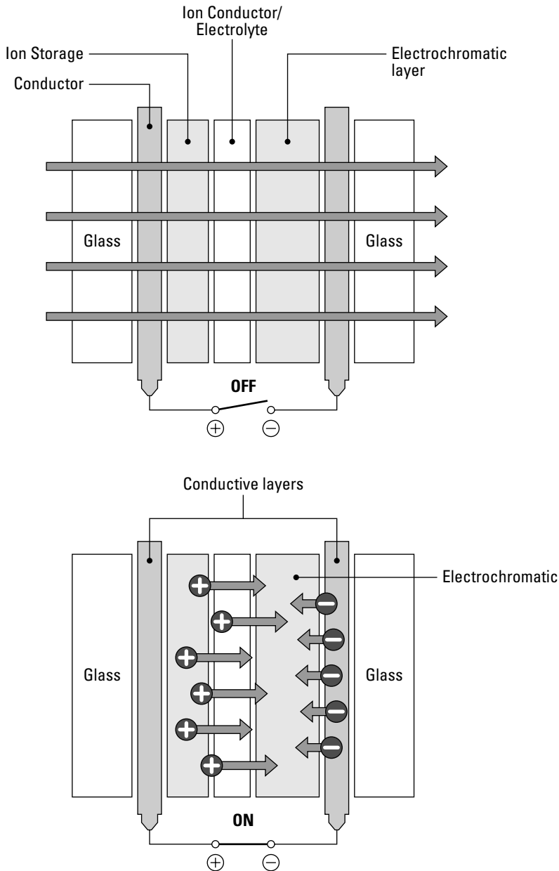
Figure 5-5: Smart windows can change their opacity.
