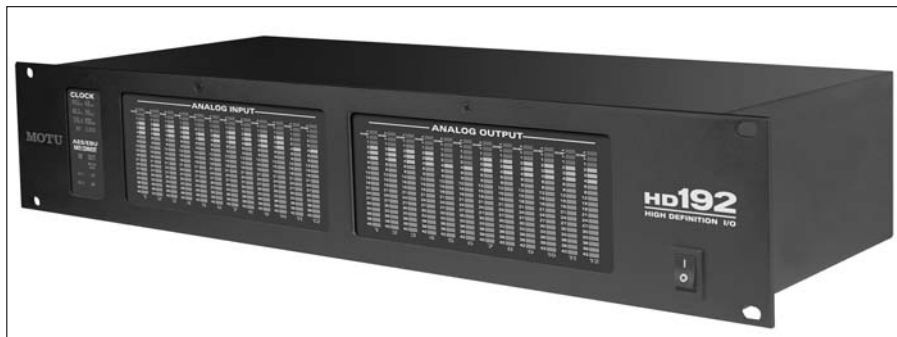
Figure 2-3: A PCI interface with a breakout box for the analog components is the preferred form of PCI interface.
