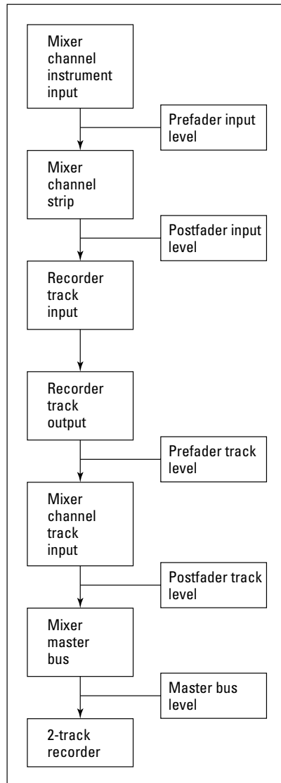
Figure 7-2: Most recording systems allow you to monitor your signal levels at various places in the signal chain.
