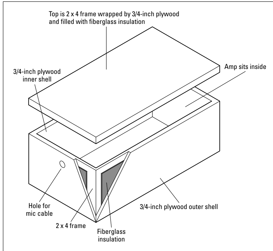
Figure 3-17: An amp-isolator box reduces the amount of noise you hear from your amp, even when it's cranked.
