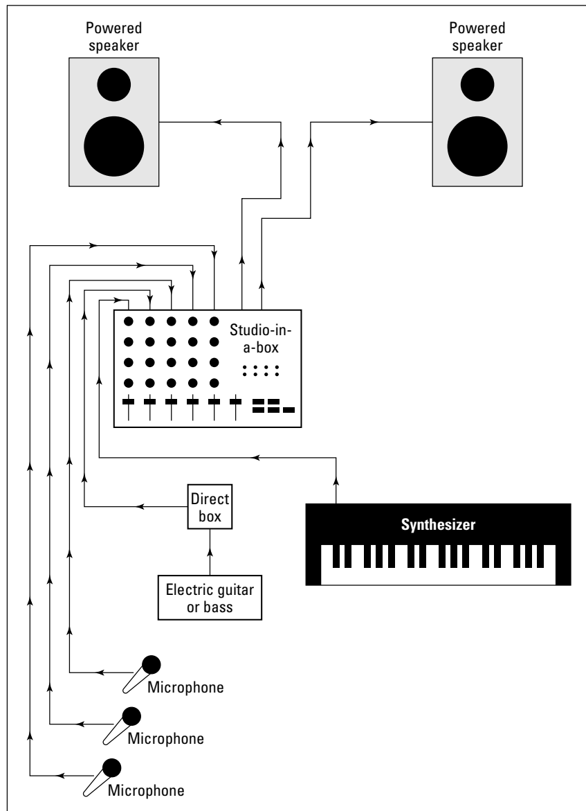
Figure 3-12: The live audio system setup. MIDI devices are rarely used.
