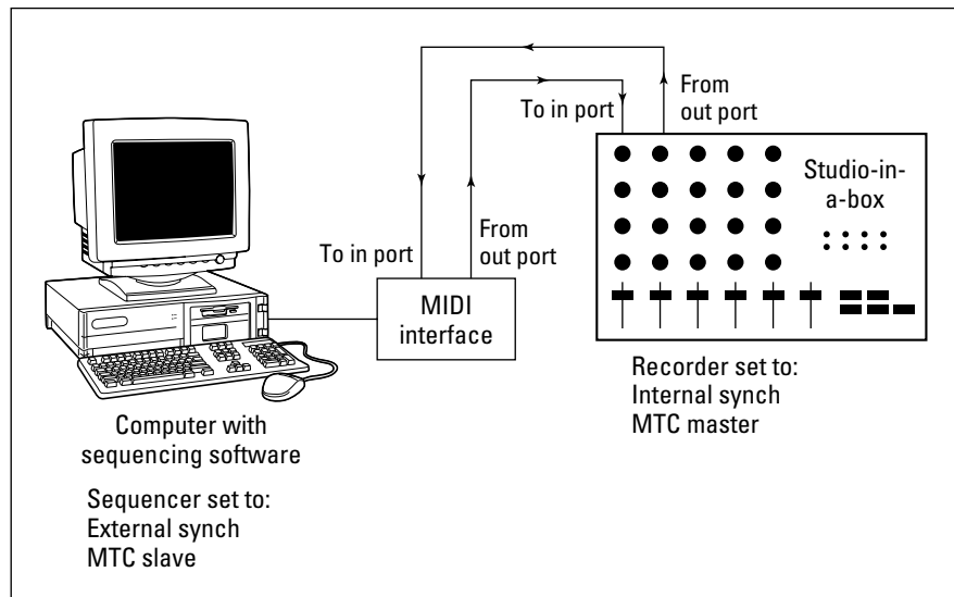
Figure 12-3: A system with a separate sequencer and audio recorder are set up this way.
