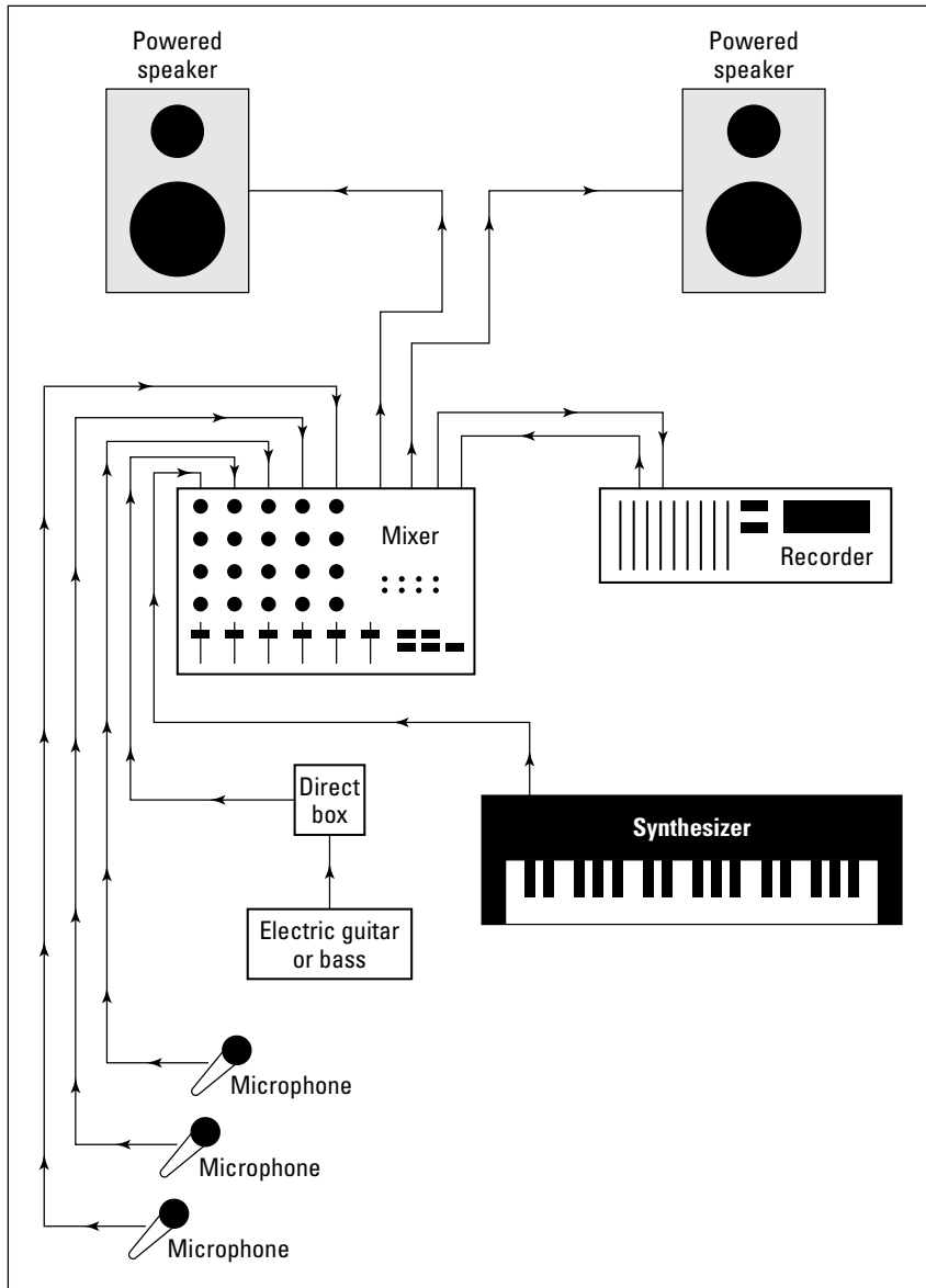
Figure 2-10: A system for live recording.
