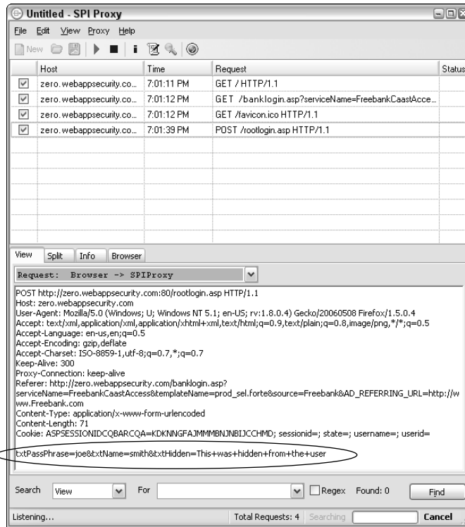
Figure 15-10: Using SPI Proxy to find and manipulate hidden fields.
