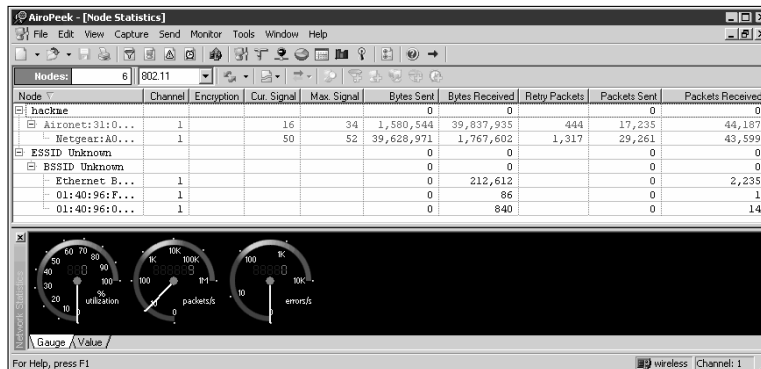
Figure 10-10: Using AiroPeek's Monitor to spot a product that doesn't belong.
