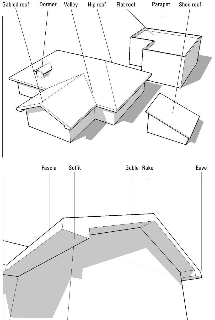
Figure 4-29: Some different kinds of roofs, and their various and sundry parts.
