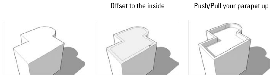
Figure 4-30: Modeling parapets on flat-roofed buildings is easy.
