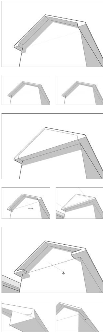
Figure 4-34: Some common gabled roof details and how to make them.
