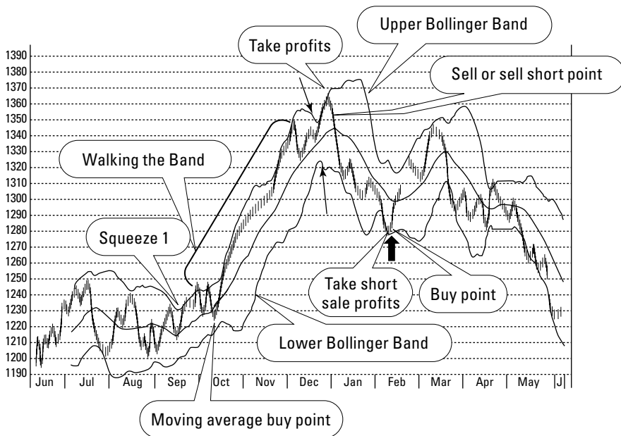
Figure 8-2: Trading the euro currency using Bollinger bands.
