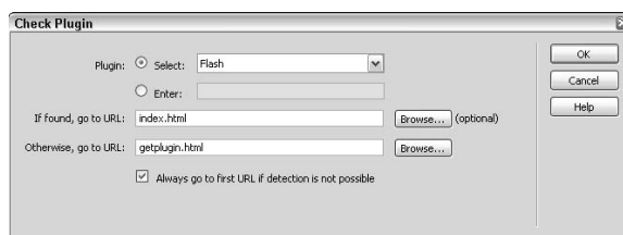
Figure 2-5: The Check Browser behavior can send a visitor to a page you specify.
