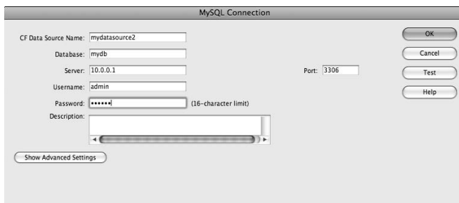
Figure 6-5: Adding a MySQL connection to ColdFusion through Dreamweaver.
